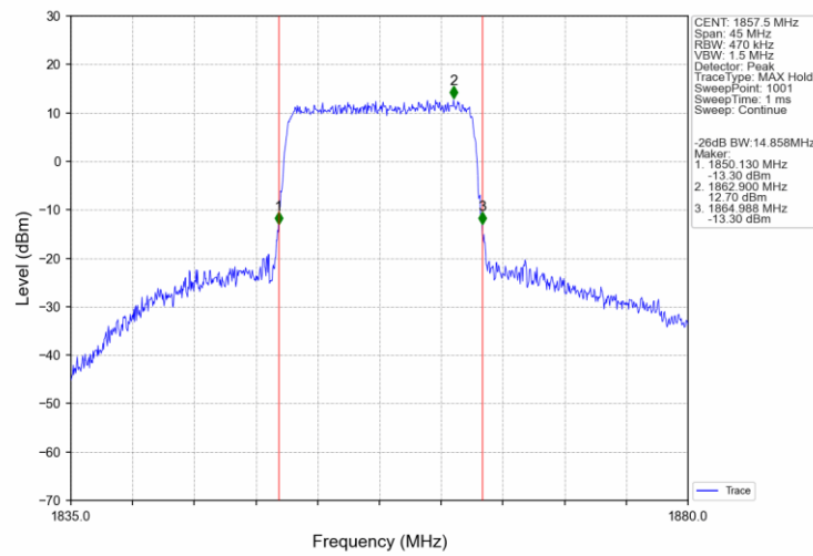
Band2_15MHz_16QAM_LCH_1857.5MHz_RB_75_0_NTNV
