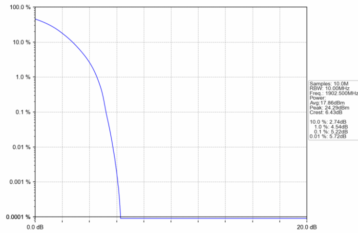
Band2_15MHz_QPSK_HCH_1902.5MHz_RB_75_0_NTNV
