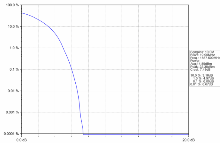
Band2_15MHz_16QAM_LCH_1857.5MHz_RB_75_0_NTNV
