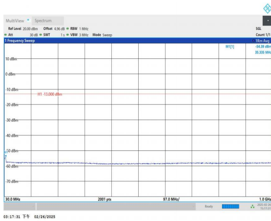
Band66_20MHz_16QAM_132322_1RB#0_30~1000_30~1000
