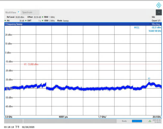
Band66_20MHz_16QAM_132572_1RB#0_3000~20000_3000~20000
