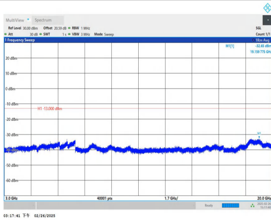
Band66_20MHz_16QAM_132322_1RB#0_3000~20000_3000~20000
