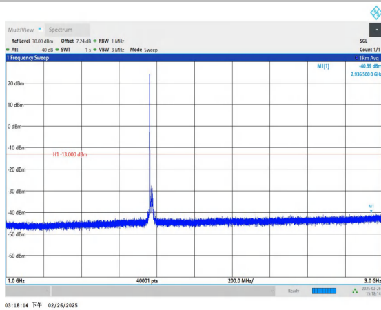
Band66_20MHz_16QAM_132572_1RB#0_1000~3000_1000~3000
