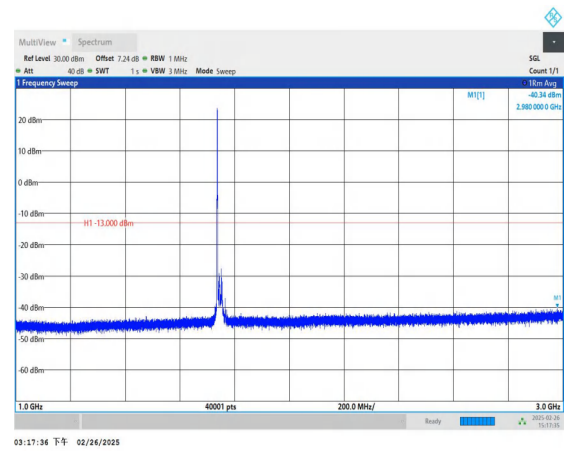
Band66_20MHz_16QAM_132322_1RB#0_1000~3000_1000~3000
