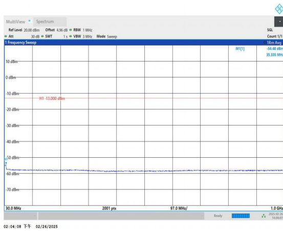
Band66_1.4MHz_16QAM_132322_1RB#0_30~1000_30~1000
