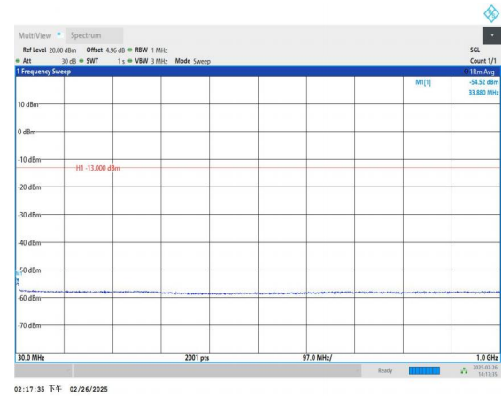
Band66_3MHz_16QAM_131987_1RB#0_30~1000_30~1000
