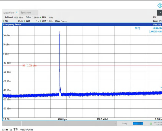
Band66_10MHz_16QAM_132022_1RB#0_1000~3000_1000~3 000
