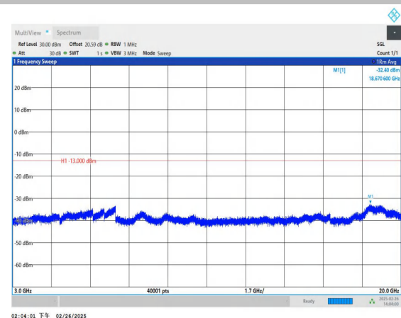
Band66_1.4MHz_QPSK_132322_1RB#0_3000~20000_3000~20000
