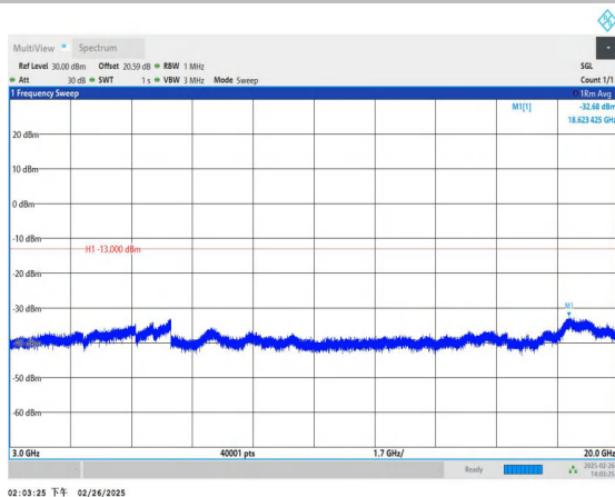
Band66_1.4MHz_QPSK_131979_1RB#0_3000~20000_3000~20000
