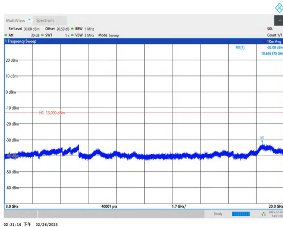
Band66_5MHz_QPSK_131997_1RB#0_3000~20000_3000~2000
