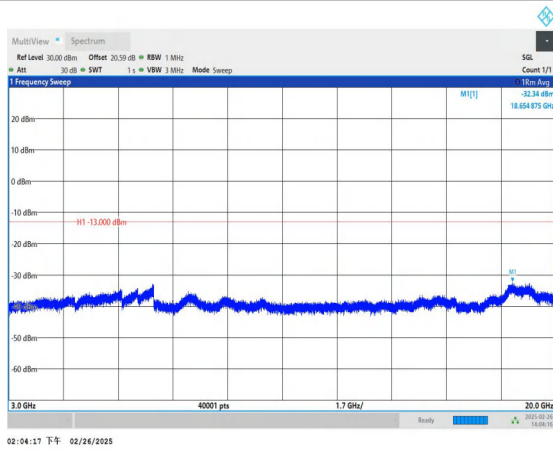
Band66_1.4MHz_16QAM_132322_1RB#0_3000~20000_3000~20000
