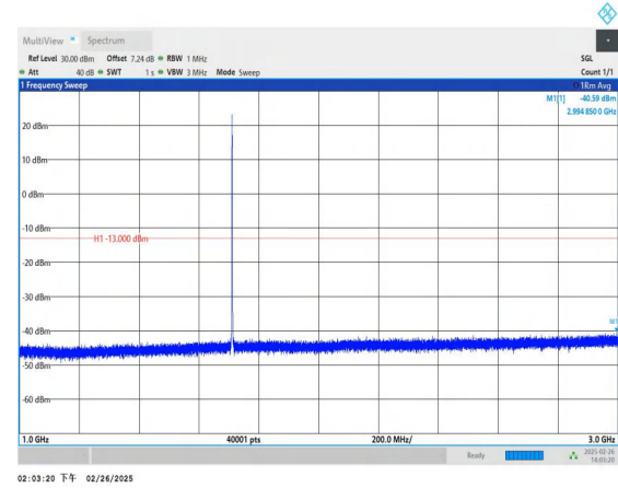
Band66_1.4MHz_QPSK_131979_1RB#0_1000~3000_1000~3000
