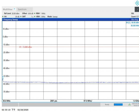
Band66_1.4MHz_QPSK_131979_1RB#0_30~1000_30~1000
