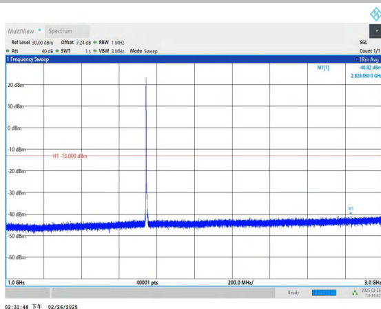
Band66_5MHz_QPSK_132322_1RB#0_1000~3000_1000~3000
