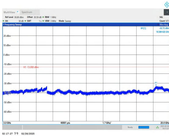
Band66_3MHz_QPSK_131987_1RB#0_3000~20000_3000~2000
