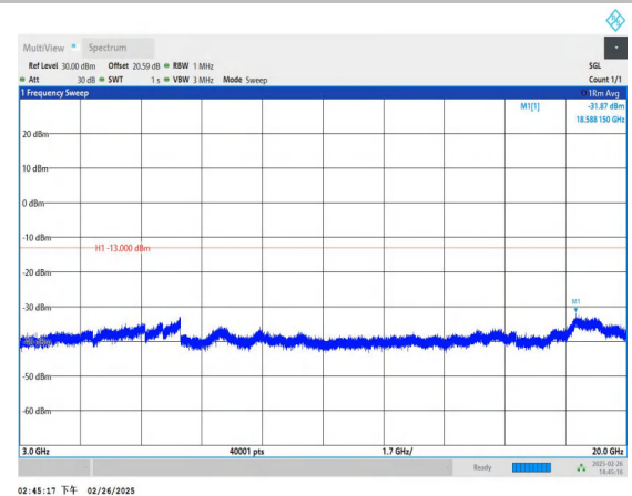
Band66_10MHz_16QAM_132022_1RB#0_3000~20000_3000~ 20000
