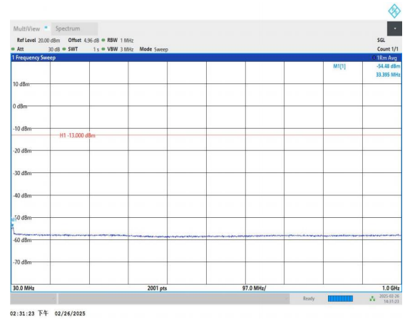
Band66_5MHz_16QAM_131997_1RB#0_30~1000_30~1000
