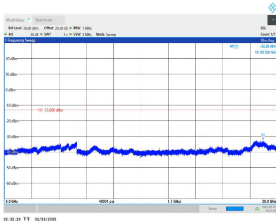
Band66_5MHz_QPSK_132647_1RB#0_3000~20000_3000~20000
