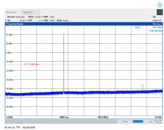
Band66_1.4MHz_16QAM_132322_1RB#0_1000~3000_1000~3000
