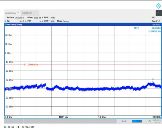
Band66_5MHz_QPSK_132322_1RB#0_3000~20000_3000~2000
