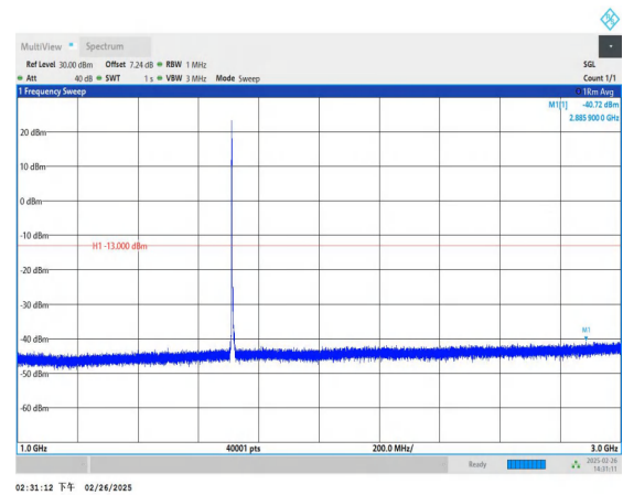
Band66_5MHz_QPSK_131997_1RB#0_1000~3000_1000~3000
