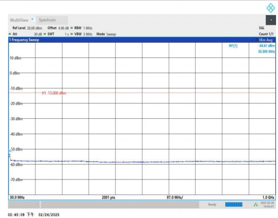
Band66_10MHz_16QAM_132022_1RB#0_30~1000_30~1000
