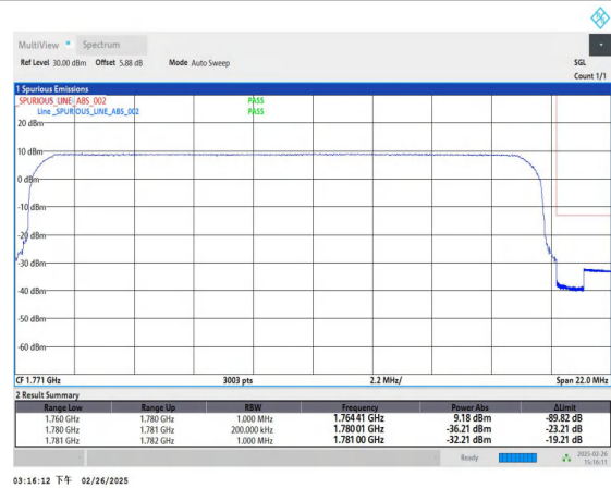
Band66_20MHz_QPSK_132572_100RB#0
