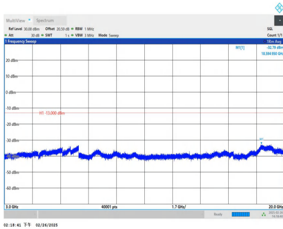
Band66_3MHz_QPSK_132657_1RB#0_3000~20000_3000~20000
