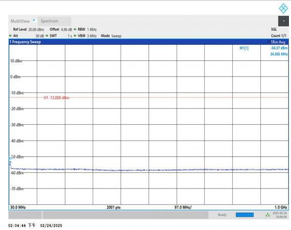
Band66_1.4MHz_16QAM_132665_1RB#0_30~1000_30~1000
