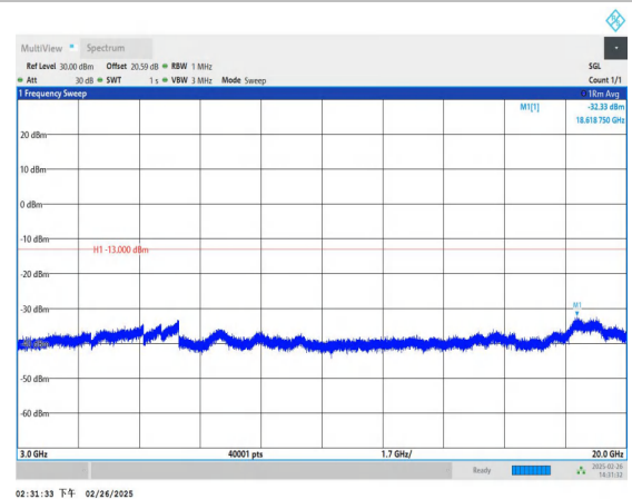
Band66_5MHz_16QAM_131997_1RB#0_3000~20000_3000~20000
