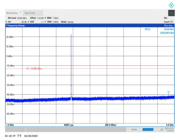
Band66_3MHz_QPSK_132657_1RB#0_1000~3000_1000~3000
