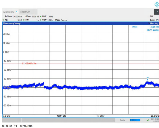
Band66_1.4MHz_QPSK_132665_1RB#0_3000~20000_3000~20000
