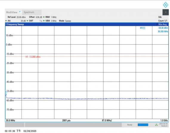
Band66_1.4MHz_16QAM_131979_1RB#0_30~1000_30~1000
