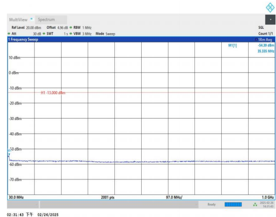
Band66_5MHz_QPSK_132322_1RB#0_30~1000_30~1000
