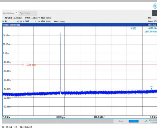
Band66_1.4MHz_QPSK_132322_1RB#0_1000~3000_1000~3000
