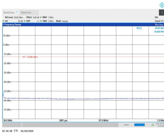
Band66_1.4MHz_QPSK_132665_1RB#0_30~1000_30~1000
