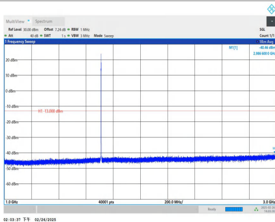
Band66_1.4MHz_16QAM_131979_1RB#0_1000~3000_1000~3000
