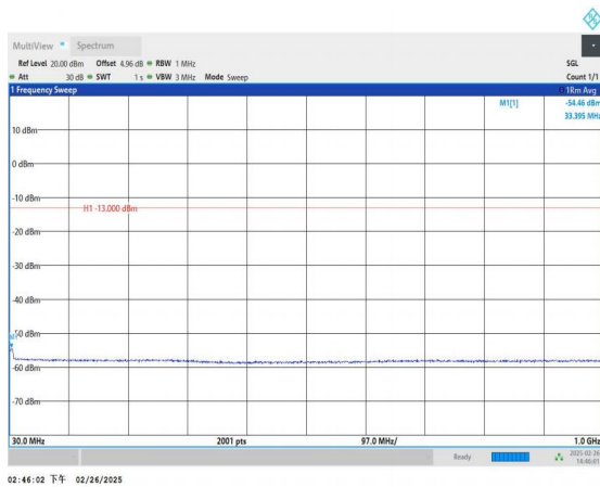
Band66_10MHz_QPSK_132622_1RB#0_30~1000_30~1000
