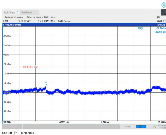
Band66_10MHz_QPSK_132622_1RB#0_3000~20000_3000~20 000
