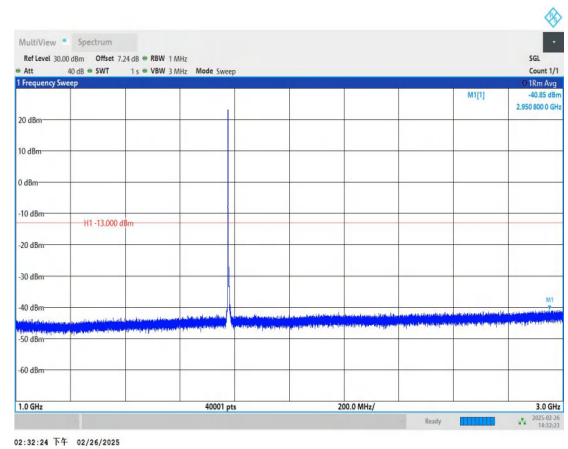
Band66_5MHz_QPSK_132647_1RB#0_1000~3000_1000~3000
