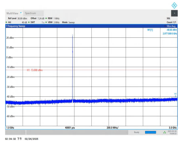
Band66_1.4MHz_QPSK_132665_1RB#0_1000~3000_1000~3000
