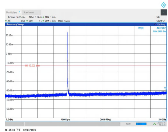
Band66_10MHz_QPSK_132622_1RB#0_1000~3000_1000~300 0
