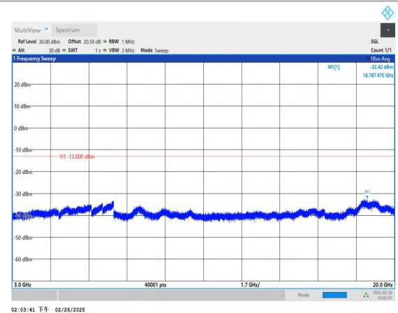
Band66_1.4MHz_16QAM_131979_1RB#0_3000~20000_3000~20000
