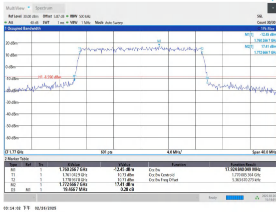
Band66-20MHz-QPSK-132572-100RB#0-PASS
