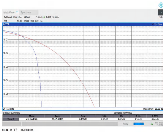
Band66-20MHz-16QAM-132072-1RB#0-PASS
