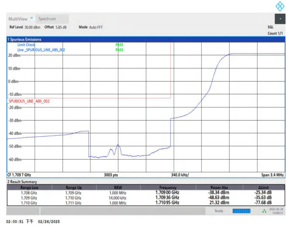
Band66_1.4MHz_QPSK_131979_1RB#5
