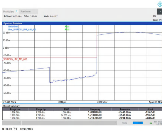
Band66_1.4MHz_QPSK_131979_6RB#0
