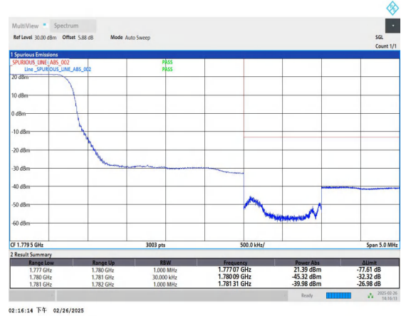
Band66_3MHz_QPSK_132657_1RB#0
