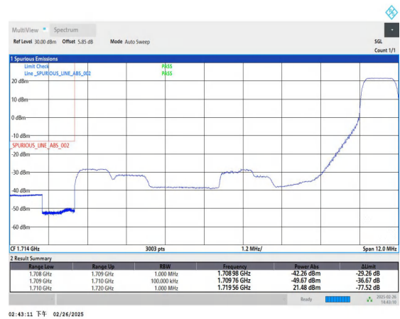
Band66_10MHz_QPSK_132022_1RB#49
