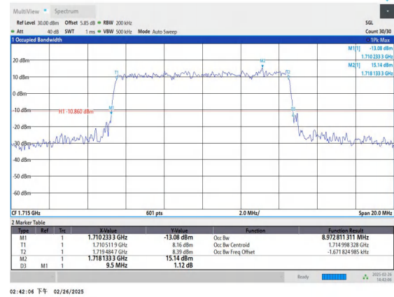
Band66-10MHz-16QAM-132022-50RB#0-PASS
