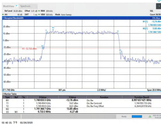
Band66-10MHz-16QAM-132322-50RB#0-PASS
