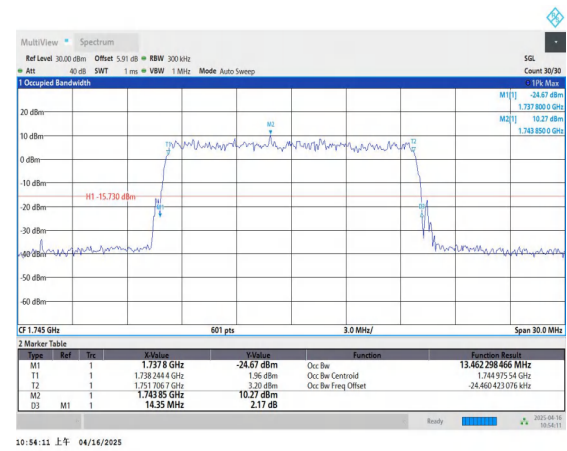
Band66-15MHz-QPSK-132322-75RB#0-PASS
