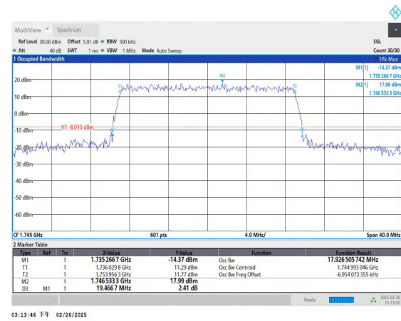
Band66-20MHz-QPSK-132322-100RB#0-PASS
