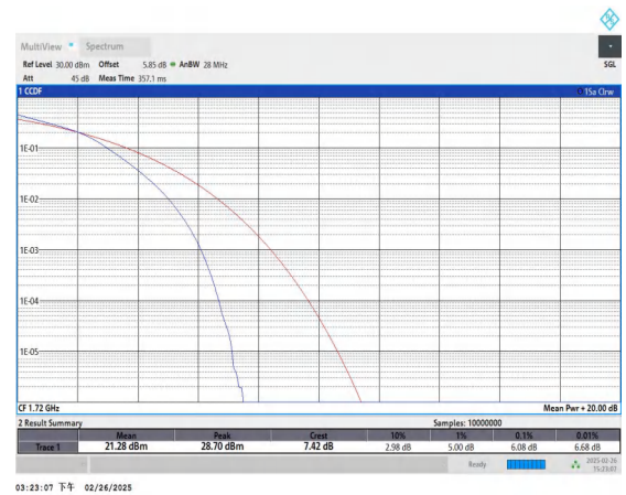
Band66-20MHz-16QAM-132072-100RB#0-PASS
