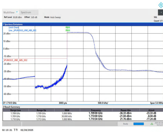
Band66_3MHz_16QAM_131987_1RB#0
