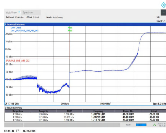
Band66_3MHz_16QAM_131987_1RB#14
