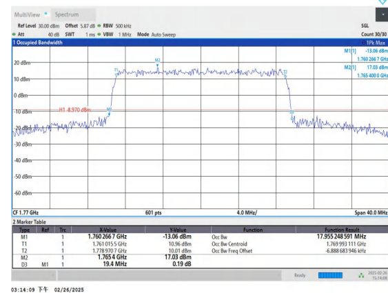
Band66-20MHz-16QAM-132572-100RB#0-PASS
