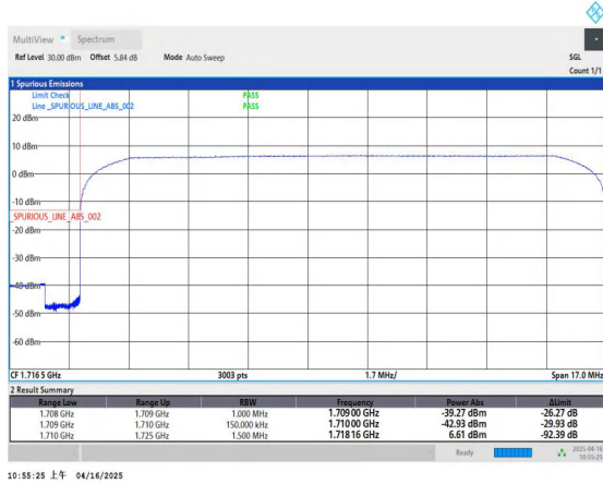
Band66_15MHz_QPSK_132047_75RB#0
