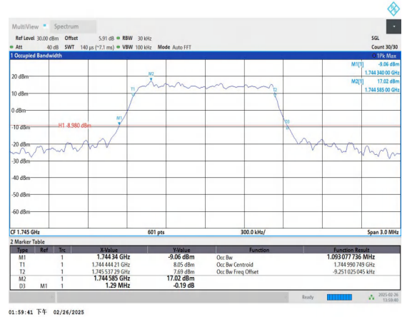
Band66-1.4MHz-QPSK-132322-6RB#0-PASS
