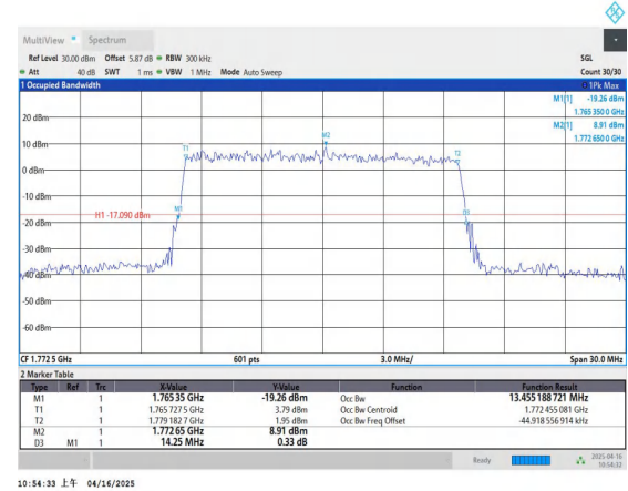
Band66-15MHz-16QAM-132597-75RB#0-PASS
