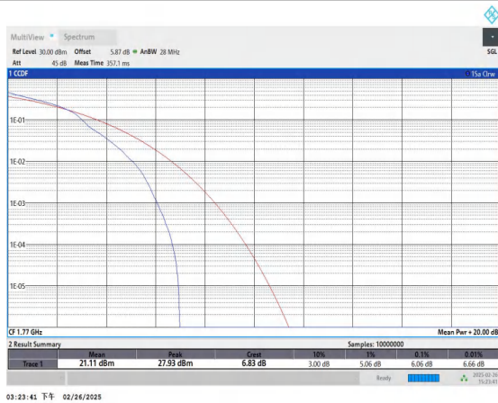
Band66-20MHz-16QAM-132572-1RB#0-PASS
