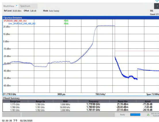
Band66_5MHz_16QAM_132647_1RB#24
