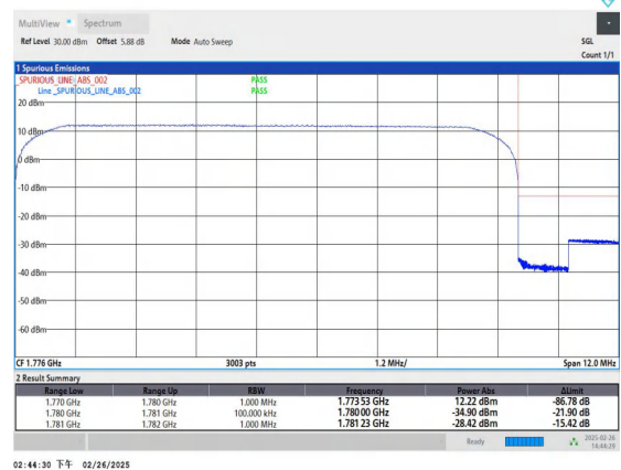
Band66_10MHz_QPSK_132622_50RB#0
