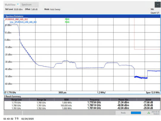
Band66_10MHz_QPSK_132622_1RB#0
