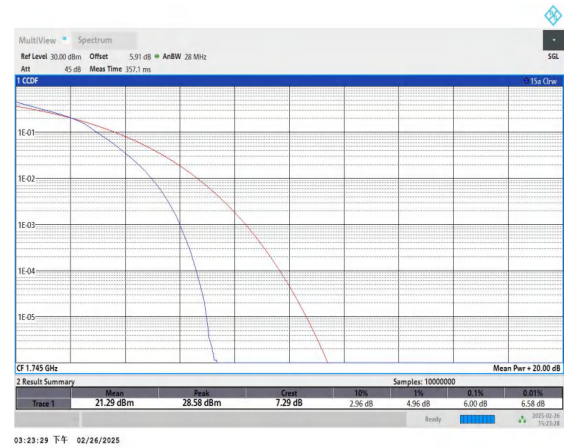
Band66-20MHz-16QAM-132322-100RB#0-PASS
