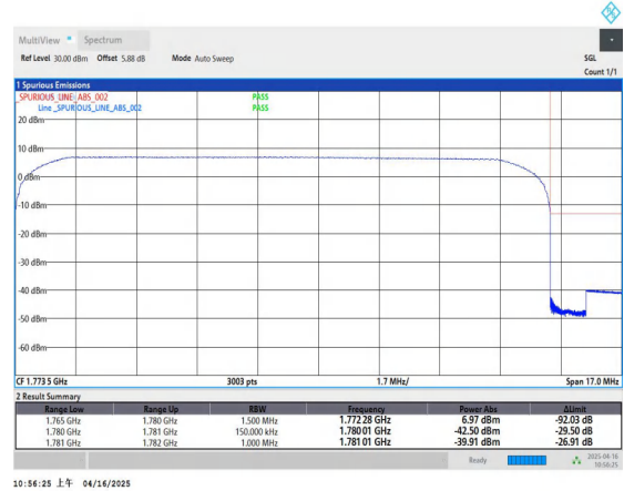
Band66_15MHz_QPSK_132597_75RB#0
