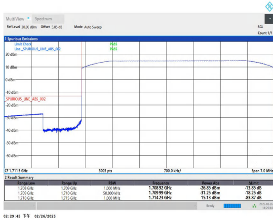
Band66_5MHz_QPSK_131997_25RB#0
