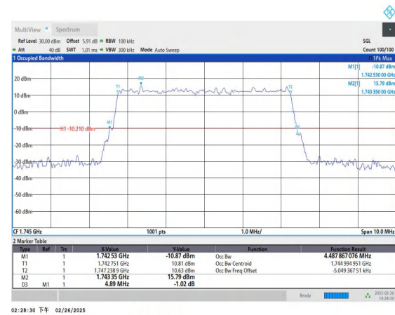
Band66-5MHz-QPSK-132322-25RB#0-PASS
