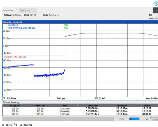
Band66_3MHz_QPSK_131987_15RB#0
