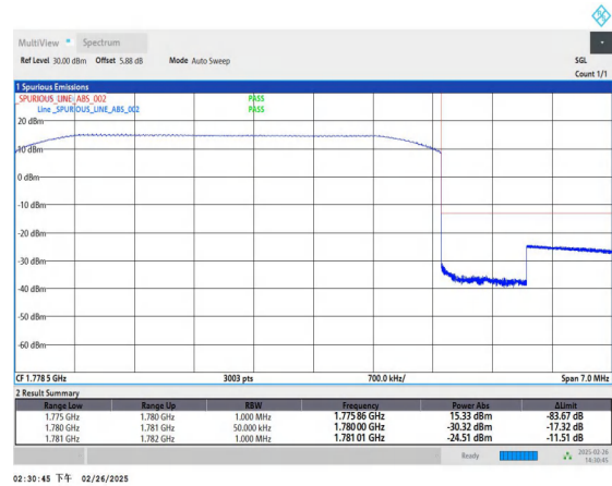
Band66_5MHz_QPSK_132647_25RB#0
