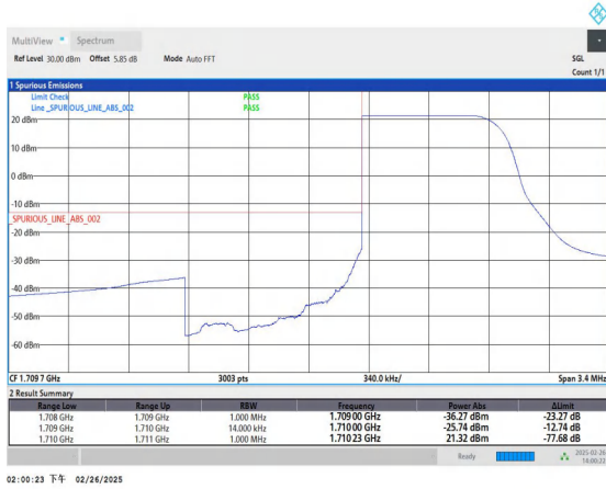
Band66_1.4MHz_QPSK_131979_1RB#0
