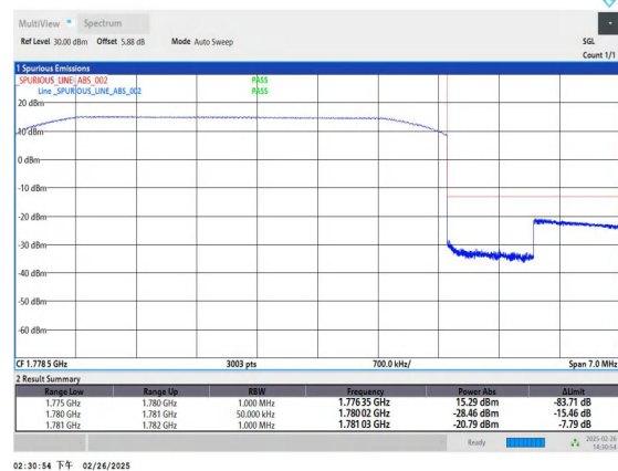
Band66_5MHz_16QAM_132647_25RB#0
