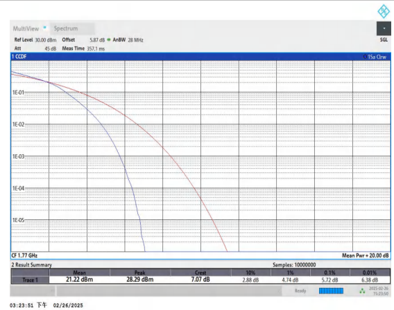
Band66-20MHz-16QAM-132572-100RB#0-PASS
