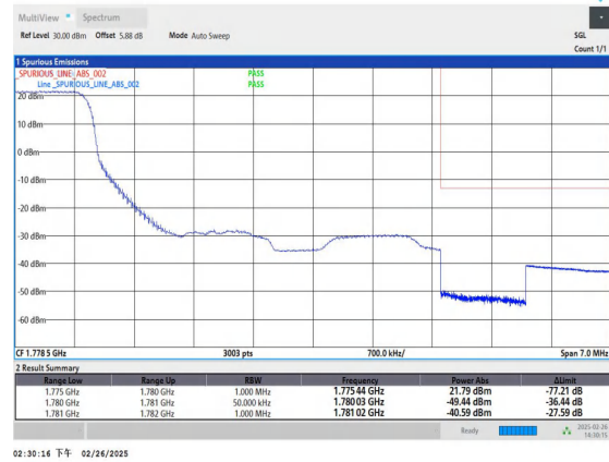
Band66_5MHz_16QAM_132647_1RB#0
