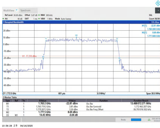
Band66-15MHz-QPSK-132597-75RB#0-PASS
