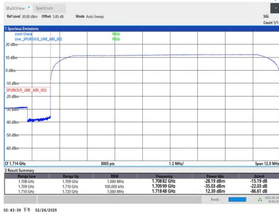
Band66_10MHz_16QAM_132022_50RB#0
