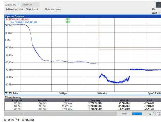
Band66_3MHz_16QAM_132657_1RB#0
