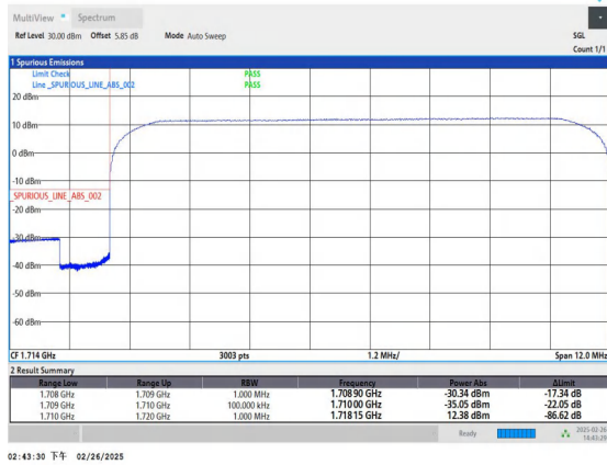
Band66_10MHz_QPSK_132022_50RB#0
