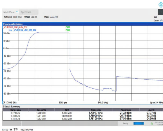
Band66_1.4MHz_16QAM_132665_1RB#5
