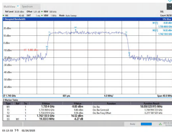
Band66-20MHz-16QAM-132322-100RB#0-PASS
