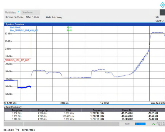
Band66_10MHz_16QAM_132022_1RB#49
