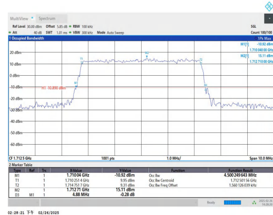
Band66-5MHz-16QAM-131997-25RB#0-PASS
