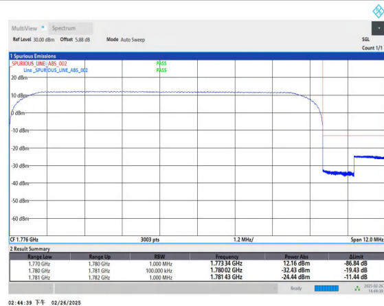
Band66_10MHz_16QAM_132622_50RB#0
