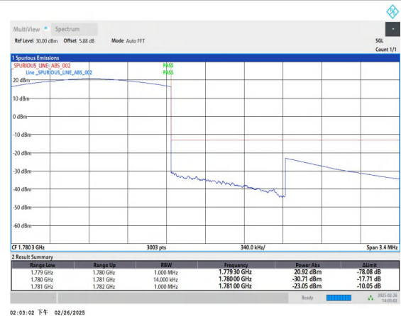
Band66_1.4MHz_16QAM_132665_6RB#0
