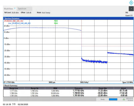
Band66_3MHz_QPSK_132657_15RB#0
