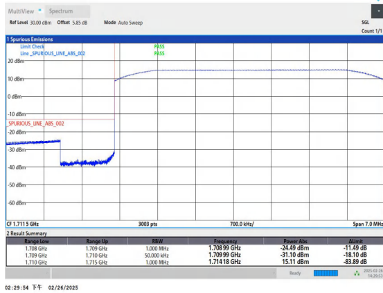
Band66_5MHz_16QAM_131997_25RB#0
