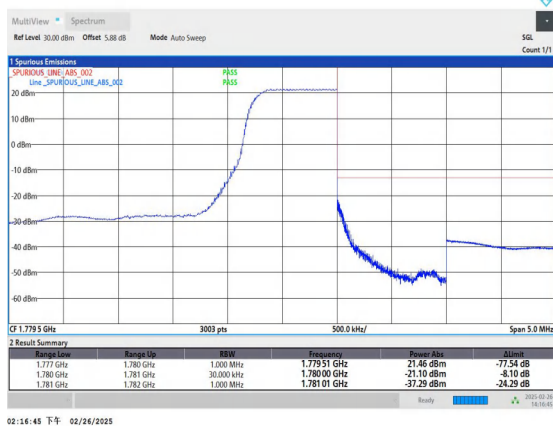
Band66_3MHz_16QAM_132657_1RB#14
