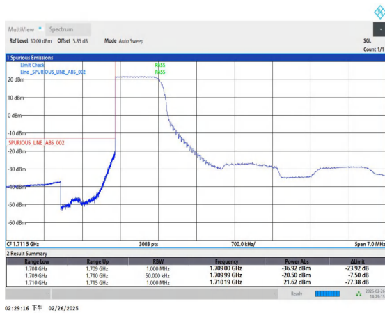
Band66_5MHz_16QAM_131997_1RB#0
