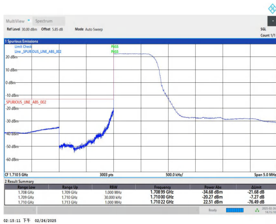
Band66_3MHz_QPSK_131987_1RB#0
