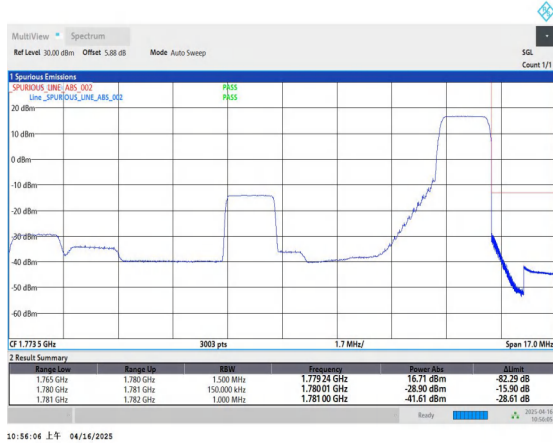
Band66_15MHz_QPSK_132597_1RB#74
