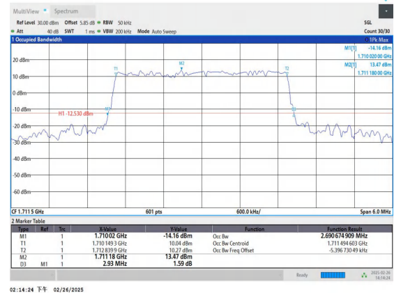
Band66-3MHz-16QAM-131987-15RB#0-PASS
