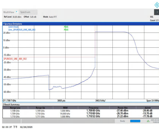
Band66_1.4MHz_16QAM_131979_1RB#0
