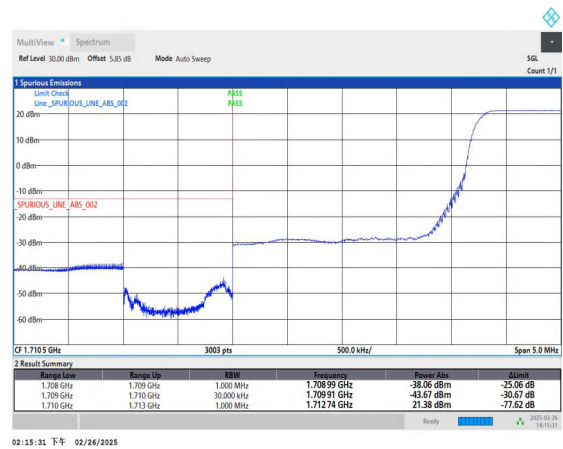
Band66_3MHz_QPSK_131987_1RB#14
