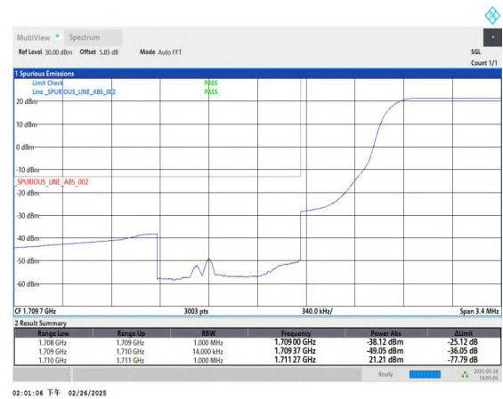
Band66_1.4MHz_16QAM_131979_1RB#5
