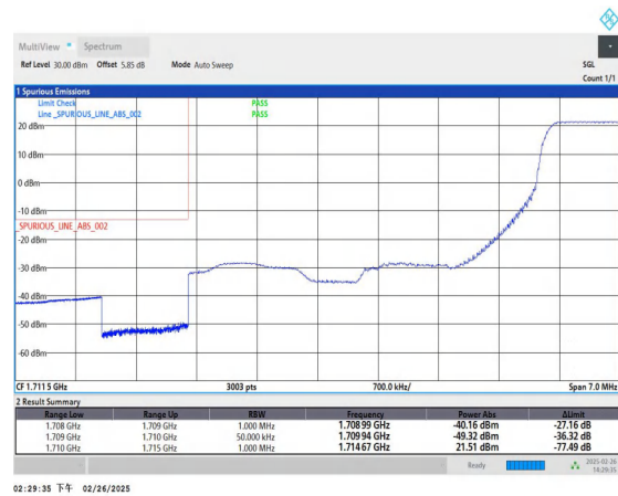
Band66_5MHz_16QAM_131997_1RB#24
