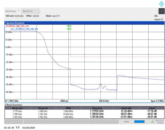
Band66_1.4MHz_16QAM_132665_1RB#0
