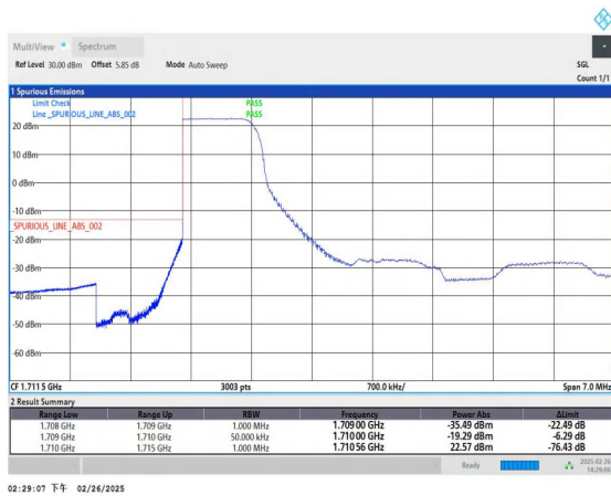
Band66_5MHz_QPSK_131997_1RB#0
