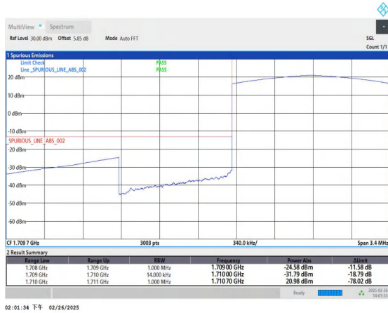
Band66_1.4MHz_16QAM_131979_6RB#0
