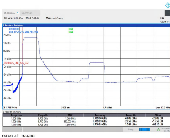
Band66_15MHz_QPSK_132047_1RB#0
