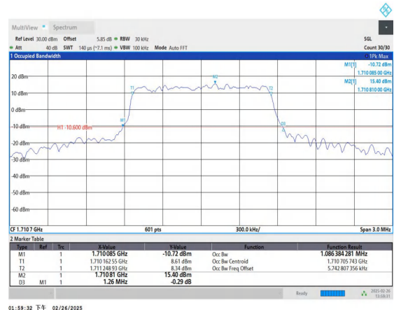
Band66-1.4MHz-16QAM-131979-6RB#0-PASS
