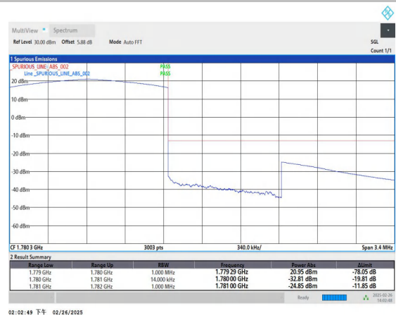
Band66_1.4MHz_QPSK_132665_6RB#0
