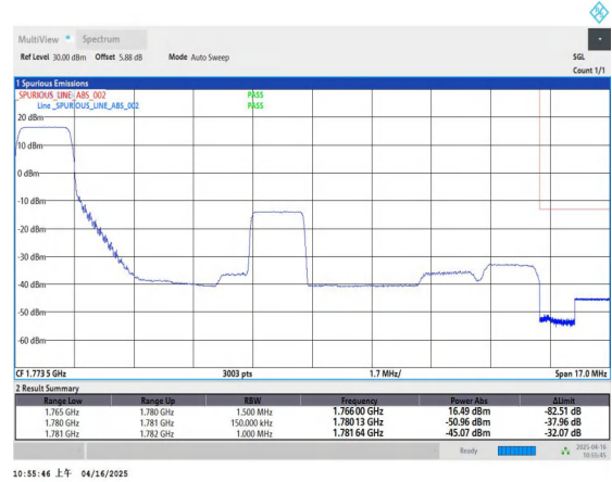
Band66_15MHz_QPSK_132597_1RB#0
