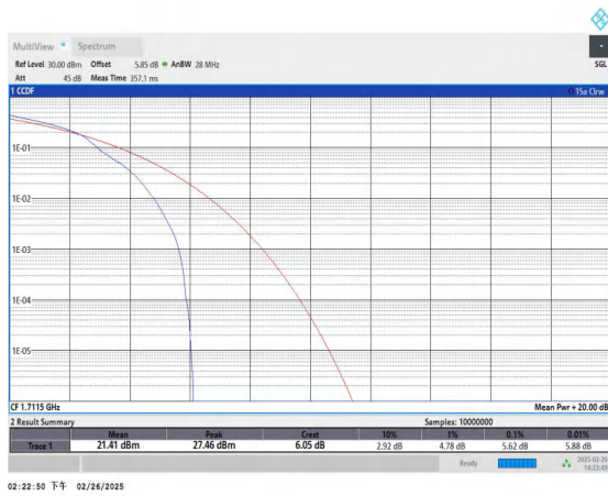
Band66-3MHz-16QAM-131987-1RB#0-PASS
