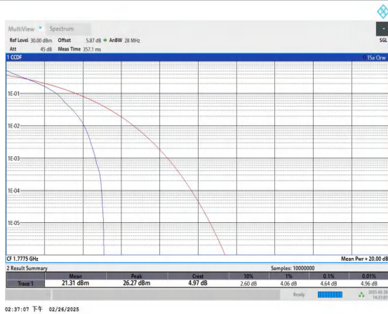
Band66-5MHz-QPSK-132647-1RB#0-PASS
