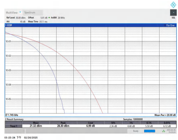
Band66-20MHz-QPSK-132322-100RB#0-PASS
