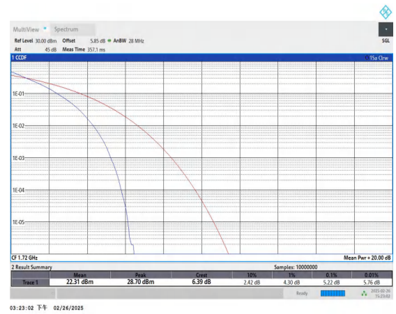
Band66-20MHz-QPSK-132072-100RB#0-PASS
