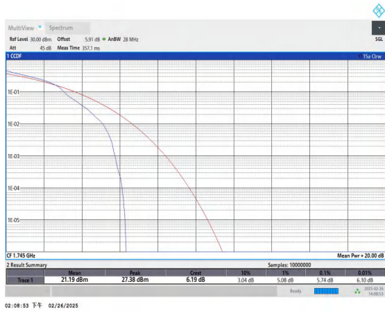
Band66-1.4MHz-16QAM-132322-1RB#0-PASS
