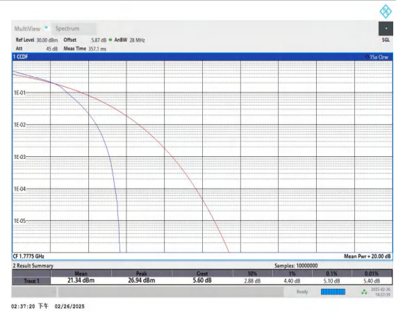
Band66-5MHz-16QAM-132647-25RB#0-PASS
