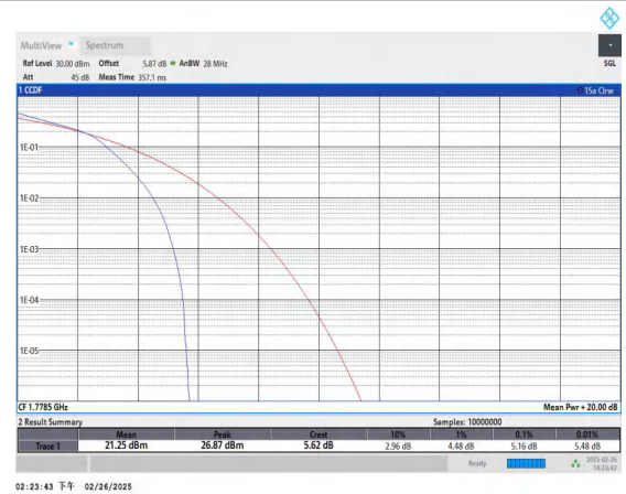
Band66-3MHz-16QAM-132657-15RB#0-PASS
