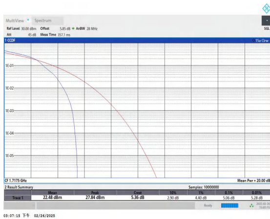
Band66-15MHz-16QAM-132047-1RB#0-PASS
