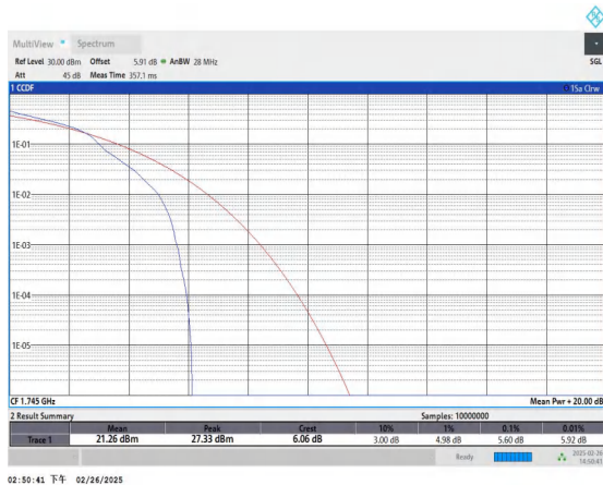
Band66-10MHz-16QAM-132322-1RB#0-PASS
