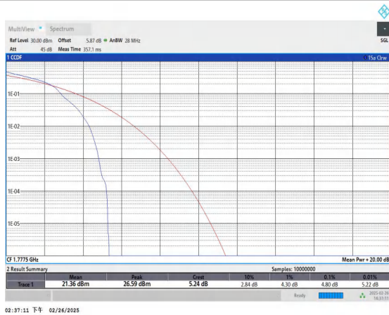
Band66-5MHz-16QAM-132647-1RB#0-PASS
