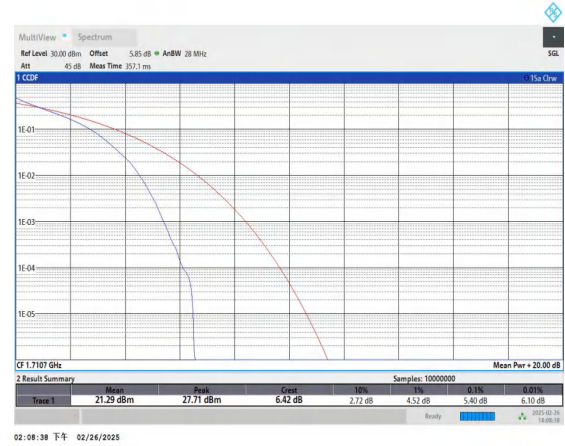
Band66-1.4MHz-QPSK-131979-6RB#0-PASS
