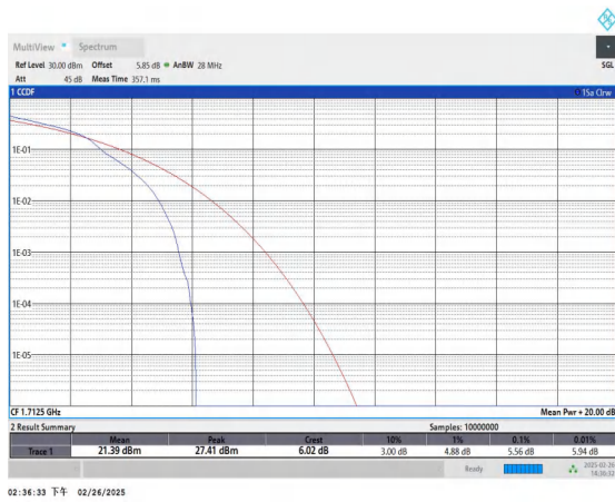
Band66-5MHz-16QAM-131997-1RB#0-PASS
