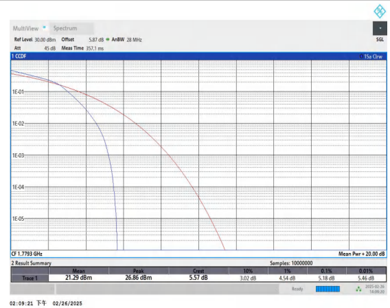
Band66-1.4MHz-16QAM-132665-6RB#0-PASS
