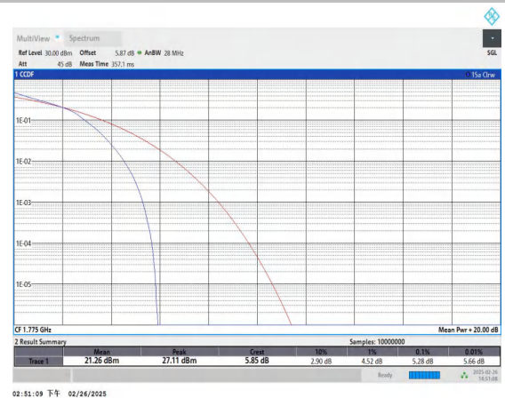
Band66-10MHz-16QAM-132622-50RB#0-PASS
