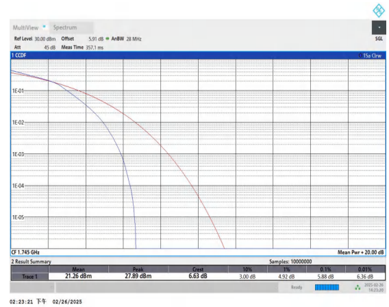
Band66-3MHz-16QAM-132322-15RB#0-PASS
