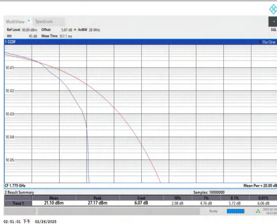
Band66-10MHz-16QAM-132622-1RB#0-PASS
