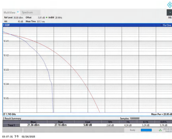
Band66-15MHz-QPSK-132322-1RB#0-PASS
