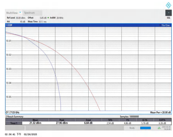
Band66-5MHz-16QAM-131997-25RB#0-PASS
