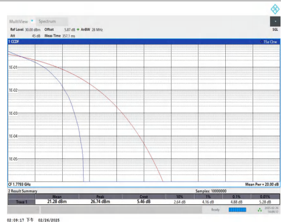
Band66-1.4MHz-QPSK-132665-6RB#0-PASS
