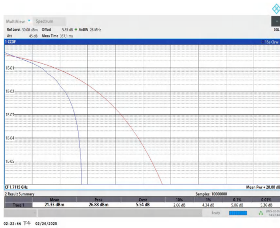
Band66-3MHz-QPSK-131987-1RB#0-PASS
