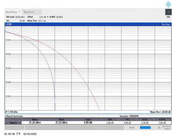
Band66-1.4MHz-QPSK-132322-6RB#0-PASS
