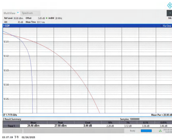
Band66-15MHz-QPSK-132047-1RB#0-PASS
