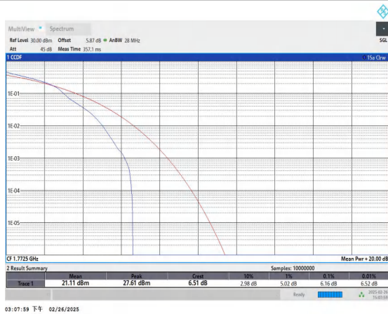
Band66-15MHz-16QAM-132597-1RB#0-PASS
