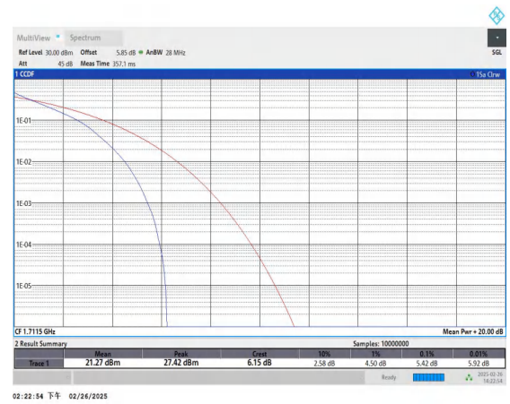
Band66-3MHz-QPSK-131987-15RB#0-PASS
