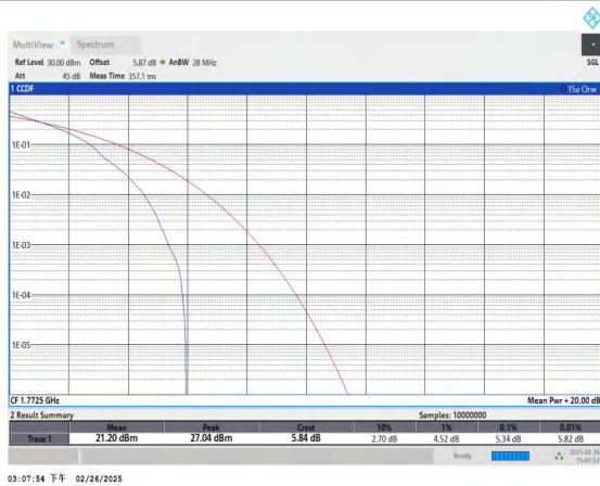
Band66-15MHz-QPSK-132597-1RB#0-PASS
