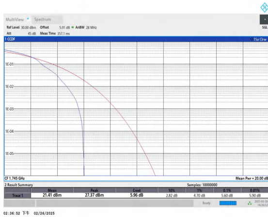
Band66-5MHz-16QAM-132322-1RB#0-PASS
