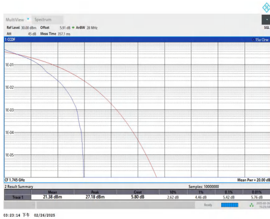
Band66-20MHz-QPSK-132322-1RB#0-PASS
