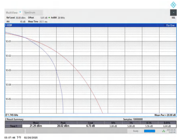
Band66-15MHz-16QAM-132322-75RB#0-PASS
