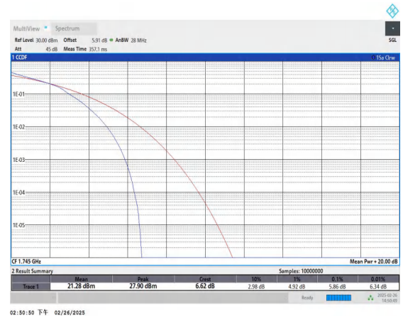
Band66-10MHz-16QAM-132322-50RB#0-PASS
