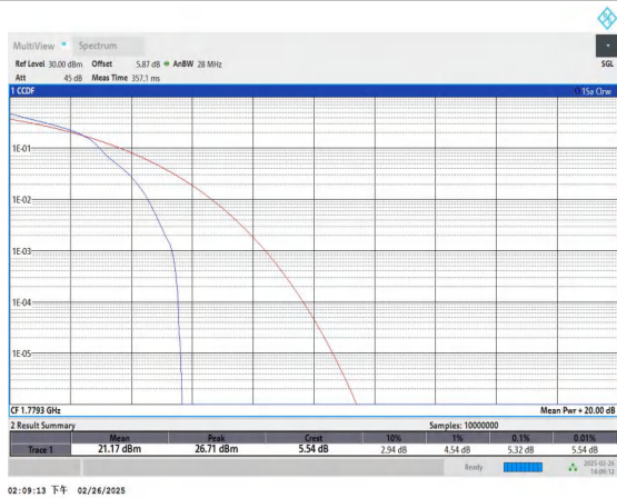
Band66-1.4MHz-16QAM-132665-1RB#0-PASS
