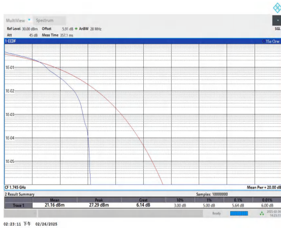
Band66-3MHz-16QAM-132322-1RB#0-PASS
