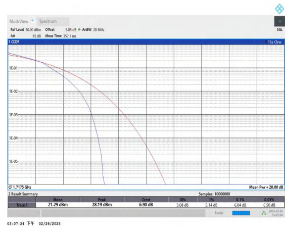
Band66-15MHz-16QAM-132047-75RB#0-PASS
