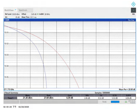
Band66-10MHz-QPSK-132022-50RB#0-PASS
