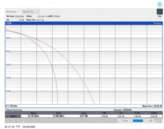
Band66-5MHz-16QAM-132322-25RB#0-PASS
