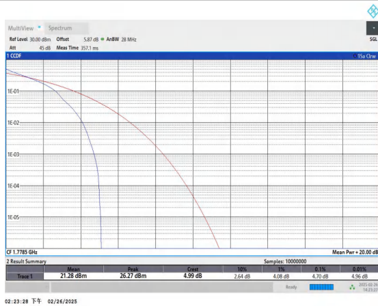
Band66-3MHz-QPSK-132657-1RB#0-PASS
