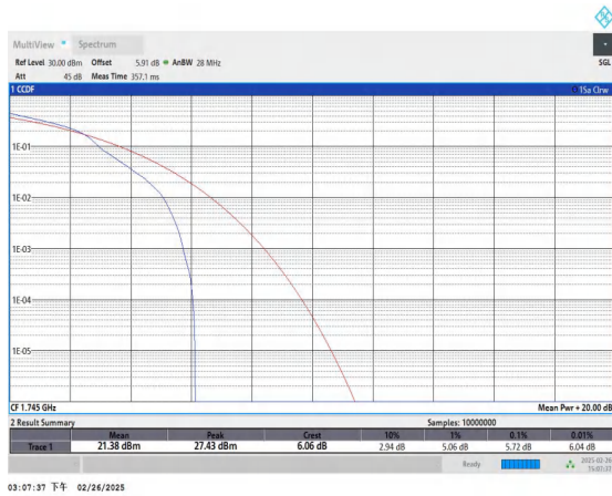
Band66-15MHz-16QAM-132322-1RB#0-PASS
