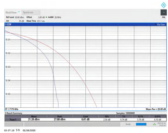
Band66-15MHz-QPSK-132047-75RB#0-PASS
