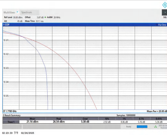
Band66-3MHz-16QAM-132657-1RB#0-PASS
