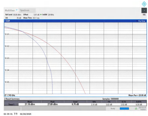
Band66-1.4MHz-16QAM-132322-6RB#0-PASS
