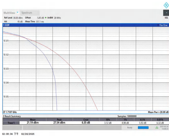
Band66-1.4MHz-16QAM-131979-1RB#0-PASS
