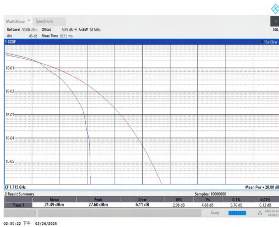
Band66-10MHz-16QAM-132022-1RB#0-PASS
