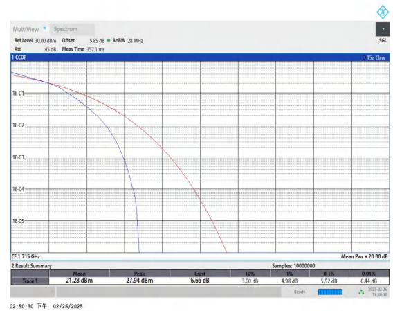
Band66-10MHz-16QAM-132022-50RB#0-PASS
