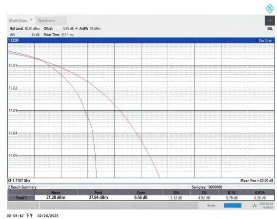
Band66-1.4MHz-16QAM-131979-6RB#0-PASS
