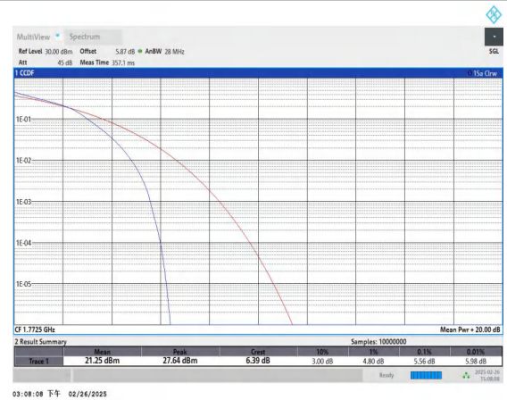
Band66-15MHz-16QAM-132597-75RB#0-PASS
