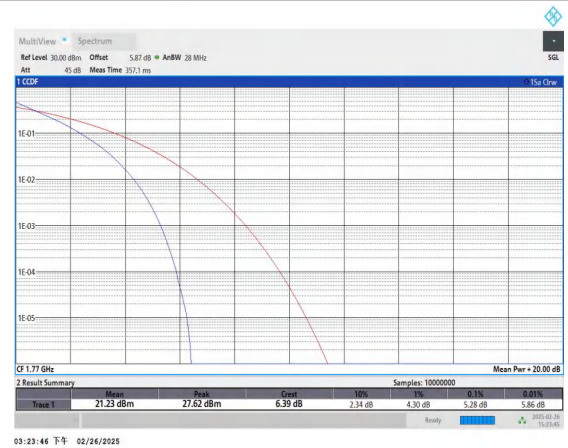
Band66-20MHz-QPSK-132572-100RB#0-PASS
