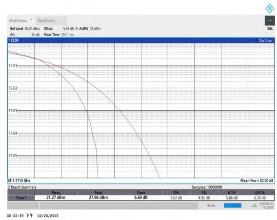
Band66-3MHz-16QAM-131987-15RB#0-PASS
