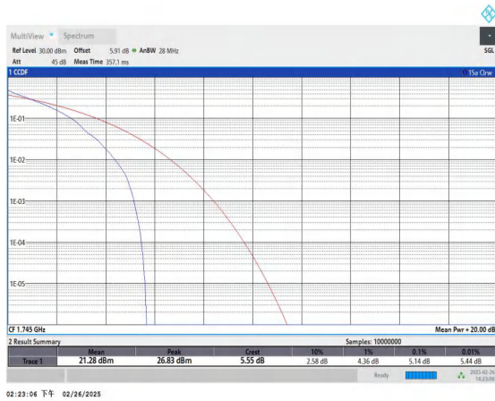
Band66-3MHz-QPSK-132322-1RB#0-PASS
