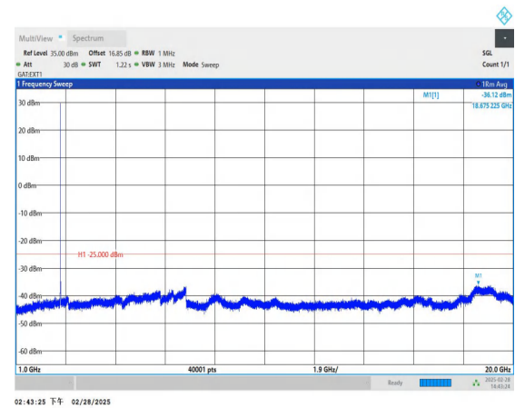
Band41_5MHz_QPSK_41565_1RB#0_1000~20000_1000~2000
