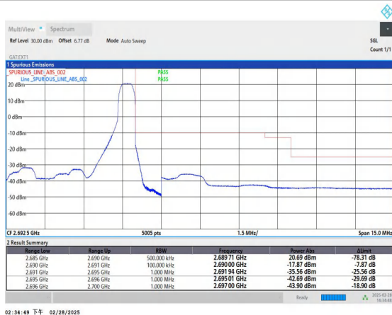
Band41_5MHz_QPSK_41565_1RB#24
