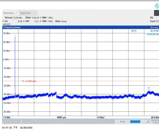
Band41_15MHz_16QAM_39765_1RB#0_1000~20000_1000~20000
