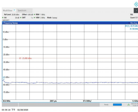
Band41_10MHz_QPSK_39740_1RB#0_30~1000_30~1000
