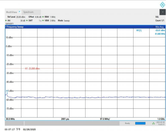
Band41_10MHz_16QAM_39740_1RB#0_30~1000_30~1000
