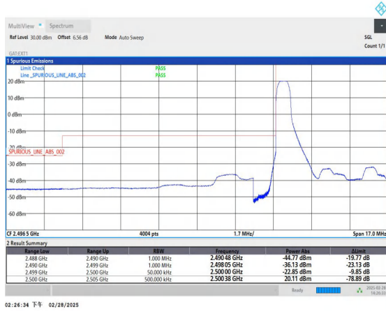
Band41_5MHz_QPSK_39715_1RB#0
