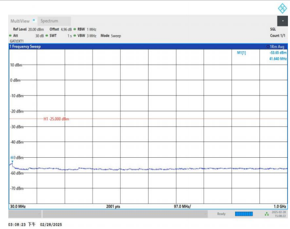
Band41_10MHz_QPSK_40620_1RB#0_30~1000_30~1000
