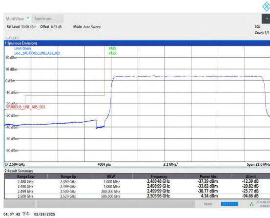
Band41_20MHz_QPSK_39790_100RB#0
