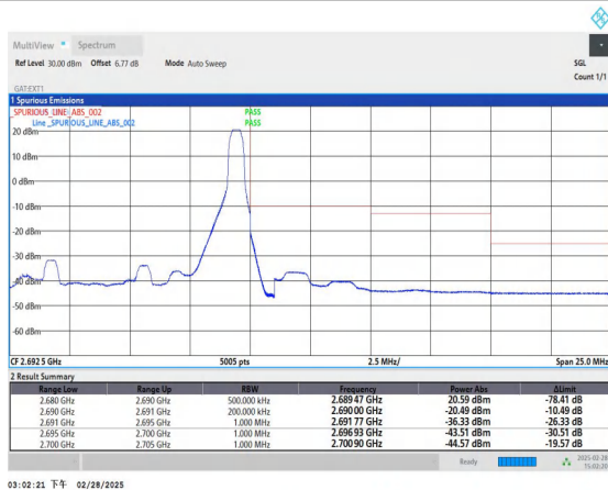
Band41_10MHz_QPSK_41540_1RB#49
