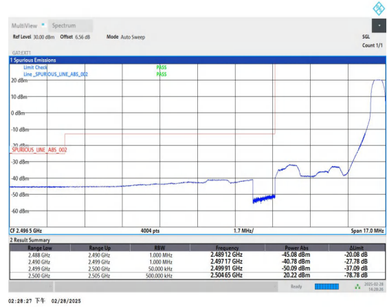
Band41_5MHz_QPSK_39715_1RB#24
