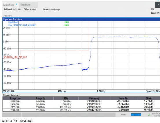
Band41_10MHz_QPSK_39740_50RB#0
