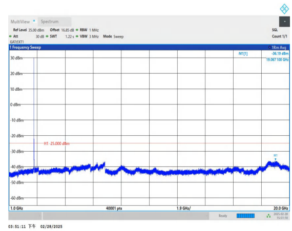
Band41_15MHz_QPSK_41515_1RB#0_1000~20000_1000~2000
