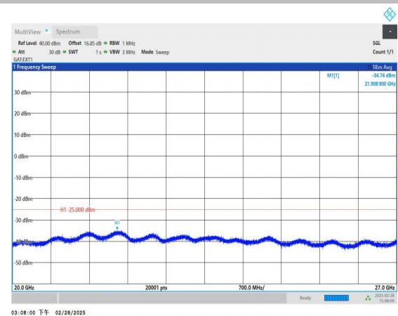
Band41_10MHz_16QAM_39740_1RB#0_20000~27000_20000~27000
