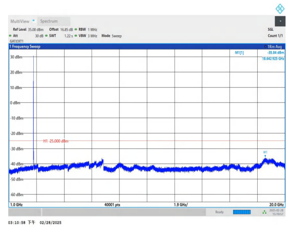
Band41_10MHz_QPSK_41540_1RB#0_1000~20000_1000~2000
