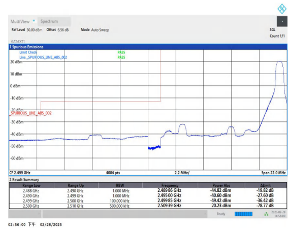
Band41_10MHz_QPSK_39740_1RB#49
