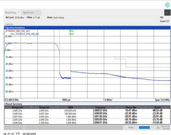
Band41_5MHz_QPSK_41565_25RB#0
