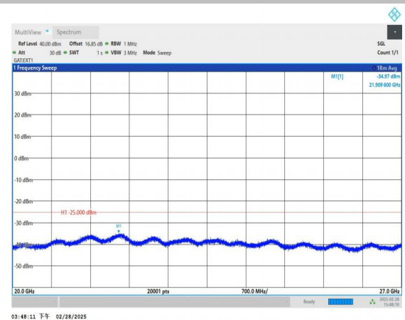
Band41_15MHz_16QAM_39765_1RB#0_20000~27000_20000~27000
