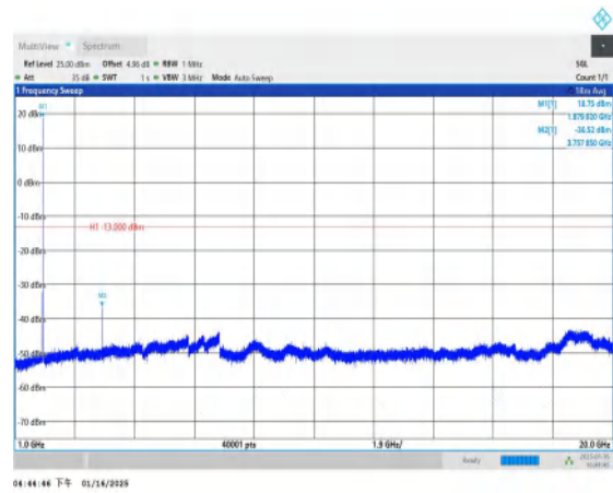
Band2-9400-1000~20000MHz-PASS
