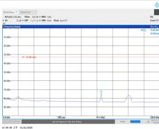
Band5-4233-0.009~0.15MHz-PASS
