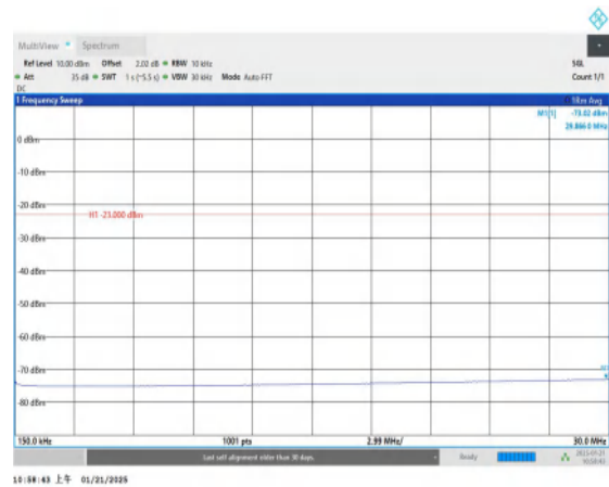
Band5-4132-0.15~30MHz-PASS
