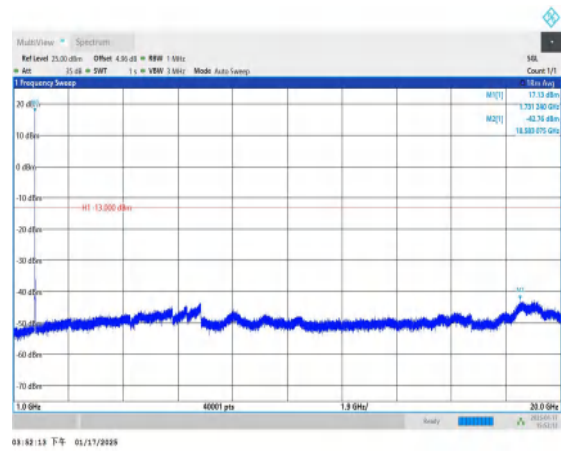
Band4-1413-1000~20000MHz-PASS
