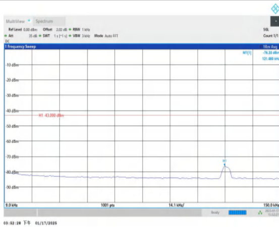
Band4-1513-0.009~0.15MHz-PASS
