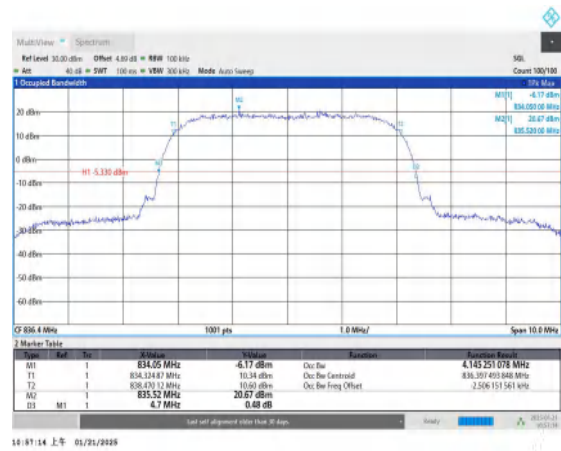
Band5-4182-PASS
