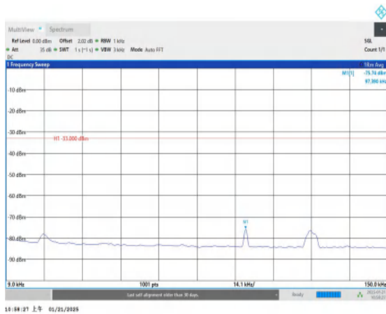
Band5-4132-0.009~0.15MHz-PASS
