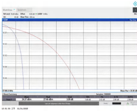
Band5-4233-PASS
