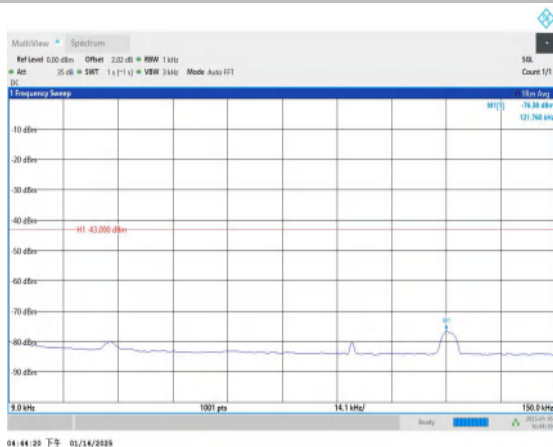
Band2-9400-0.009~0.15MHz-PASS
