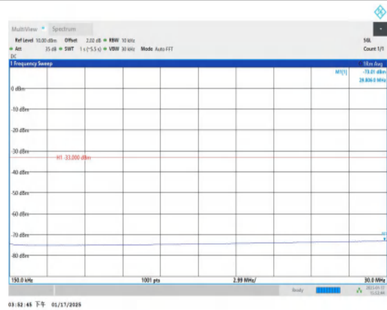
Band4-1513-0.15~30MHz-PASS
