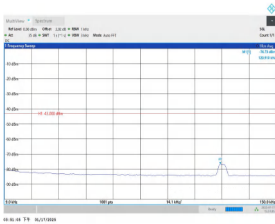
Band4-1312-0.009~0.15MHz-PASS
