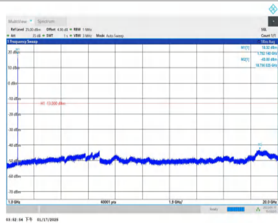
Band4-1513-1000~20000MHz-PASS
