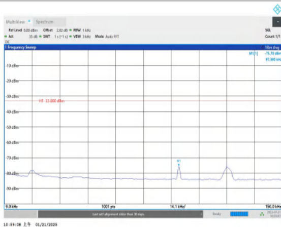
Band5-4182-0.009~0.15MHz-PASS
