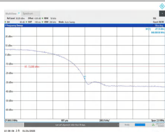
Band5-4233-PASS
