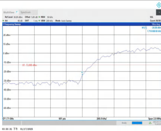
Band4-1312-PASS
