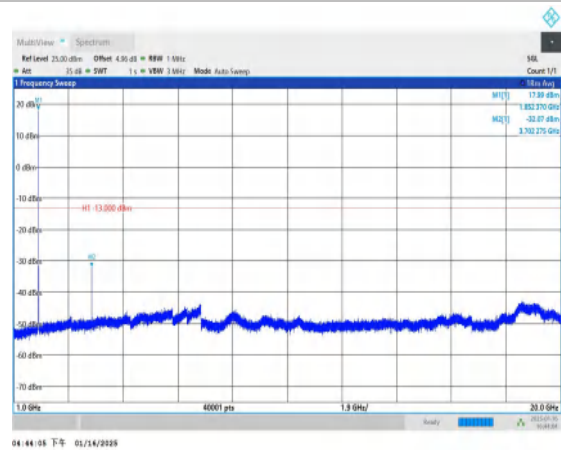
Band2-9262-1000~20000MHz-PASS
