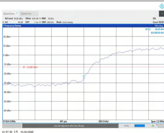
Band5-4132-PASS
