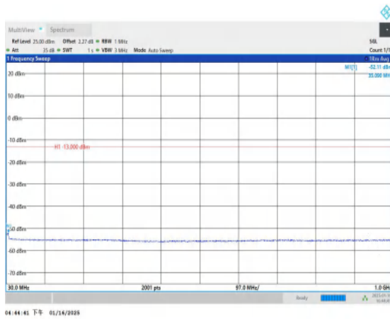
Band2-9400-30~1000MHz-PASS
