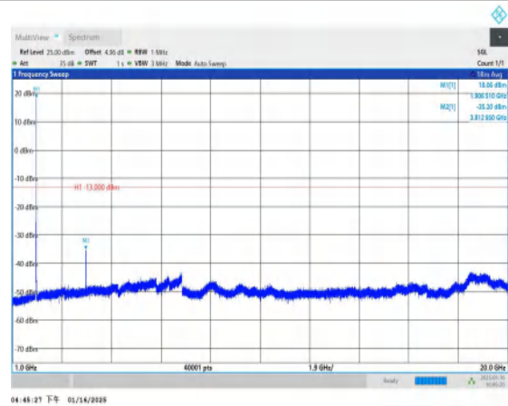
Band2-9538-1000~20000MHz-PASS
