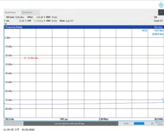
Band5-4233-0.15~30MHz-PASS
