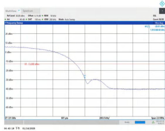
Band2-9538-PASS
