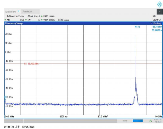
Band5_10MHz_QPSK_20525_1RB#0_30~1000_30~1000
