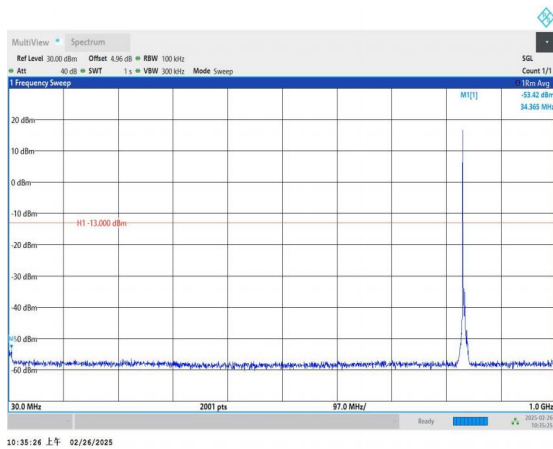
Band5_5MHz_16QAM_20525_1RB#0_30~1000_30~1000
