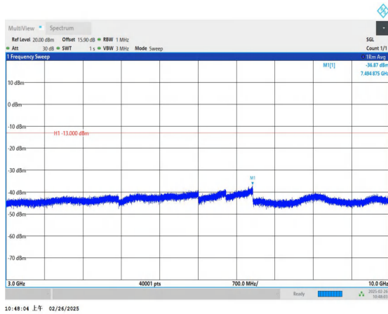
Band5_10MHz_QPSK_20450_1RB#0_3000~10000_3000~1000
