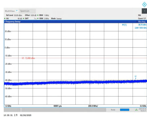
Band5_5MHz_16QAM_20525_1RB#0_1000~3000_1000~3000
