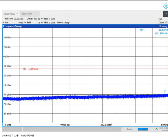
Band5_10MHz_QPSK_20525_1RB#0_1000~3000_1000~3000
