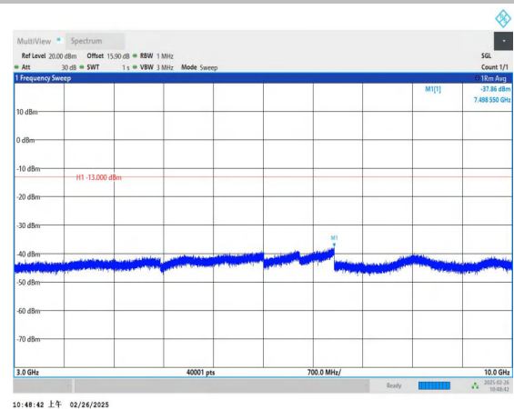
Band5_10MHz_QPSK_20525_1RB#0_3000~10000_3000~1000
