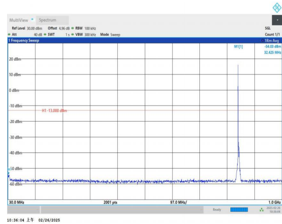
Band5_5MHz_16QAM_20625_1RB#0_30~1000_30~1000
