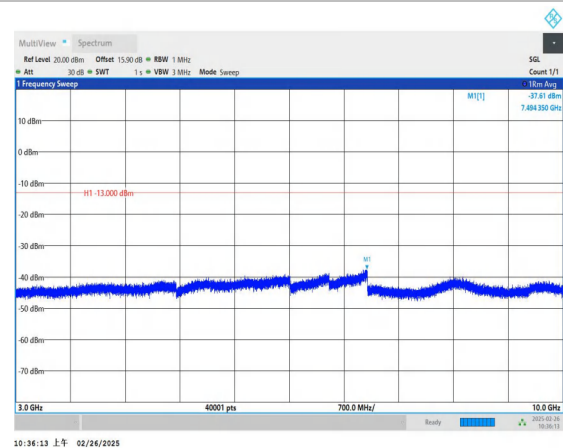
Band5_5MHz_16QAM_20625_1RB#0_3000~10000_3000~10000
