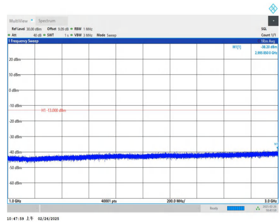
Band5_10MHz_QPSK_20450_1RB#0_1000~3000_1000~3000
