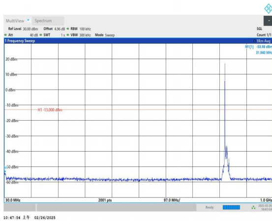
Band5_10MHz_QPSK_20450_1RB#0_30~1000_30~1000
