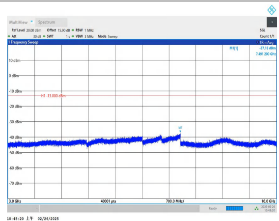
Band5_10MHz_16QAM_20450_1RB#0_3000~10000_3000~10
