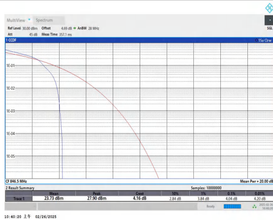
Band5-5MHz-16QAM-20625-1RB#0-PASS
