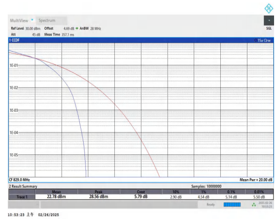
Band5-10MHz-16QAM-20450-50RB#0-PASS
