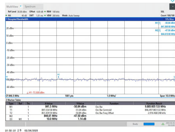
Band5-5MHz-16QAM-20625-25RB#0-PASS
