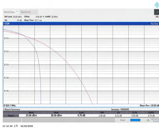
Band5-1.4MHz-16QAM-20407-1RB#0-PASS
