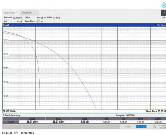
Band5-3MHz-16QAM-20415-1RB#0-PASS
