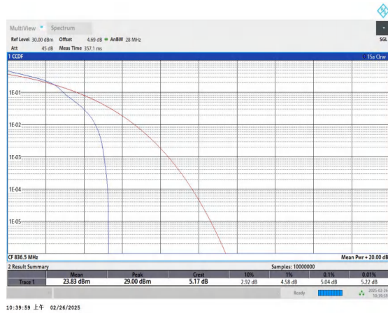
Band5-5MHz-16QAM-20525-1RB#0-PASS
