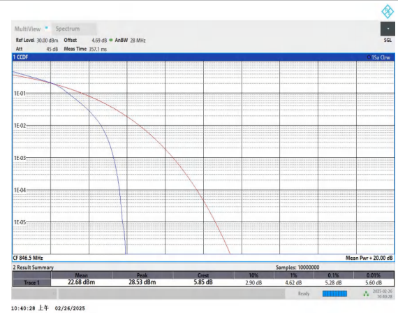
Band5-5MHz-16QAM-20625-25RB#0-PASS
