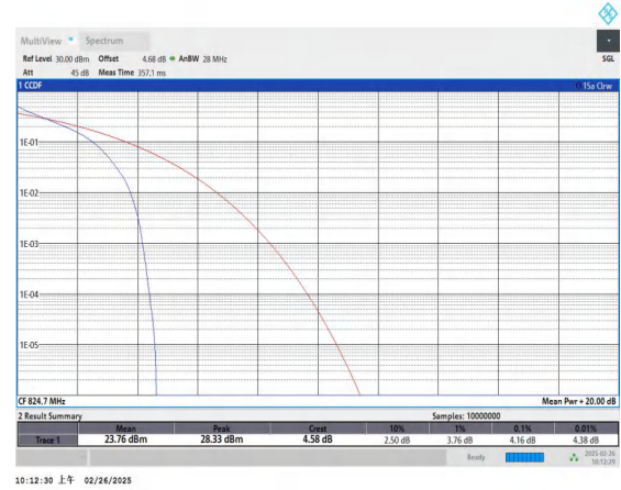
Band5-1.4MHz-QPSK-20407-6RB#0-PASS
