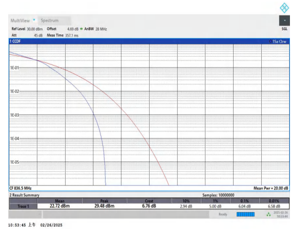
Band5-10MHz-16QAM-20525-50RB#0-PASS
