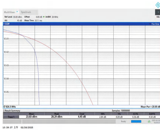
Band5-5MHz-16QAM-20425-1RB#0-PASS
