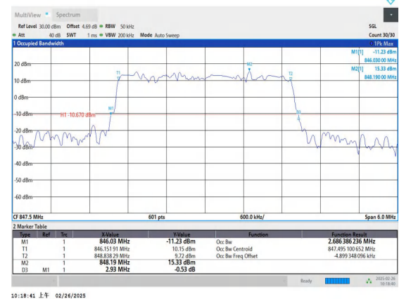
Band5-3MHz-16QAM-20635-15RB#0-PASS
