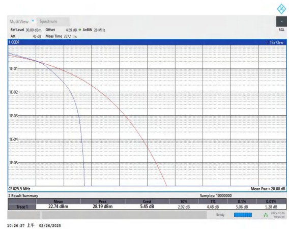
Band5-3MHz-16QAM-20415-15RB#0-PASS
