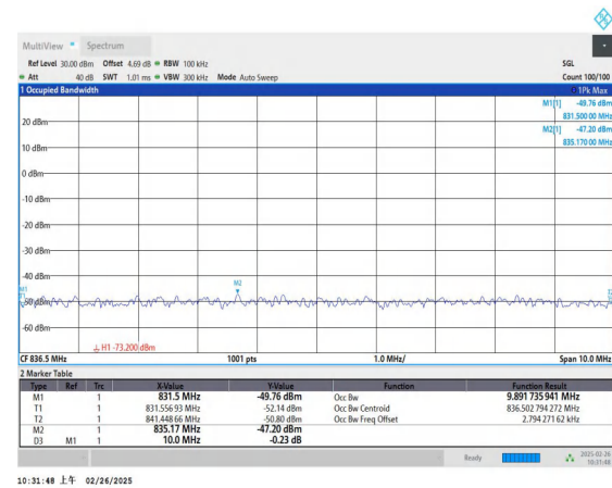
Band5-5MHz-QPSK-20525-25RB#0-PASS
