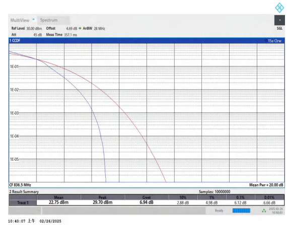
Band5-5MHz-16QAM-20525-25RB#0-PASS
