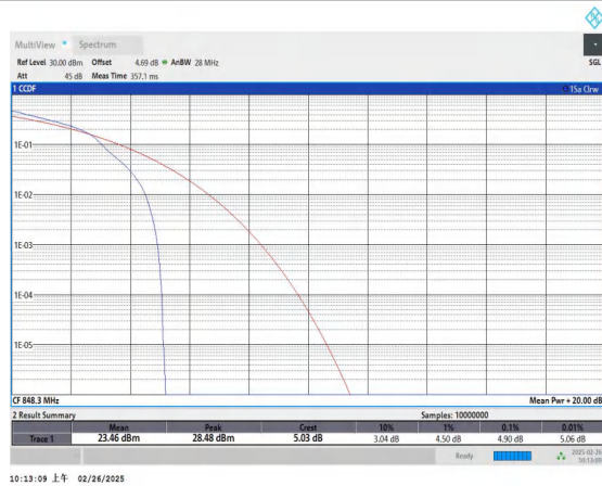
Band5-1.4MHz-16QAM-20643-1RB#0-PASS
