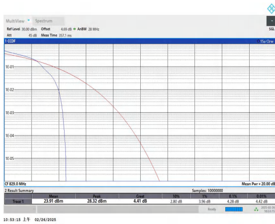
Band5-10MHz-16QAM-20450-1RB#0-PASS
