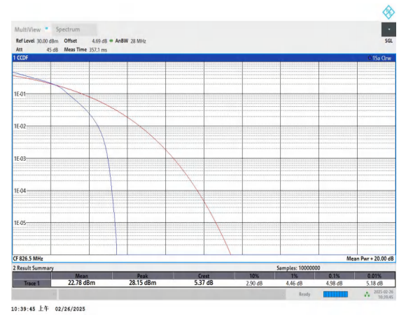
Band5-5MHz-16QAM-20425-25RB#0-PASS
