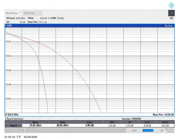
Band5-10MHz-QPSK-20450-50RB#0-PASS
