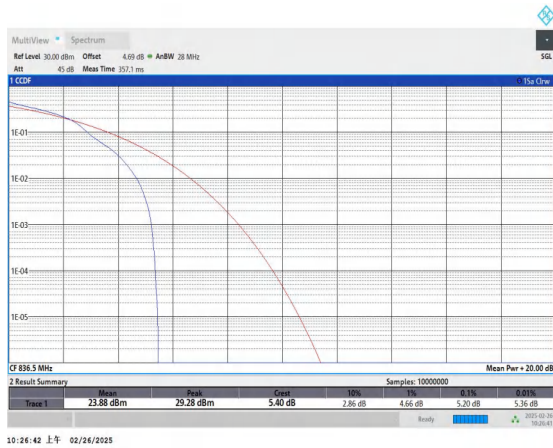
Band5-3MHz-16QAM-20525-1RB#0-PASS
