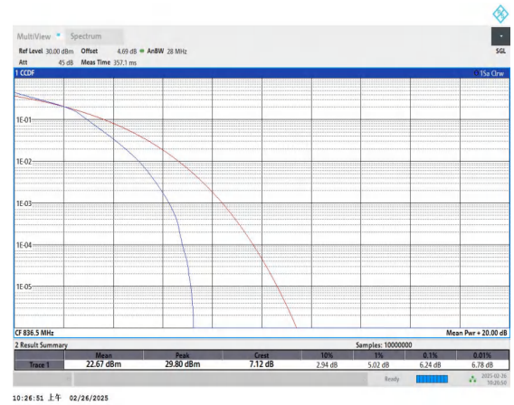
Band5-3MHz-16QAM-20525-15RB#0-PASS
