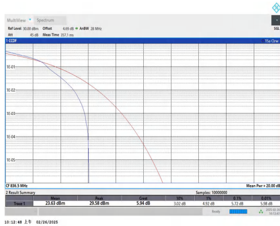
Band5-1.4MHz-16QAM-20525-1RB#0-PASS
