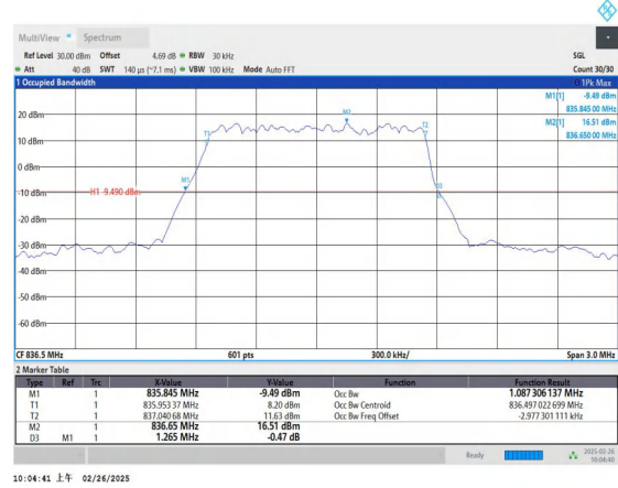
Band5-1.4MHz-QPSK-20525-6RB#0-PASS
