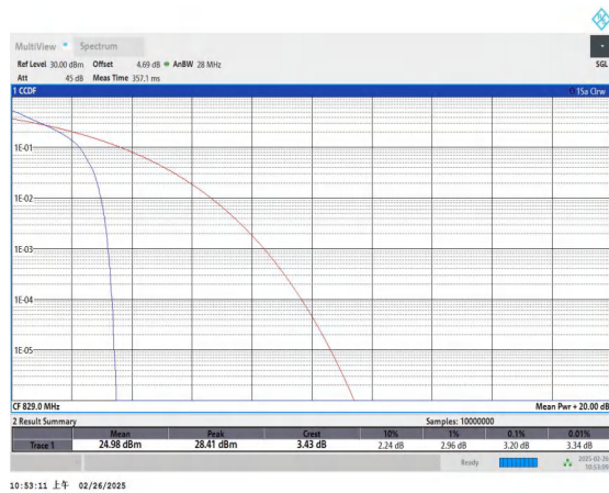
Band5-10MHz-QPSK-20450-1RB#0-PASS
