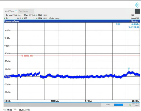
Band4_10MHz_16QAM_20350_1RB#0_3000~20000_3000~20
