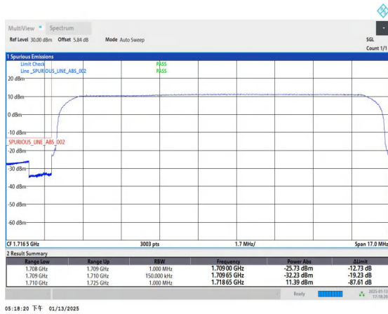
Band4_15MHz_16QAM_20025_75RB#0
