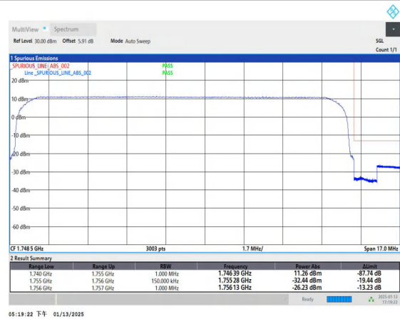
Band4_15MHz_16QAM_20325_75RB#0
