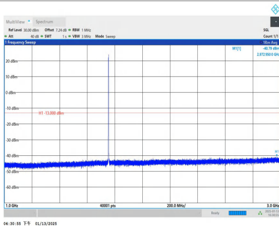
Band4_1.4MHz_16QAM_20393_1RB#0_1000~3000_1000~3000 0
