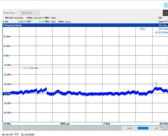
Band4_3MHz_QPSK_20385_1RB#0_3000~20000_3000~20000
