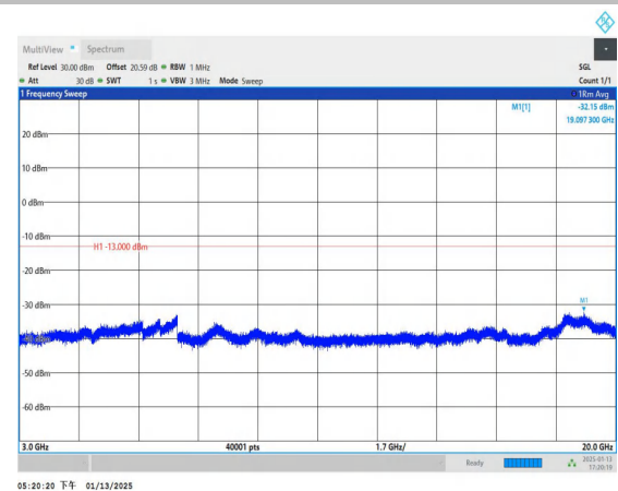
Band4_15MHz_QPSK_20175_1RB#0_3000~20000_3000~2000
