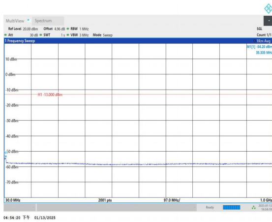
Band4_5MHz_QPSK_19975_1RB#0_30~1000_30~1000
