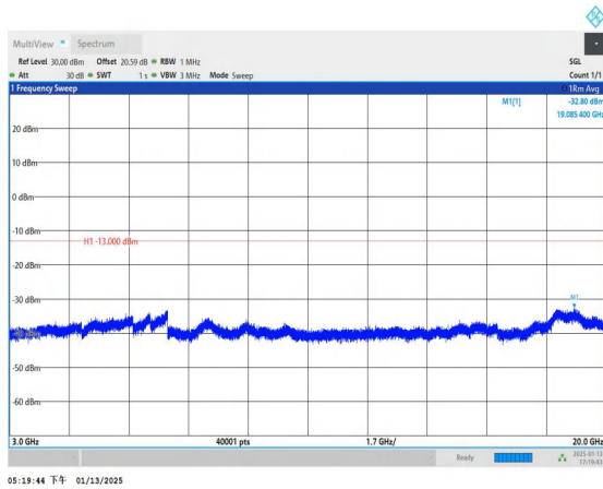
Band4_15MHz_QPSK_20025_1RB#0_3000~20000_3000~2000
