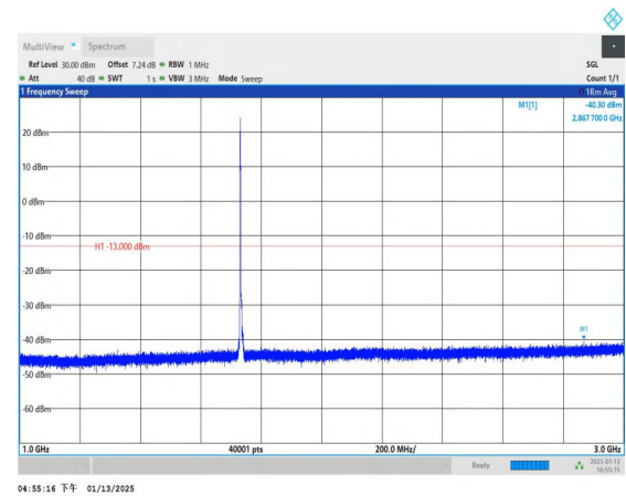
Band4_5MHz_16QAM_20175_1RB#0_1000~3000_1000~3000
