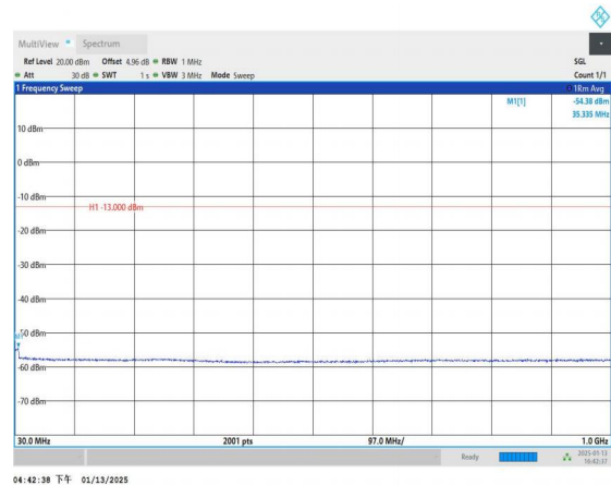
Band4_3MHz_QPSK_20175_1RB#0_30~1000_30~1000
