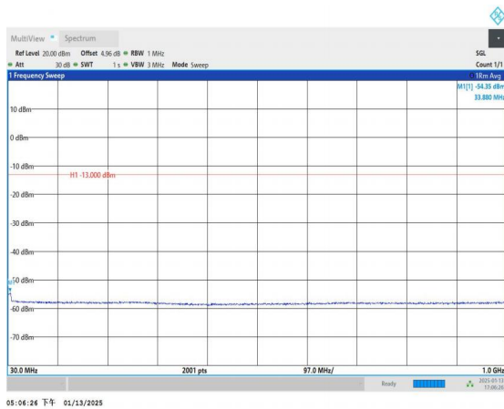
Band4_10MHz_QPSK_20000_1RB#0_30~1000_30~1000
