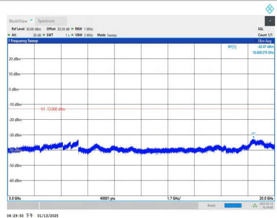
Band4_1.4MHz_16QAM_19957_1RB#0_3000~20000_3000~20000
