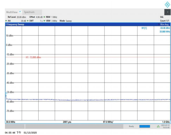
Band4_5MHz_16QAM_20375_1RB#0_30~1000_30~1000
