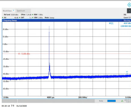
Band4_15MHz_QPSK_20175_1RB#0_1000~3000_1000~3000
