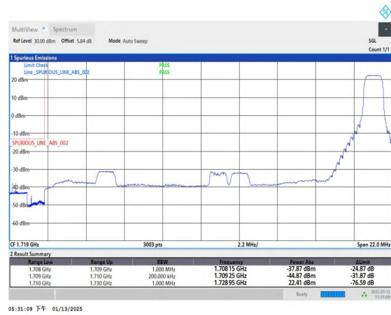
Band4_20MHz_16QAM_20050_1RB#99
