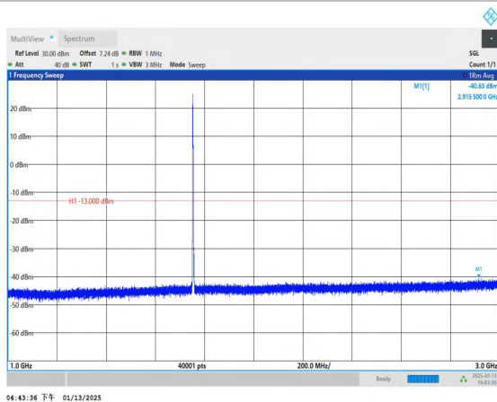
Band4_3MHz_16QAM_20385_1RB#0_1000~3000_1000~3000
