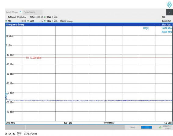
Band4_10MHz_16QAM_20000_1RB#0_30~1000_30~1000
