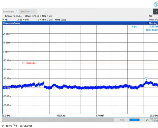
Band4_3MHz_16QAM_20175_1RB#0_3000~20000_3000~20000
