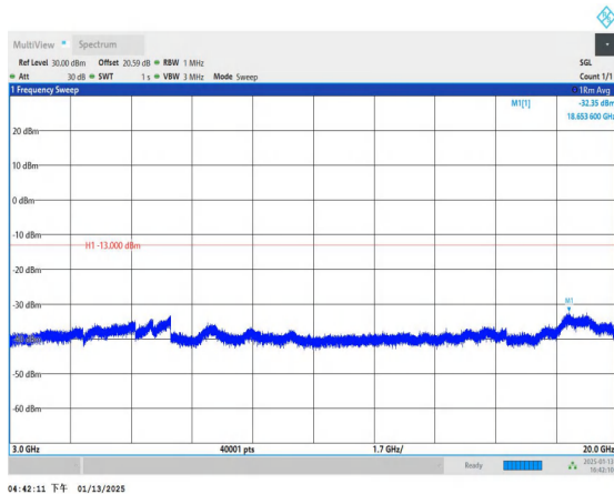
Band4_3MHz_QPSK_19965_1RB#0_3000~20000_3000~20000
