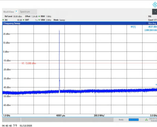
Band4_3MHz_QPSK_20175_1RB#0_1000~3000_1000~3000
