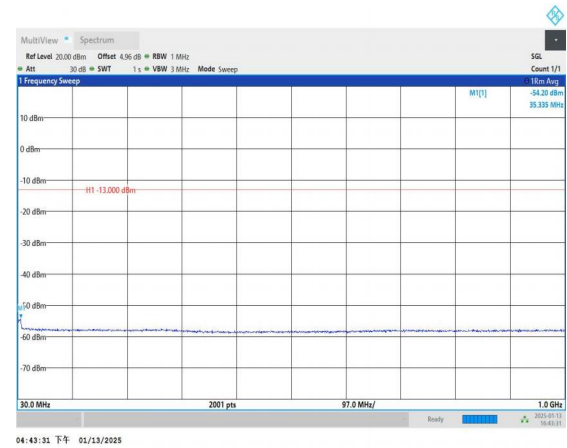
Band4_3MHz_16QAM_20385_1RB#0_30~1000_30~1000
