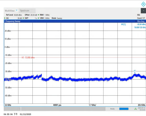
Band4_5MHz_QPSK_20175_1RB#0_3000~20000_3000~20000
