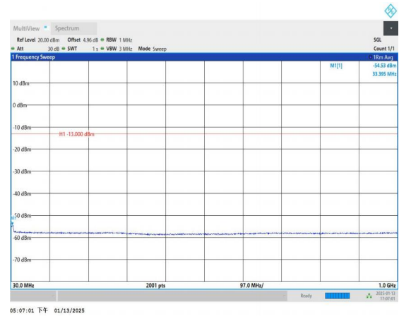
Band4_10MHz_QPSK_20175_1RB#0_30~1000_30~1000
