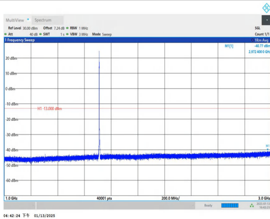
Band4_3MHz_16QAM_19965_1RB#0_1000~3000_1000~3000
