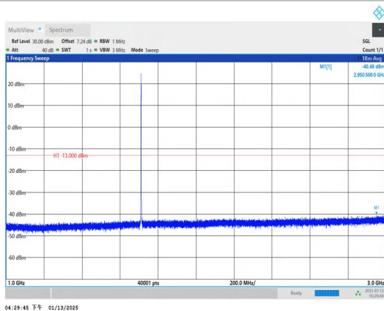
Band4_1.4MHz_16QAM_19957_1RB#0_1000~3000_1000~3000
