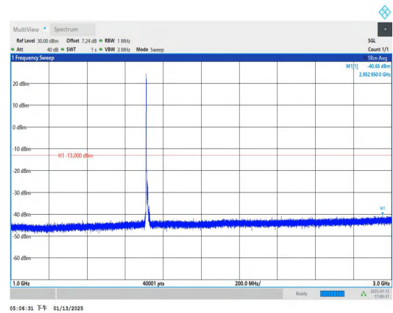
Band4_10MHz_QPSK_20000_1RB#0_1000~3000_1000~3000
