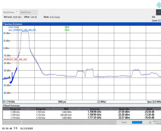
Band4_20MHz_16QAM_20050_1RB#0
