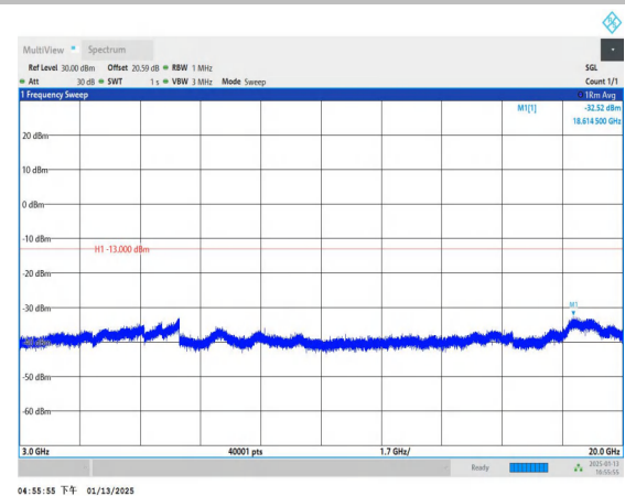
Band4_5MHz_16QAM_20375_1RB#0_3000~20000_3000~20000
