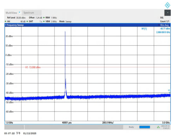
Band4_10MHz_16QAM_20175_1RB#0_1000~3000_1000~300
