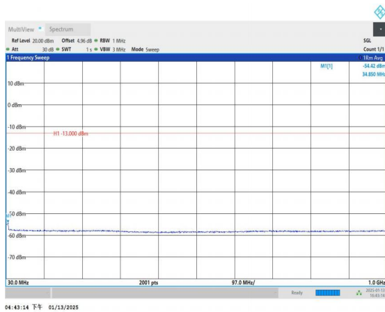
Band4_3MHz_QPSK_20385_1RB#0_30~1000_30~1000
