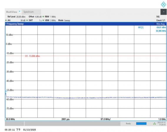
Band4_15MHz_QPSK_20175_1RB#0_30~1000_30~1000
