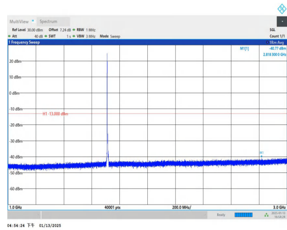
Band4_5MHz_QPSK_19975_1RB#0_1000~3000_1000~3000
