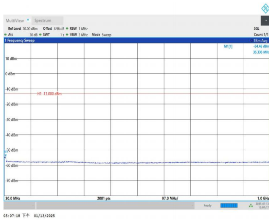
Band4_10MHz_16QAM_20175_1RB#0_30~1000_30~1000
