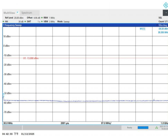
Band4_3MHz_16QAM_20175_1RB#0_30~1000_30~1000
