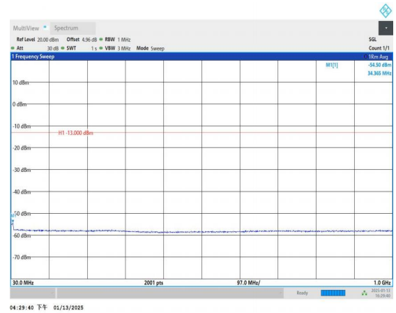
Band4_1.4MHz_16QAM_19957_1RB#0_30~1000_30~1000
