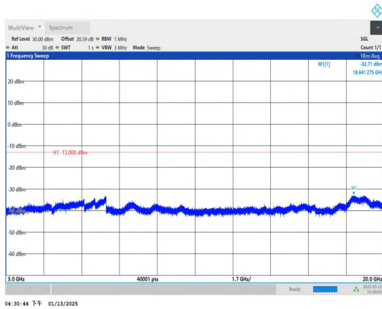
Band4_1.4MHz_QPSK_20393_1RB#0_3000~20000_3000~20000
