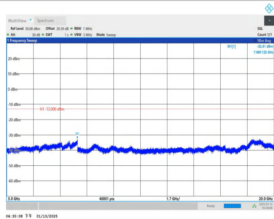
Band4_1.4MHz_QPSK_20175_1RB#0_3000~20000_3000~20000
