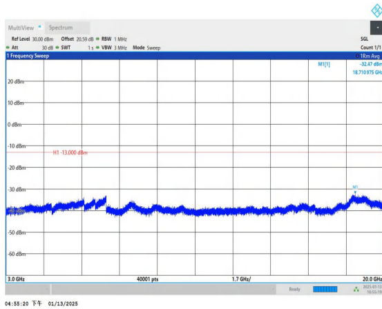
Band4_5MHz_16QAM_20175_1RB#0_3000~20000_3000~20000
