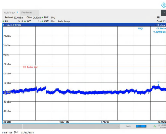
Band4_5MHz_QPSK_20375_1RB#0_3000~20000_3000~20000
