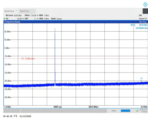
Band4_3MHz_QPSK_19965_1RB#0_1000~3000_1000~3000
