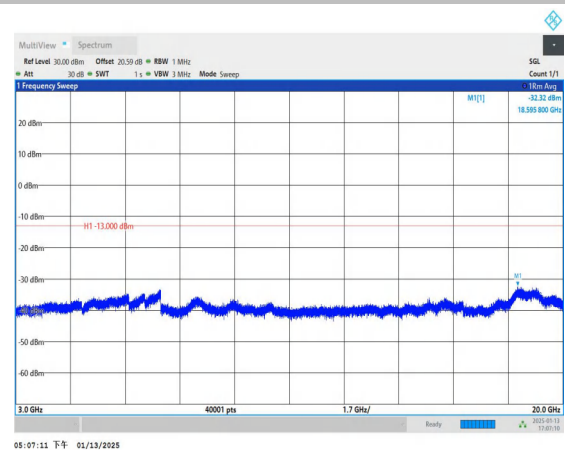
Band4_10MHz_QPSK_20175_1RB#0_3000~20000_3000~2000
