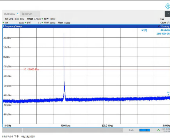
Band4_10MHz_QPSK_20175_1RB#0_1000~3000_1000~3000
