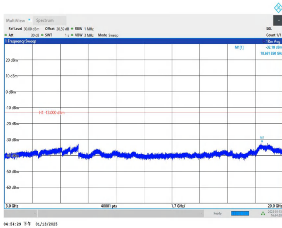
Band4_5MHz_QPSK_19975_1RB#0_3000~20000_3000~20000
