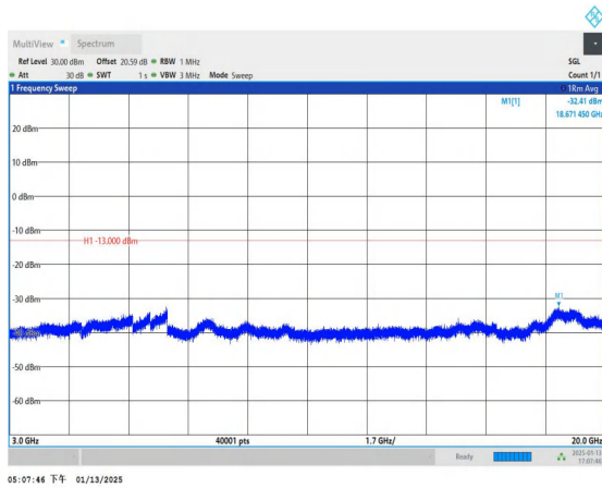
Band4_10MHz_QPSK_20350_1RB#0_3000~20000_3000~2000
