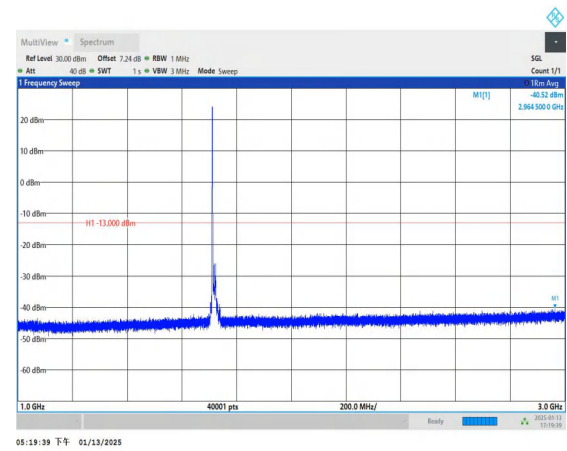
Band4_15MHz_QPSK_20025_1RB#0_1000~3000_1000~3000
