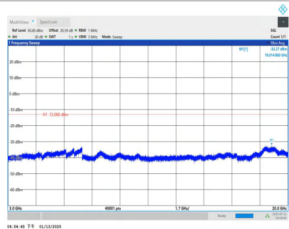
Band4_5MHz_16QAM_19975_1RB#0_3000~20000_3000~20000
