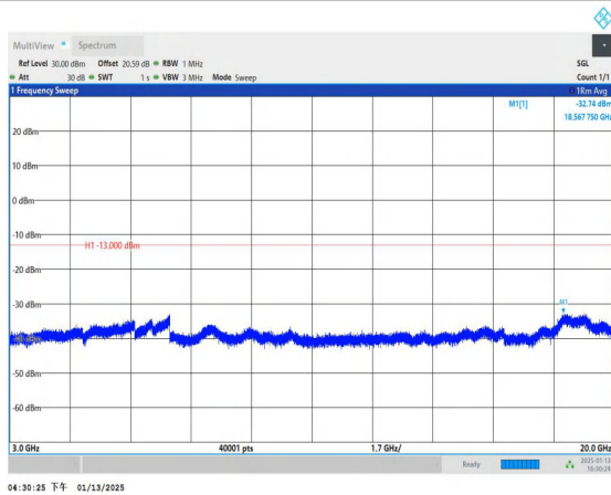
Band4_1.4MHz_16QAM_20175_1RB#0_3000~20000_3000~20000 000
