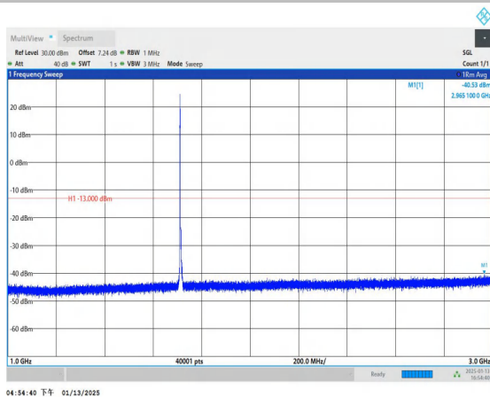
Band4_5MHz_16QAM_19975_1RB#0_1000~3000_1000~3000
