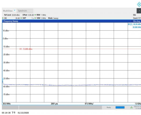
Band4_15MHz_QPSK_20025_1RB#0_30~1000_30~1000
