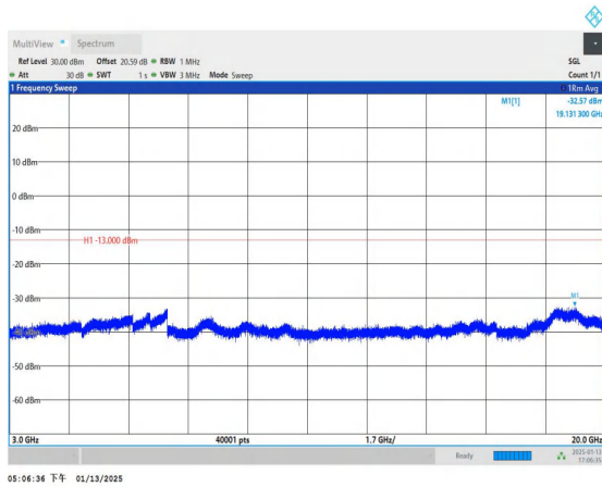
Band4_10MHz_QPSK_20000_1RB#0_3000~20000_3000~2000
