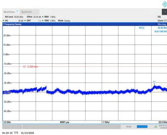
Band4_1.4MHz_QPSK_19957_1RB#0_3000~20000_3000~20000
