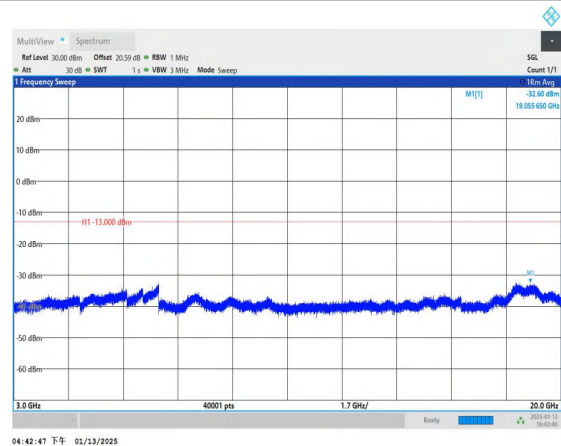
Band4_3MHz_QPSK_20175_1RB#0_3000~20000_3000~20000
