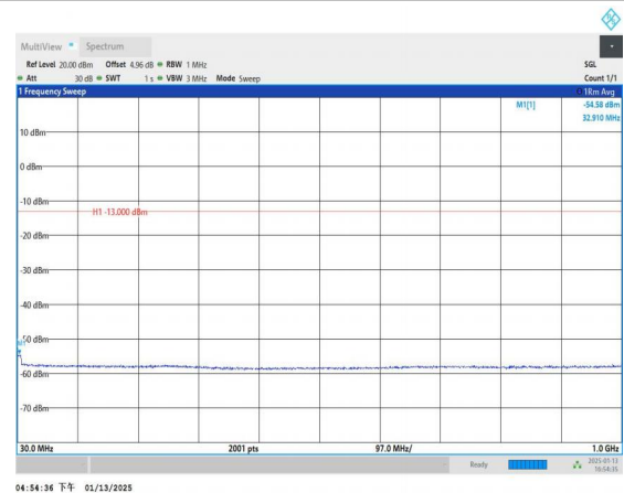
Band4_5MHz_16QAM_19975_1RB#0_30~1000_30~1000
