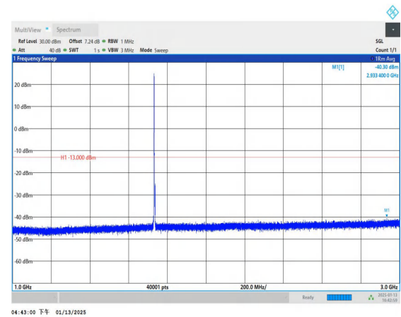
Band4_3MHz_16QAM_20175_1RB#0_1000~3000_1000~3000
