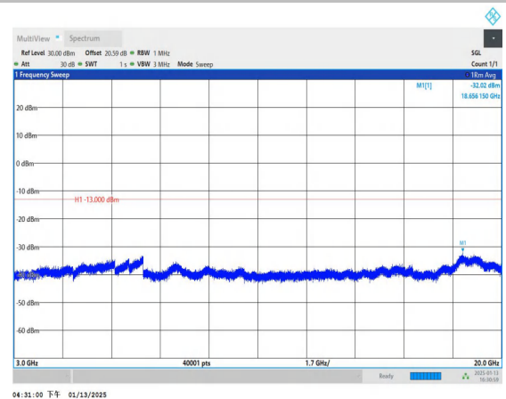
Band4_1.4MHz_16QAM_20393_1RB#0_3000~20000_3000~20000 000
