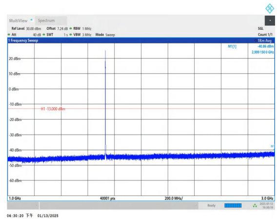
Band4_1.4MHz_16QAM_20175_1RB#0_1000~3000_1000~3000 0
