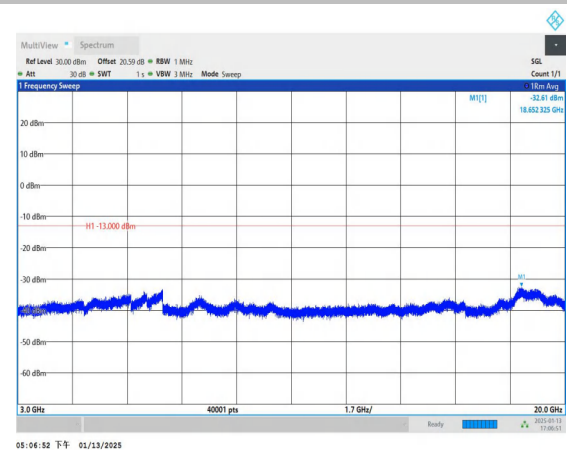
Band4_10MHz_16QAM_20000_1RB#0_3000~20000_3000~2000
