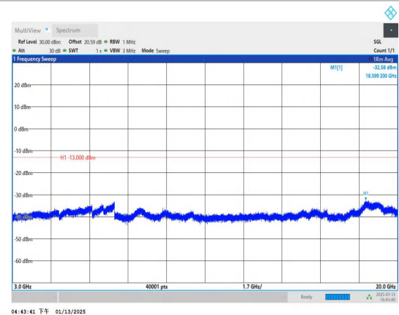
Band4_3MHz_16QAM_20385_1RB#0_3000~20000_3000~20000
