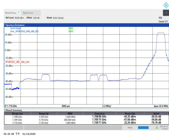
Band4_20MHz_QPSK_20050_1RB#99
