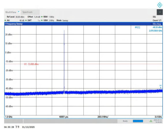
Band4_1.4MHz_QPSK_20393_1RB#0_1000~3000_1000~3000
