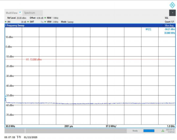
Band4_10MHz_16QAM_20350_1RB#0_30~1000_30~1000
