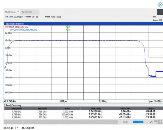
Band4_20MHz_QPSK_20300_100RB#0
