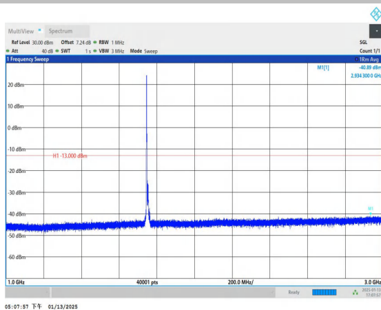
Band4_10MHz_16QAM_20350_1RB#0_1000~3000_1000~300
