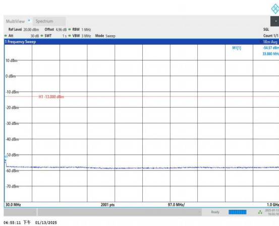
Band4_5MHz_16QAM_20175_1RB#0_30~1000_30~1000
