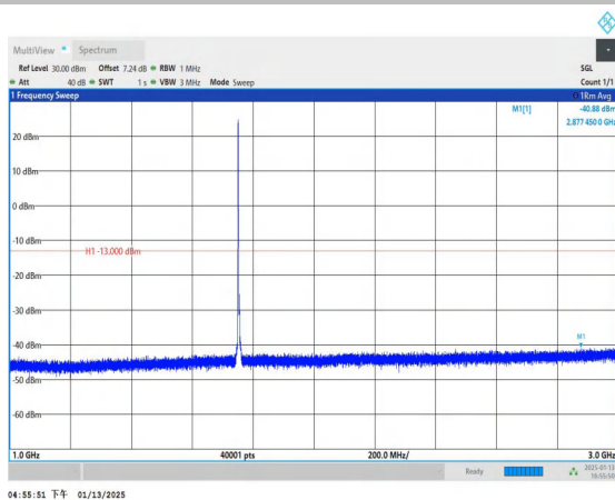
Band4_5MHz_16QAM_20375_1RB#0_1000~3000_1000~3000
