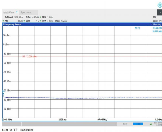
Band4_1.4MHz_16QAM_20175_1RB#0_30~1000_30~1000
