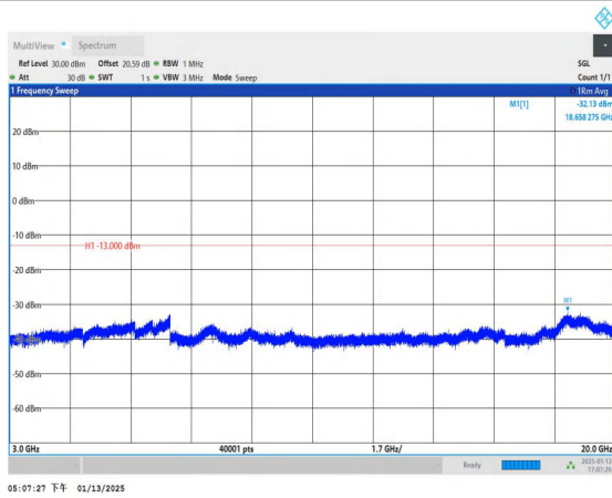
Band4_10MHz_16QAM_20175_1RB#0_3000~20000_3000~20
