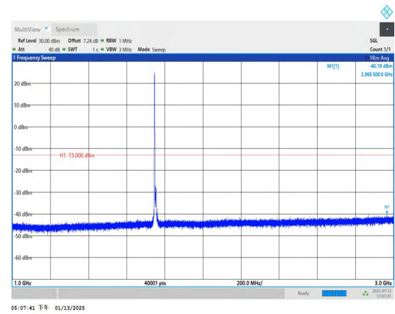
Band4_10MHz_QPSK_20350_1RB#0_1000~3000_1000~3000
