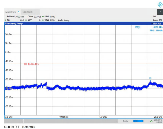
Band4_3MHz_16QAM_19965_1RB#0_3000~20000_3000~20000
