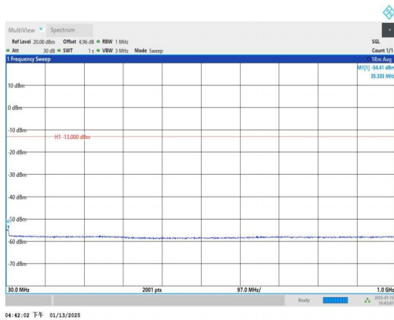
Band4_3MHz_QPSK_19965_1RB#0_30~1000_30~1000
