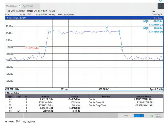
Band4-3MHz-16QAM-20385-15RB#0-PASS
