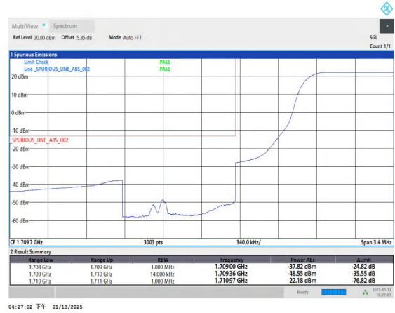
Band4_1.4MHz_QPSK_19957_1RB#5
