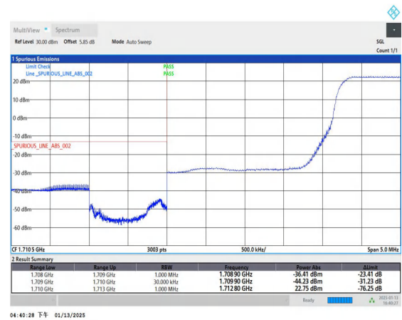
Band4_3MHz_16QAM_19965_1RB#14
