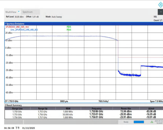
Band4_5MHz_16QAM_20375_25RB#0
