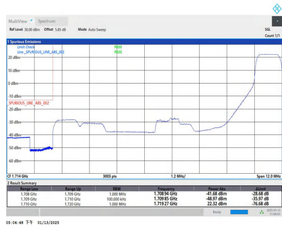
Band4_10MHz_QPSK_20000_1RB#49
