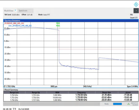
Band4_1.4MHz_QPSK_20393_6RB#0
