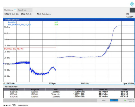
Band4_3MHz_QPSK_19965_1RB#14
