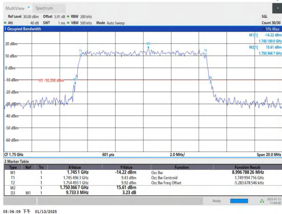
Band4-10MHz-QPSK-20350-50RB#0-PASS
