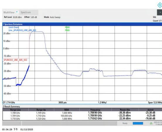
Band4_10MHz_QPSK_20000_1RB#0
