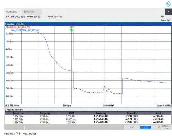
Band4_1.4MHz_16QAM_20393_1RB#0
