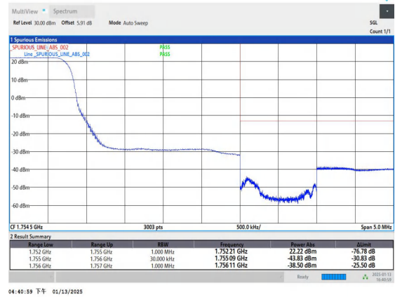
Band4_3MHz_QPSK_20385_1RB#0
