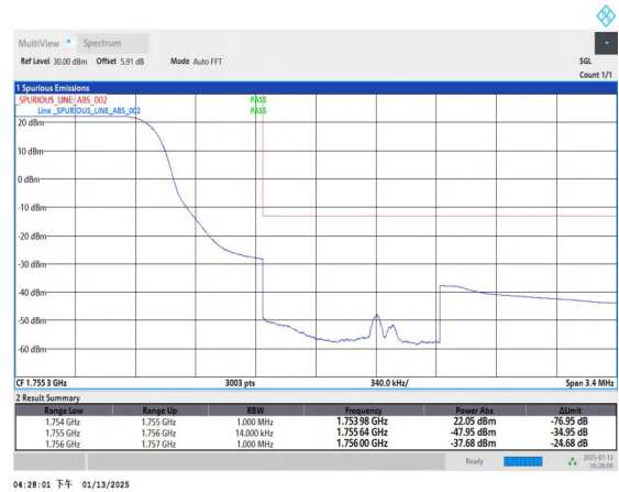
Band4_1.4MHz_QPSK_20393_1RB#0
