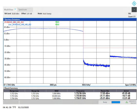
Band4_3MHz_QPSK_20385_15RB#0
