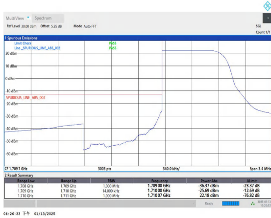
Band4_1.4MHz_QPSK_19957_1RB#0
