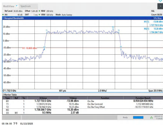
Band4-10MHz-16QAM-20175-50RB#0-PASS
