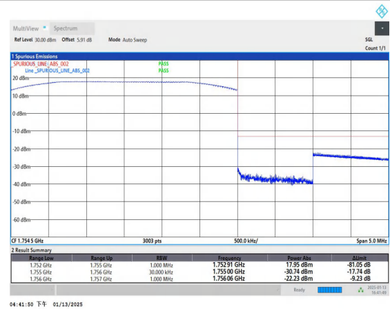
Band4_3MHz_16QAM_20385_15RB#0
