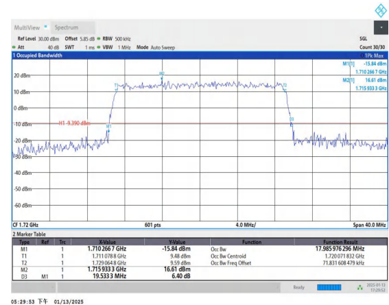
Band4-20MHz-16QAM-20050-100RB#0-PASS
