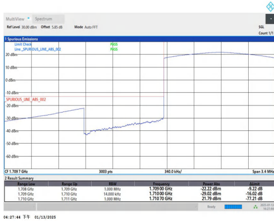
Band4_1.4MHz_16QAM_19957_6RB#0
