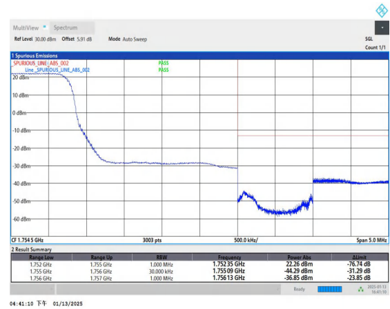
Band4_3MHz_16QAM_20385_1RB#0
