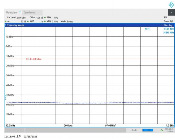
Band2_20MHz_16QAM_18700_1RB#0_30~1000_30~1000
