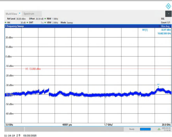
Band2_20MHz_16QAM_18700_1RB#0_3000~20000_3000~2000
