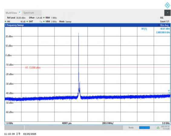
Band2_20MHz_QPSK_19100_1RB#0_1000~3000_1000~3000
