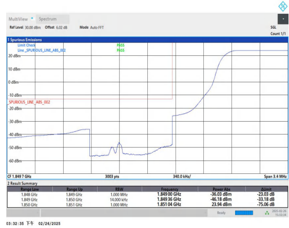
Band2_1.4MHz_QPSK_18607_1RB#5
