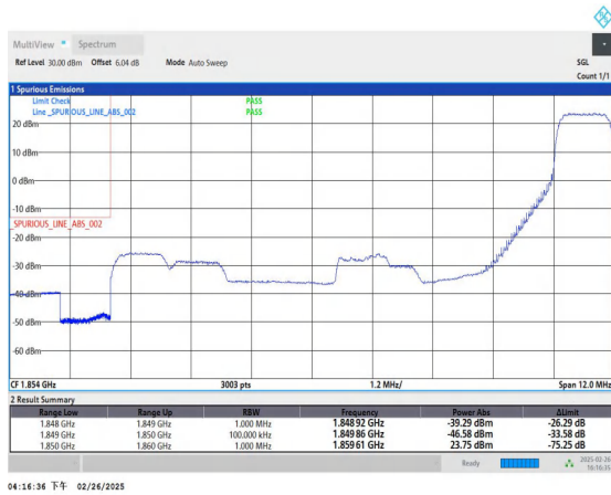
Band2_10MHz_16QAM_18650_1RB#49
