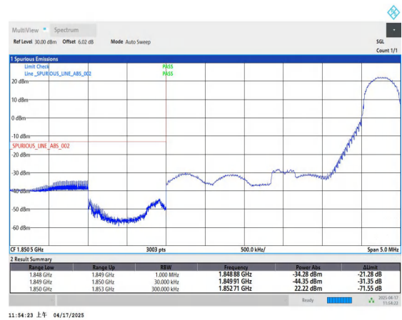
Band2_3MHz_16QAM_18615_1RB#14
