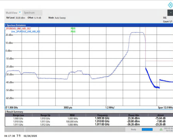
Band2_10MHz_16QAM_19150_1RB#0
