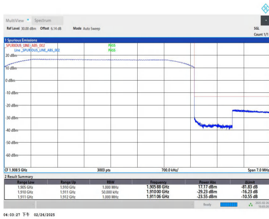
Band2_5MHz_QPSK_19175_25RB#0
