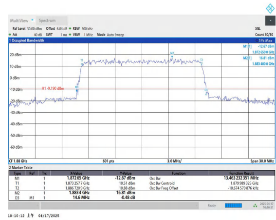
Band2-15MHz-QPSK-18900-75RB#0-PASS
