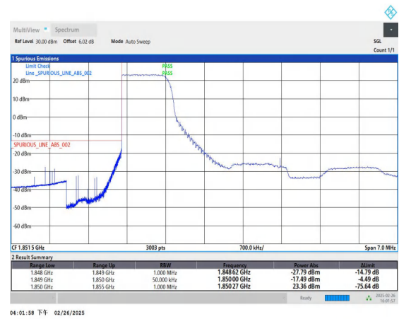
Band2_5MHz_16QAM_18625_1RB#0
