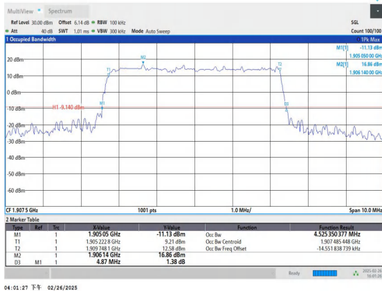
Band2-5MHz-QPSK-19175-25RB#0-PASS
