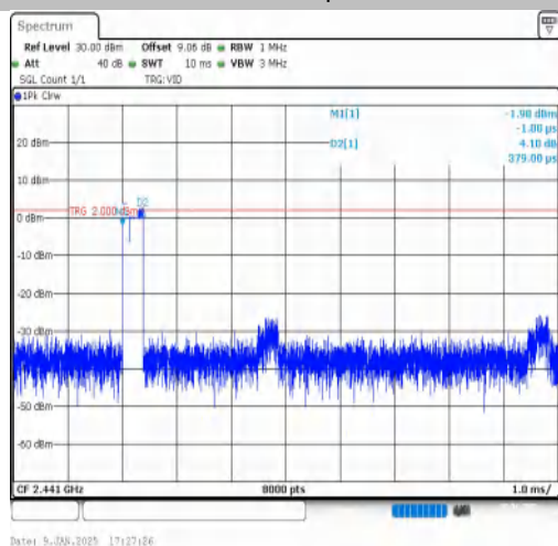
2DH3-Ant1-Hop-PASS
