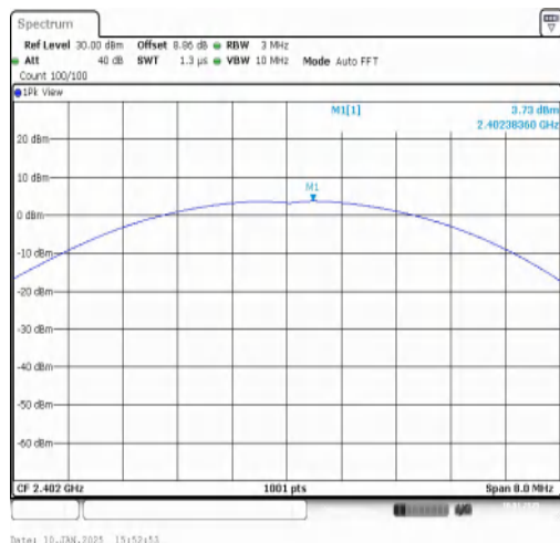
3DH5-Ant1-2402-PASS
