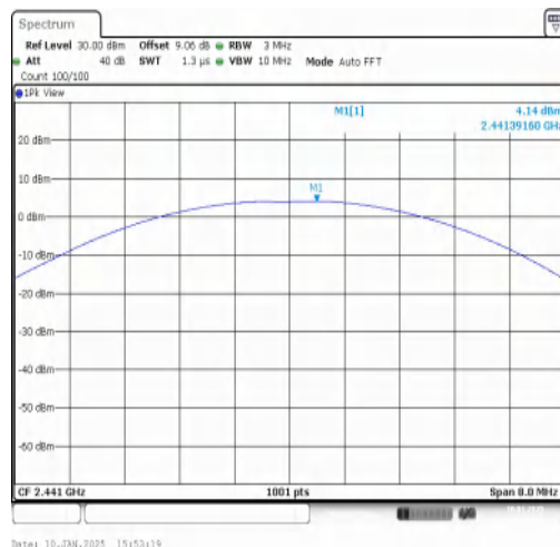
3DH5-Ant1-2441-PASS
