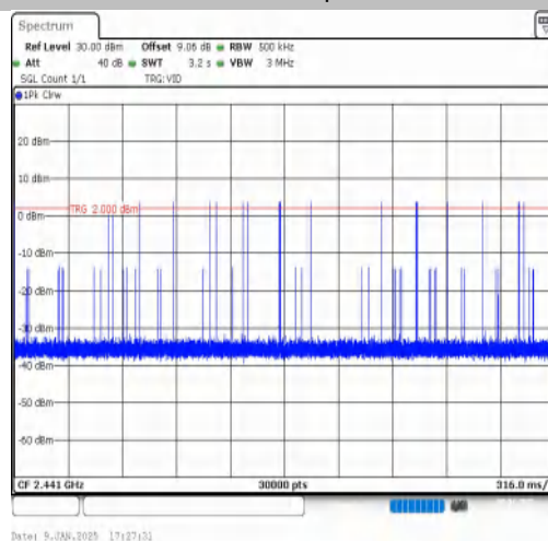
2DH3-Ant1-Hop-PASS
