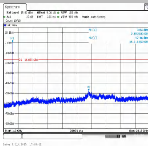
2DH5-Ant1-2480-1000~26500-PASS
