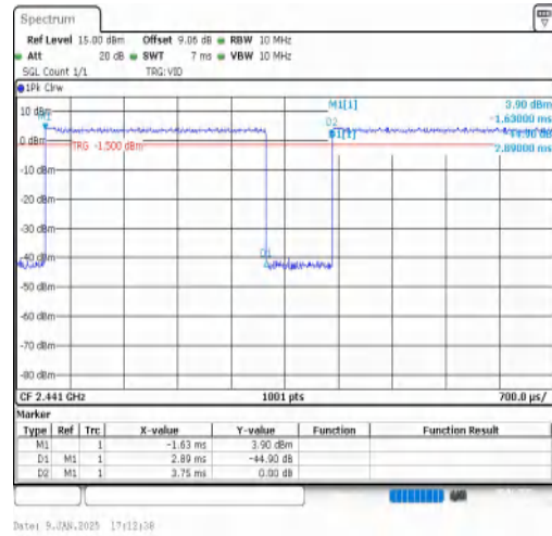
NTNV-3DH5-Ant1-2441
