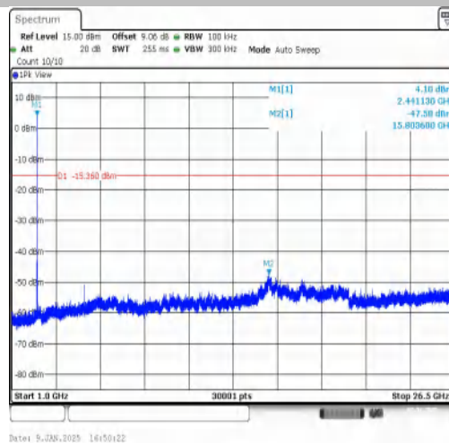
DH5-Ant1-2441-1000~26500-PASS
