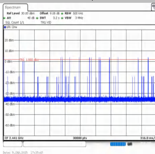
3DH3-Ant1-Hop-PASS
