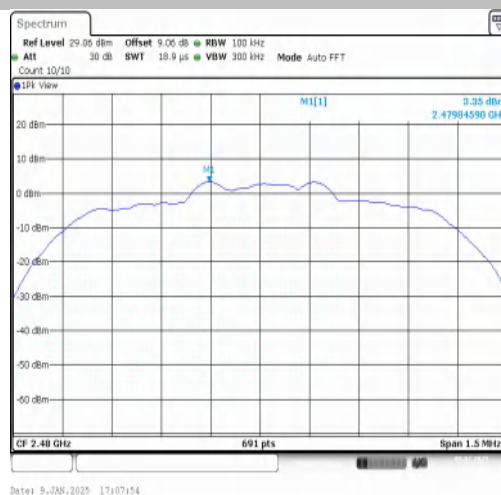
2DH5-Ant1-2480-0~Reference-PASS
