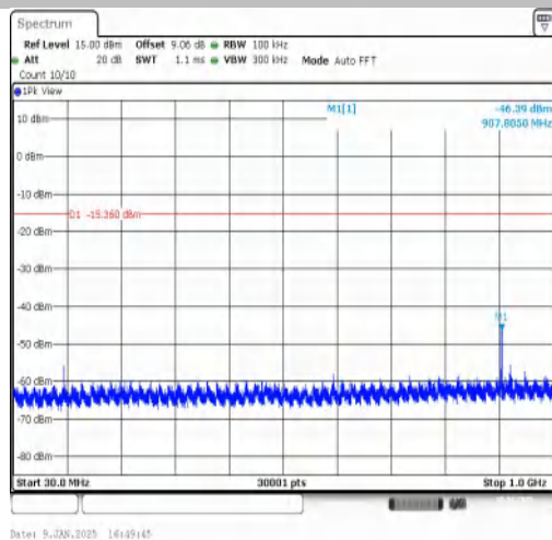
DH5-Ant1-2441-30~1000-PASS
