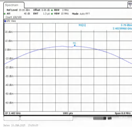
2DH5-Ant1-2402-PASS
