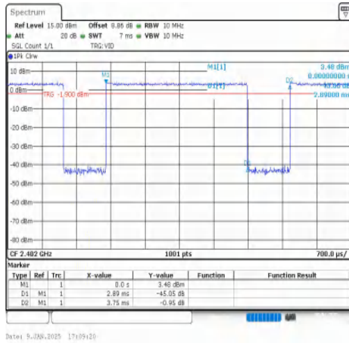
NTNV-3DH5-Ant1-2402
