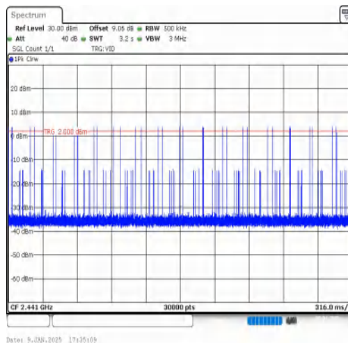
3DH1-Ant1-Hop-PASS
