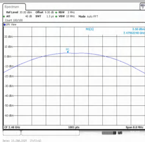
3DH5-Ant1-2480-PASS
