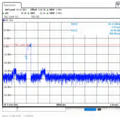
2DH1-Ant1-Hop-PASS
