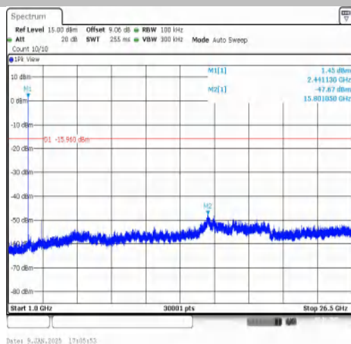
2DH5-Ant1-2441-1000~26500-PASS
