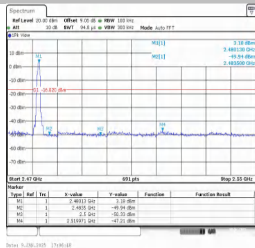
2DH5-Ant1-2480-PASS
