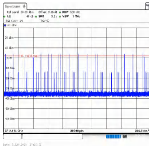
2DH1-Ant1-Hop-PASS
