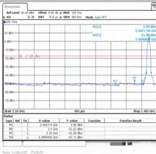
2DH5-Ant1-2402-PASS
