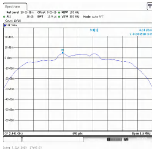
2DH5-Ant1-2441-0~Reference-PASS
