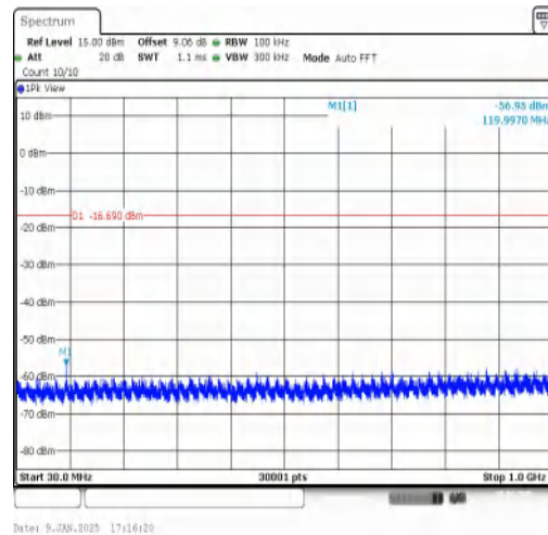
3DH5-Ant1-2480-30~1000-PASS
