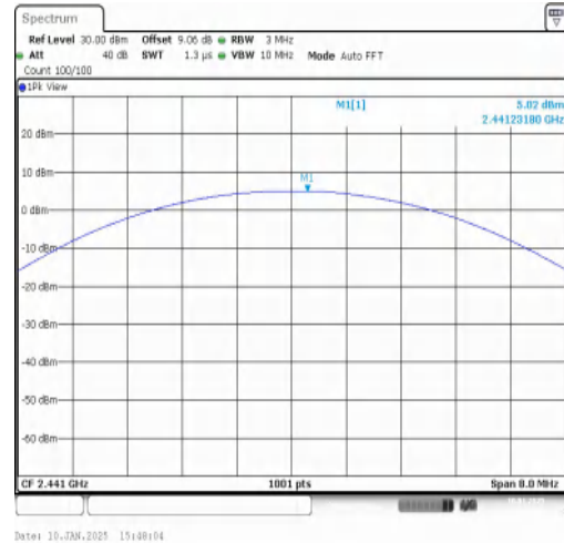
DH5-Ant1-2441-PASS
