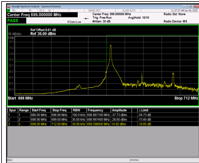
Band12-10MHz-64QAM-23060-50RB#0
