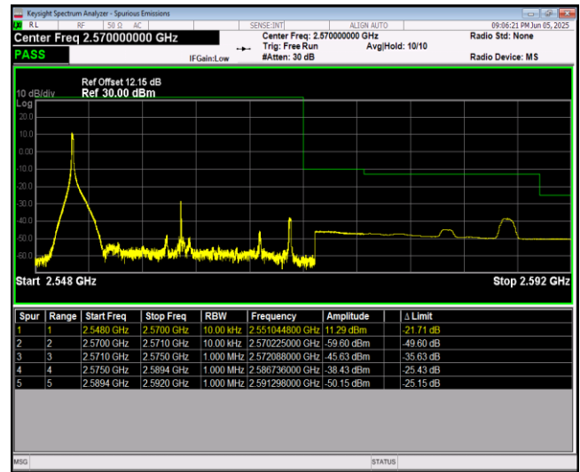
Band7-20MHz-64QAM-21350-100RB#0
