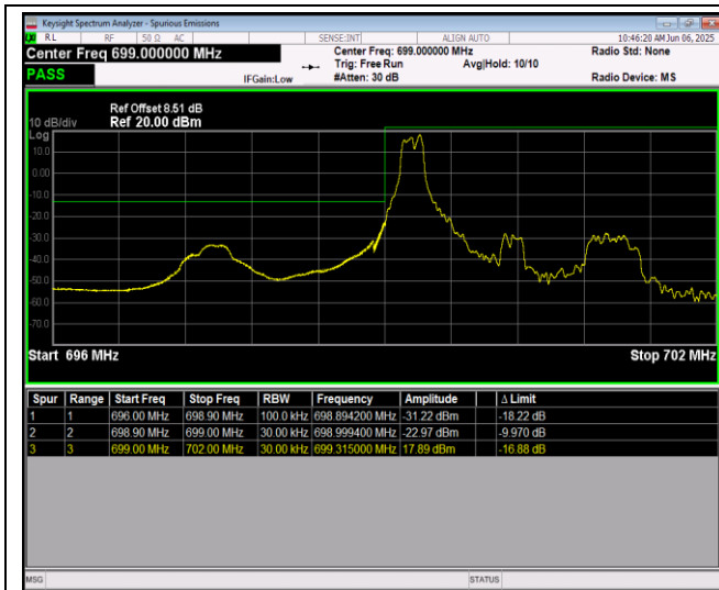
Band12-1.4MHz-QPSK-23017-6RB#0
