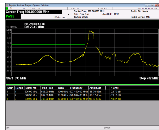
Band12-1.4MHz-64QAM-23017-6RB#0
