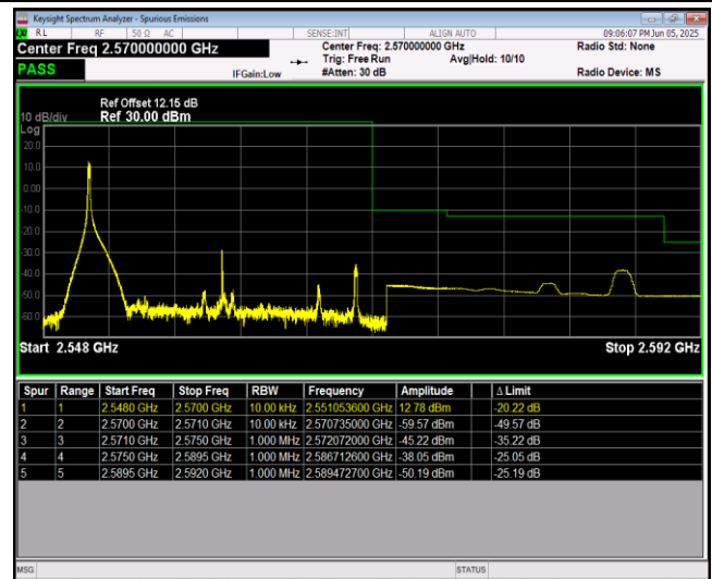
Band7-20MHz-16QAM-21350-100RB#0
