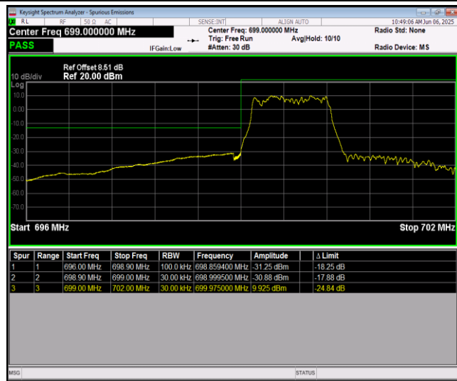
Band12-1.4MHz-QPSK-23173-1RB#5
