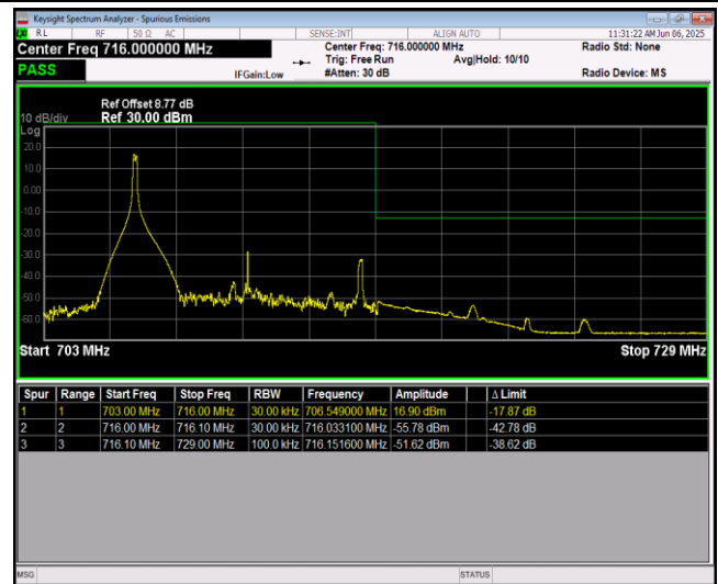
Band12-10MHz-16QAM-23130-50RB#0
