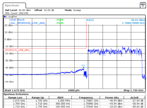
n66_25MHz_15kHz_1722.5MHz_DFT-s-OFDM QPSK_RB128@0
