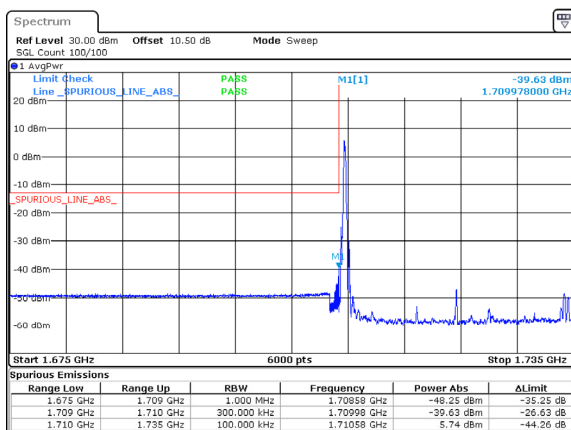
n66_25MHz_15kHz_1722.5MHz_DFT-s-OFDM QPSK_RB1@0
