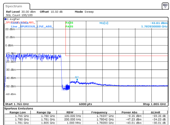
n66_15MHz_15kHz_1772.5MHz_DFT-s-OFDM QPSK_RB75@0
