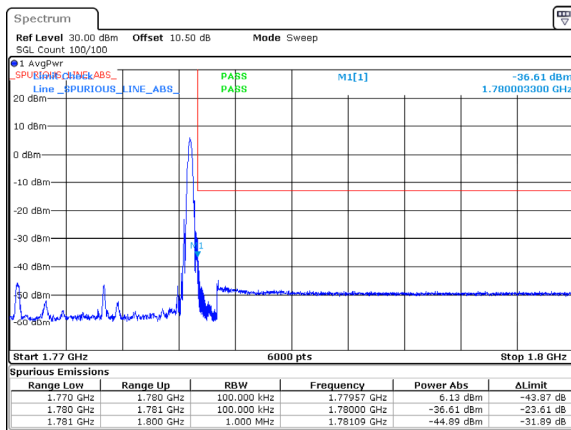
n66_10MHz_15kHz_1775MHz_DFT-s-OFDM QPSK_RB1@51
