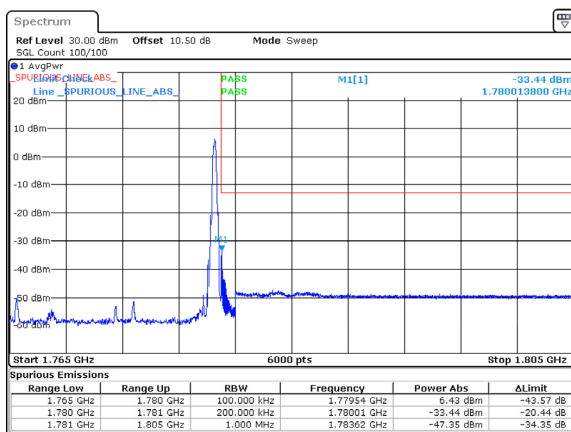
n66_15MHz_15kHz_1772.5MHz_DFT-s-OFDM QPSK_RB1@78
