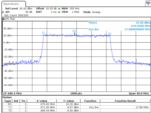
Occupied Bandwidth
