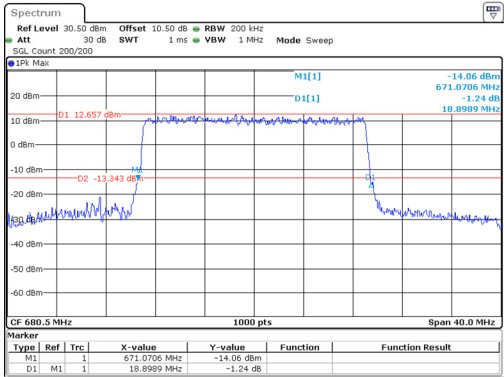
26dB Bandwidth
