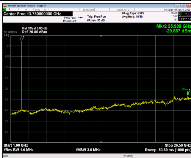
Band41-20MHz-16QAM-40620-1RB#0-Range2:1000~26500MHz
