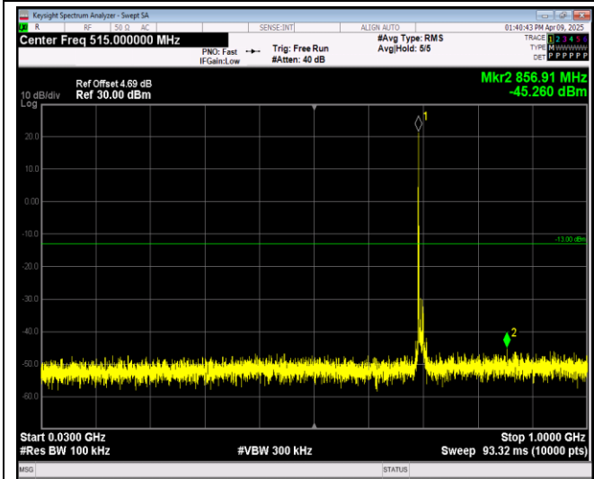
Band12-10MHz-16QAM-23095-1RB#0-Range1:30~-1000MHz
