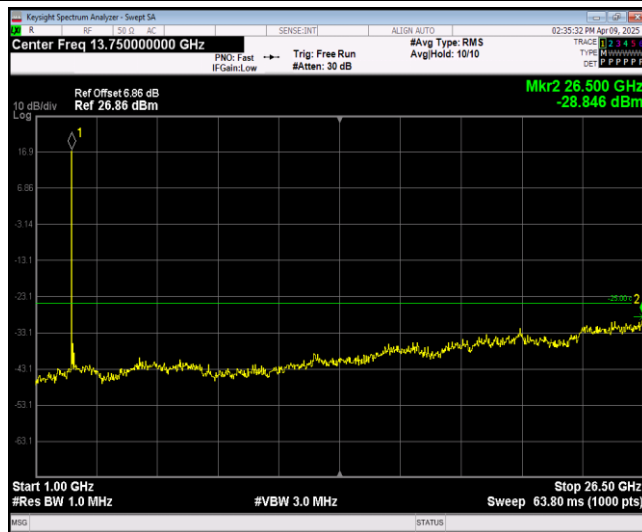
Band41-5MHz-64QAM-40620-1RB#0-Range2:1000~26500MHz
