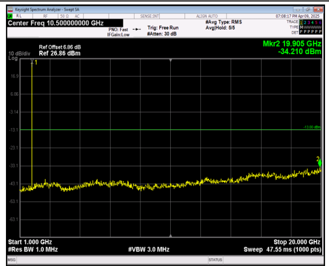
Band66-1.4MHz-QPSK-132665-1RB#0-Range2:1000~20000MHz
