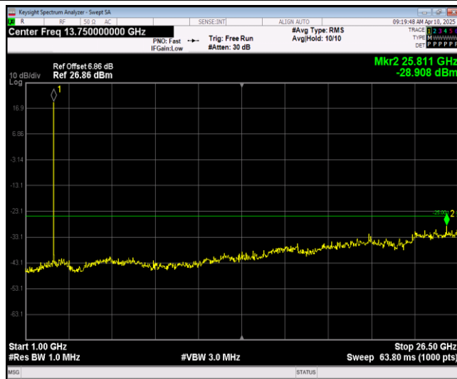
Band41-20MHz-16QAM-39750-1RB#0-Range2:1000~26500MHz
