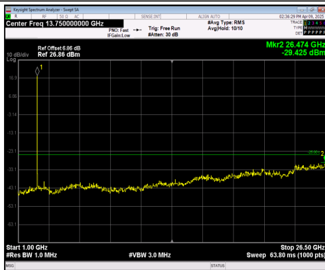
Band41-5MHz-64QAM-41565-1RB#0-Range2:1000~26500MHz
