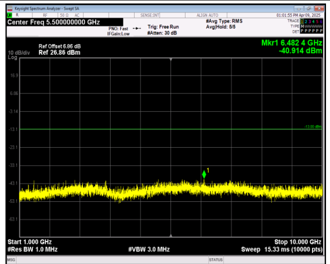
Band12-1.4MHz-64QAM-23017-1RB#0-Range2:1000 ~10000MHz
