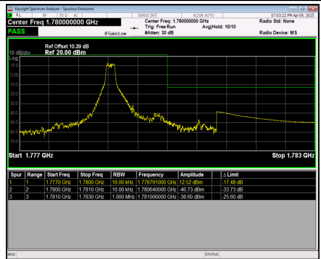
Band66-1.4MHz-16QAM-132665-6RB#0
