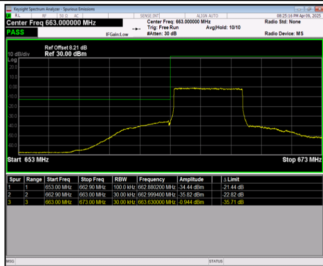
Band71-5MHz-16QAM-133447-1RB#24
