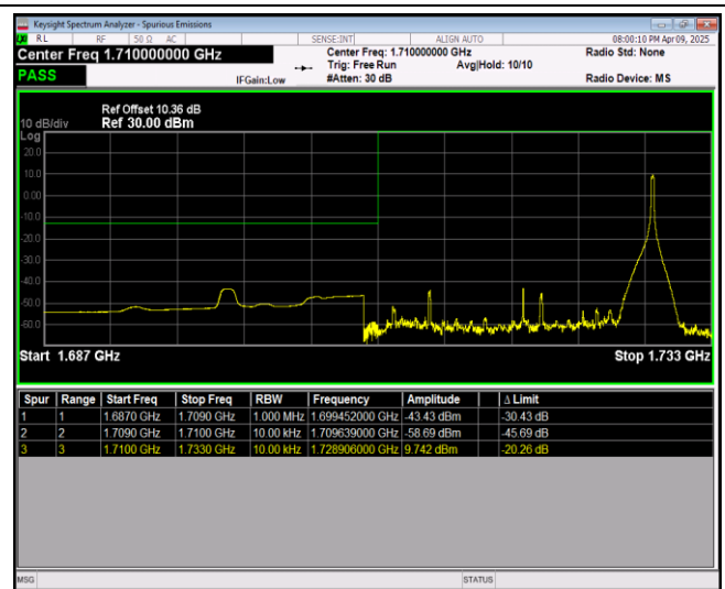
Band66-20MHz-64QAM-132572-1RB#0
