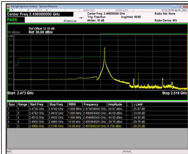
Band41-20MHz-16QAM-39750-100RB#0
