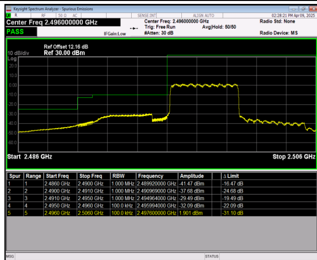
Band41-5MHz-QPSK-41565-1RB#24
