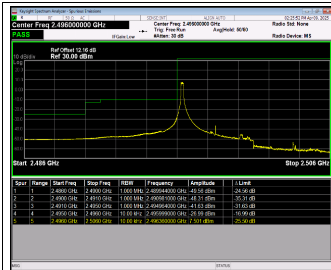
Band41-5MHz-16QAM-39675-25RB#0
