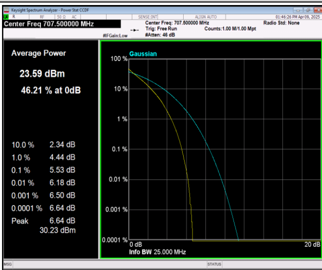
Band12-10MHz-64QAM-23095-50RB#0
