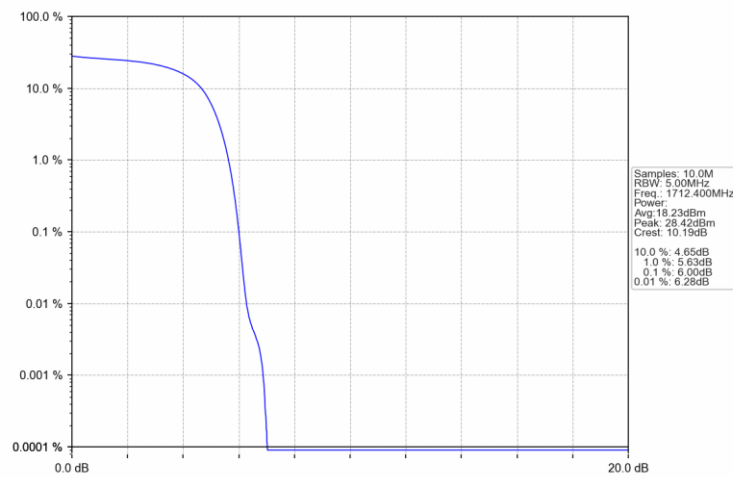
Band4_HSDPA_LCH_1712.4MHz_Subtest 1_NTNV
