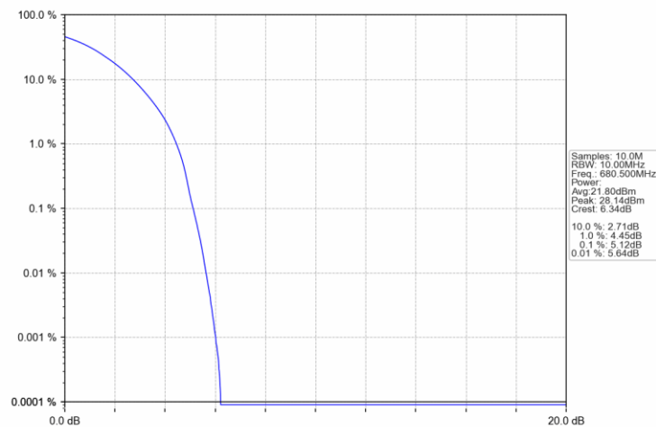
Band71_15MHz_QPSK_MCH_680.5MHz_RB_75_0_NTNV
