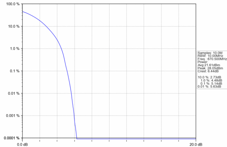
Band71_15MHz_QPSK_LCH_670.5MHz_RB_75_0_NTNV
