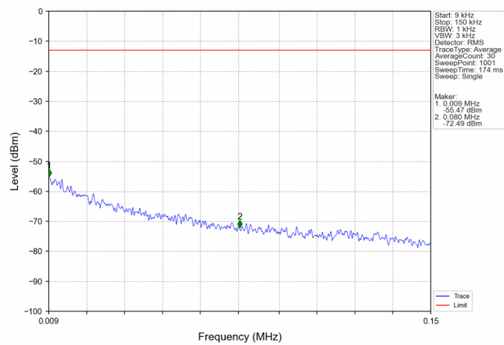
Band5_5MHz_QPSK_LCH_826.5MHz_RB_1_0_NTNV
