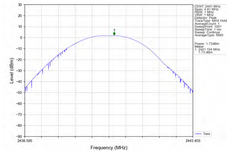
GFSK_DH5_MCH_2441MHz_Ant1_NTNV
