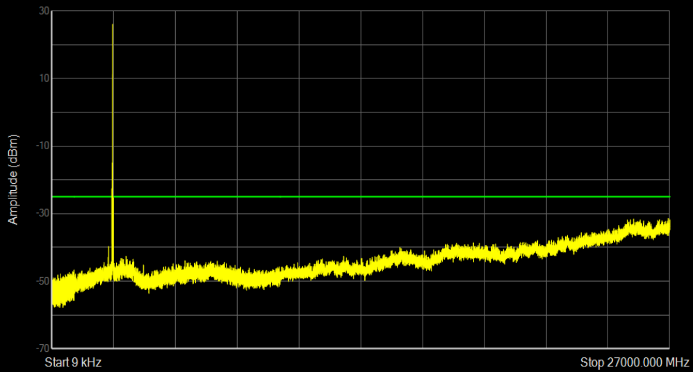
Band41 QPSK BW=15MHz Channel=41515 RB Size=1 Position=#0
