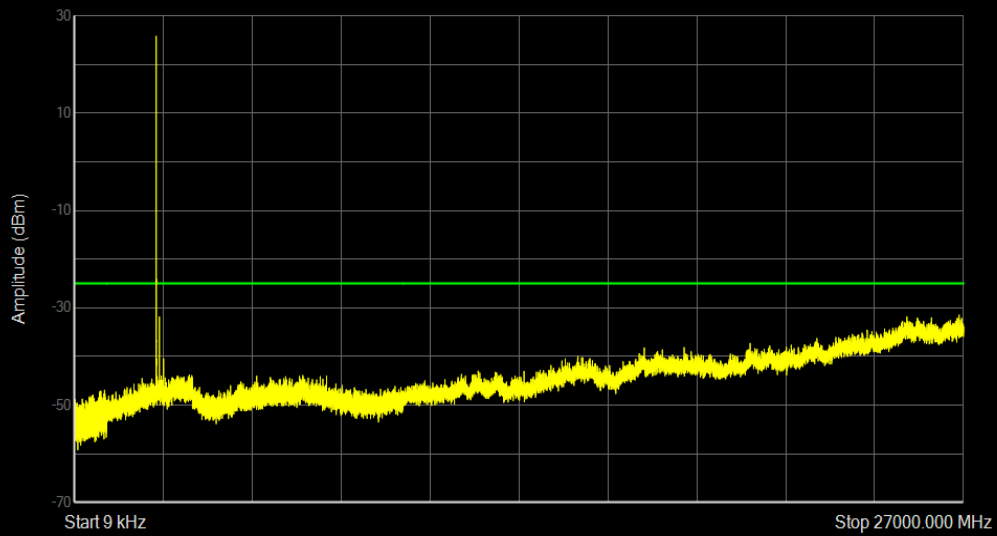
Band41 QPSK BW=5MHz Channel=39675 RB Size=1 Position=#0
