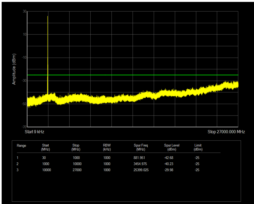
Band41(2565-2645) 16QAM BW=15MHz Channel=41065 RB Size=75 Position=#0
