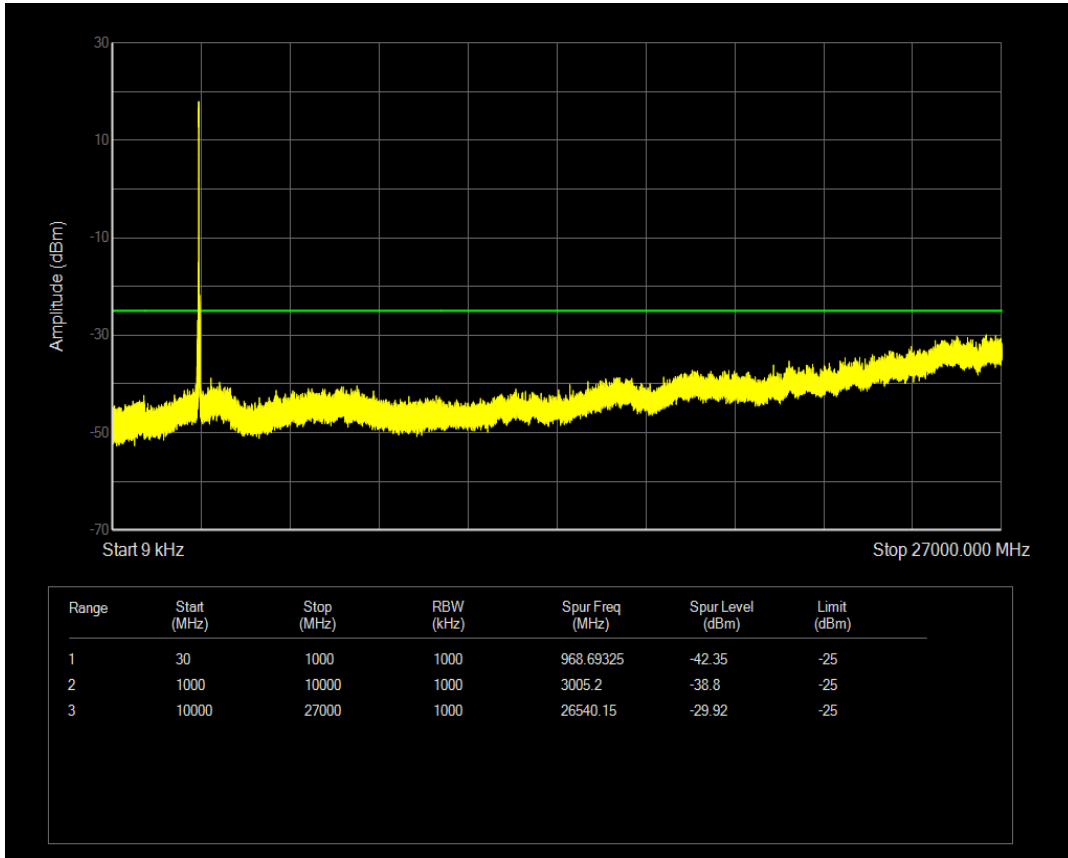
Band41(2565-2645) QPSK BW=20MHz Channel=40440 RB Size=1 Position=#0
