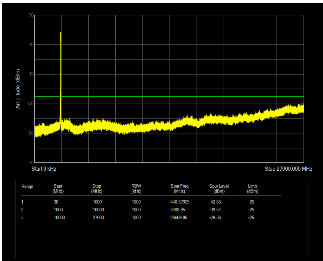
Band41(2565-2645) QPSK BW=15MHz Channel=41065 RB Size=1 Position=#0
