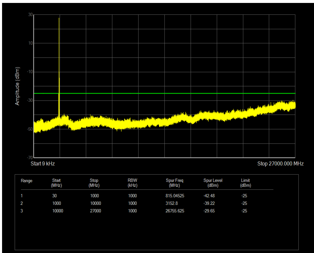
Band41(2565-2645) 16QAM BW=20MHz Channel=41040 RB Size=100 Position=#0
