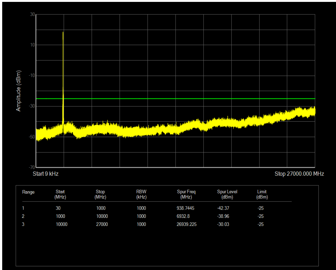
Band41(2565-2645) 16QAM BW=15MHz Channel=41065 RB Size=1 Position=#0
