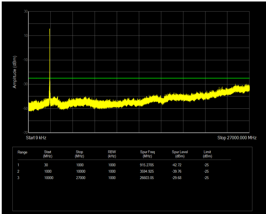
Band41(2565-2645) QPSK BW=20MHz Channel=41040 RB Size=1 Position=#0
