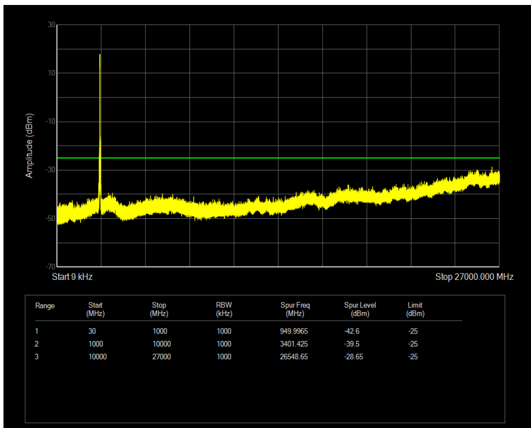
Band41(2565-2645) 16QAM BW=20MHz Channel=41040 RB Size=1 Position=#0
