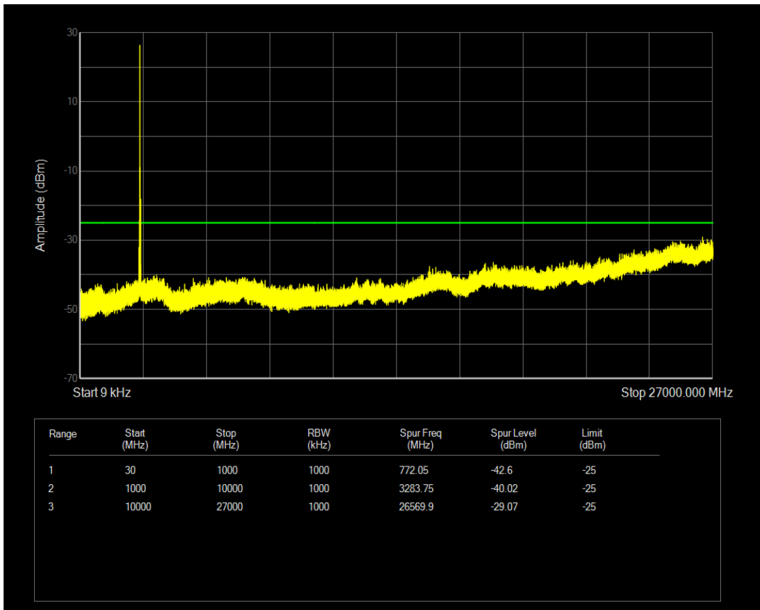
Band41(2565-2645) QPSK BW=20MHz Channel=40440 RB Size=100 Position=#0
