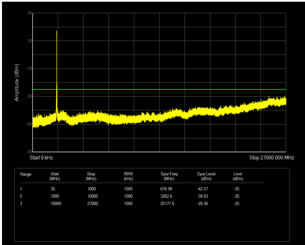
Band41(2565-2645) 16QAM BW=20MHz Channel=40440 RB Size=1 Position=#0
