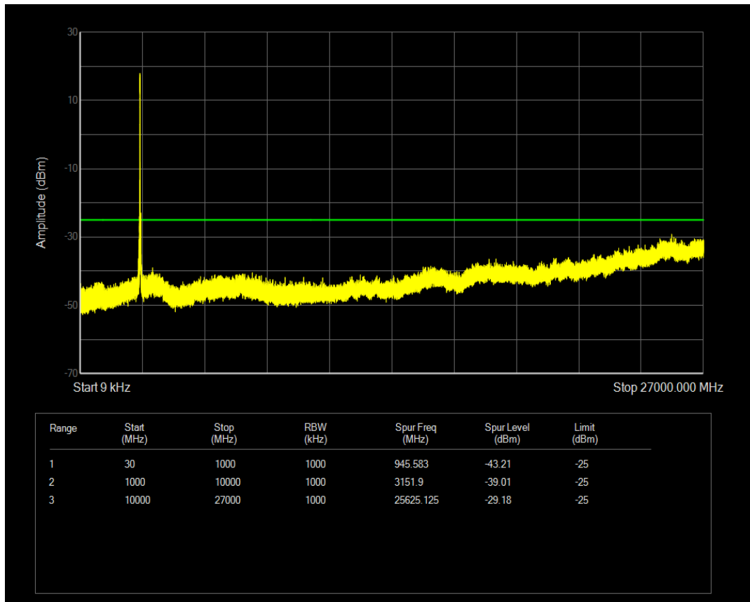
Band41(2565-2645) 16QAM BW=20MHz Channel=40740 RB Size=1 Position=#0
