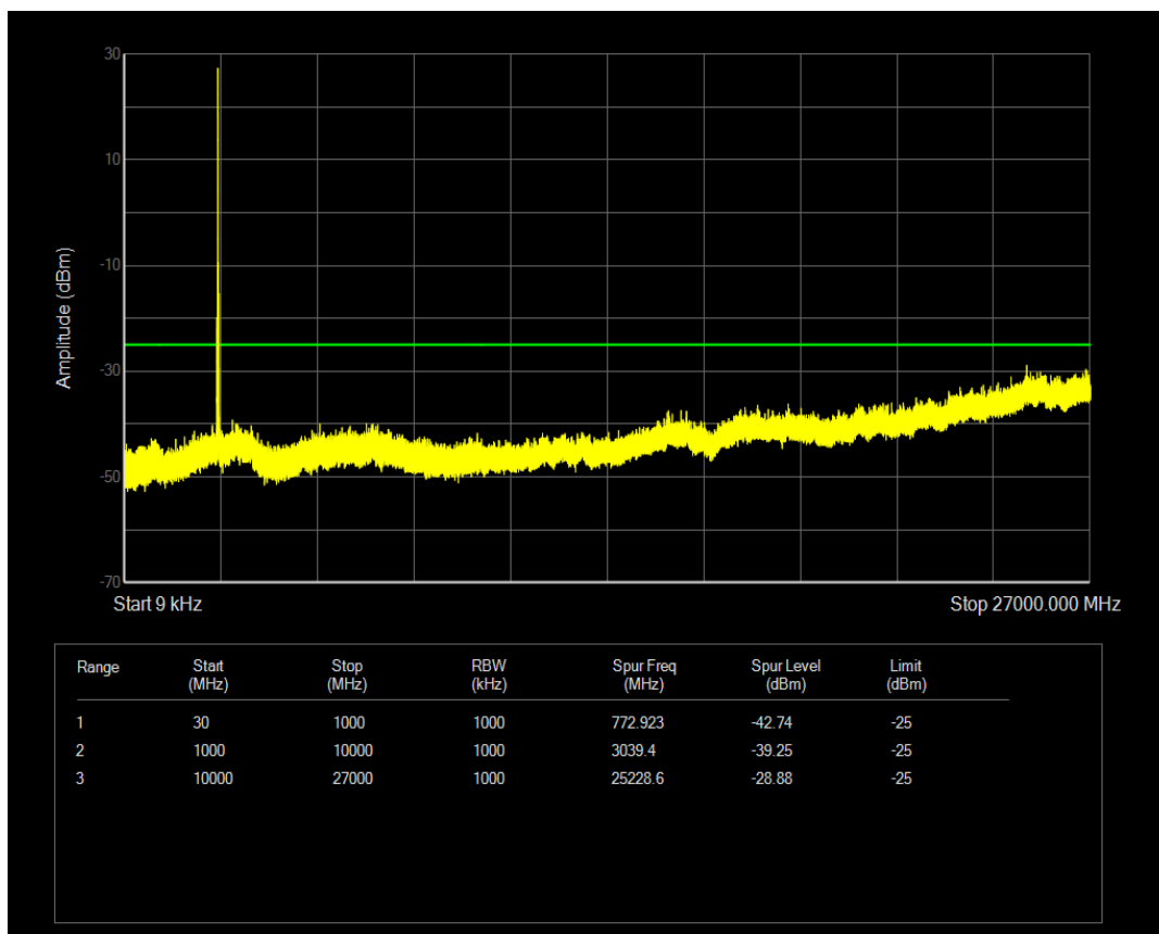
Band41(2565-2645) QPSK BW=15MHz Channel=41065 RB Size=75 Position=#0
