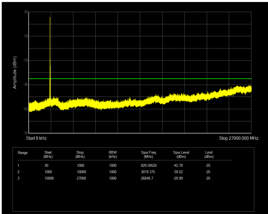
Band41(2565-2645) QPSK BW=20MHz Channel=40740 RB Size=100 Position=#0
