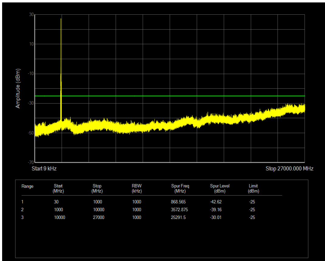
Band41(2565-2645) QPSK BW=20MHz Channel=41040 RB Size=100 Position=#0
