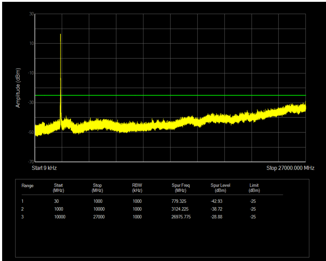
Band41(2565-2645) QPSK BW=20MHz Channel=40740 RB Size=1 Position=#0
