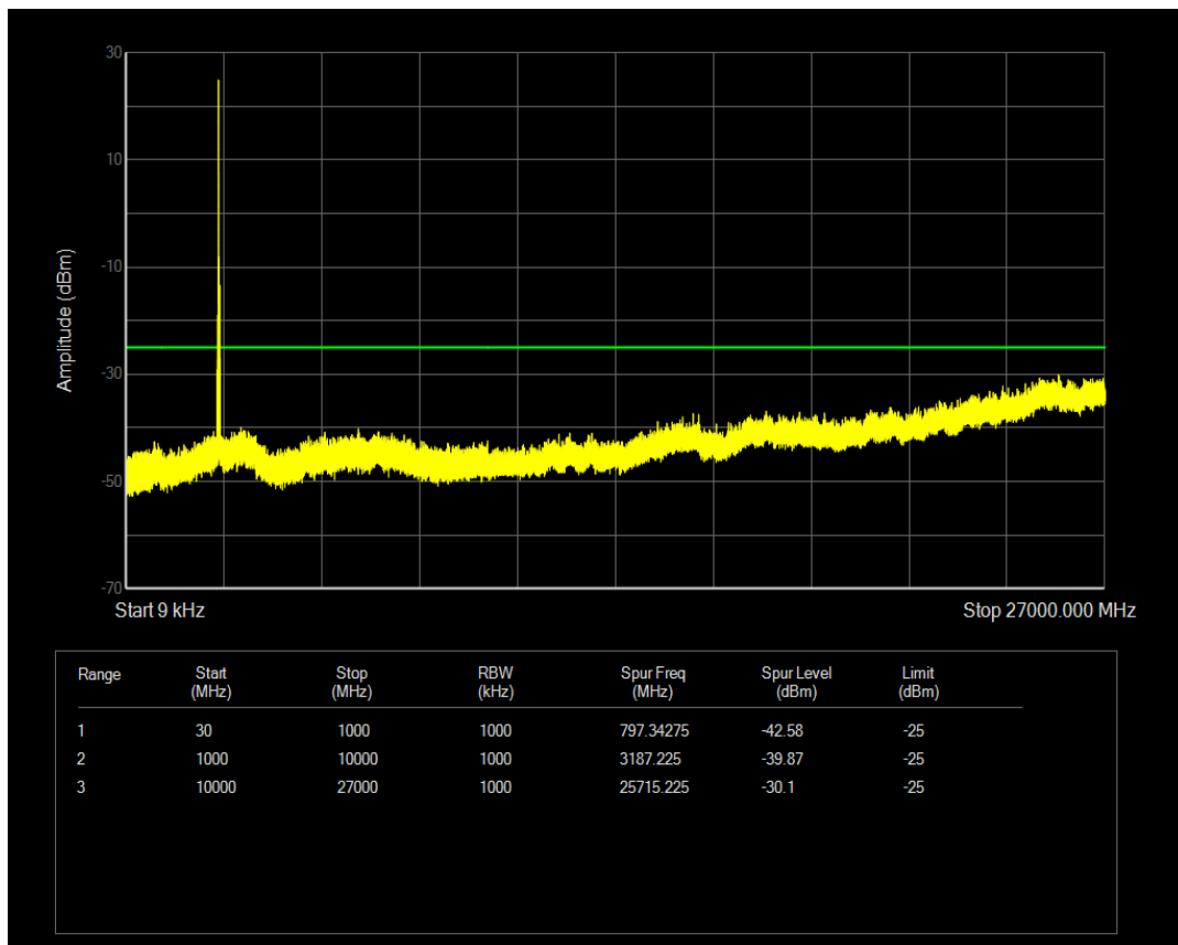
Band41(2565-2645) 16QAM BW=20MHz Channel=40440 RB Size=100 Position=#0
