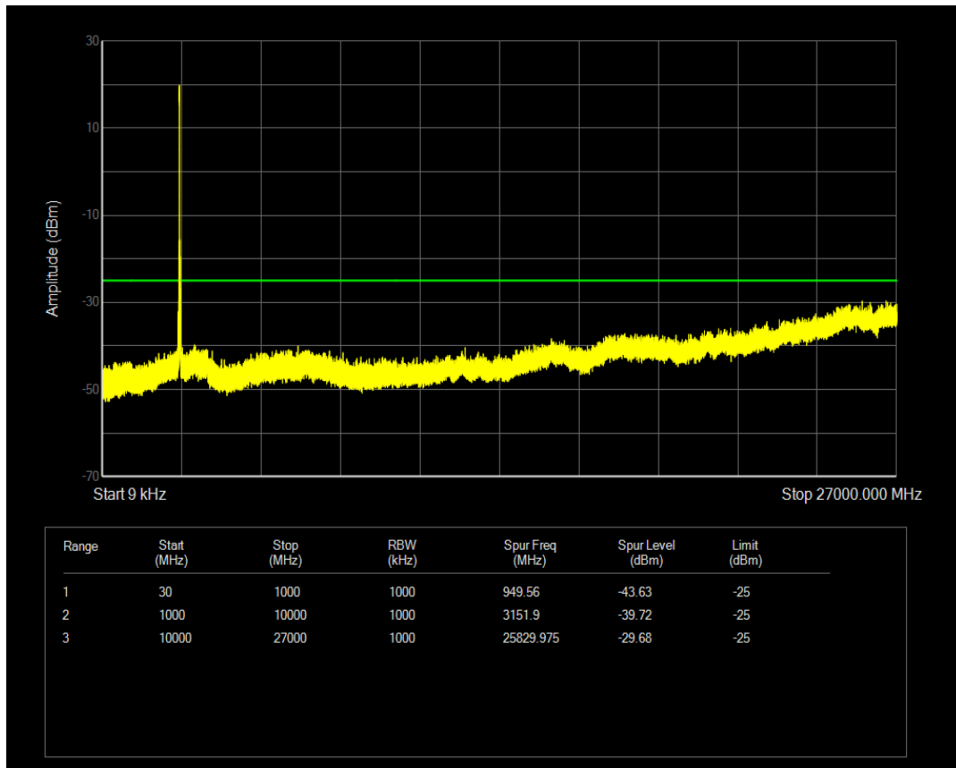
Band41(2565-2645) 16QAM BW=10MHz Channel=41090 RB Size=1 Position=#0
