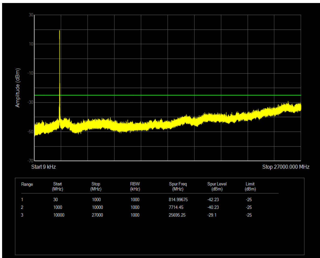
Band41(2565-2645) 16QAM BW=15MHz Channel=40415 RB Size=75 Position=#0
