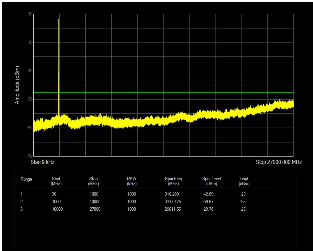
Band41(2565-2645) 16QAM BW=10MHz Channel=40740 RB Size=50 Position=#0
