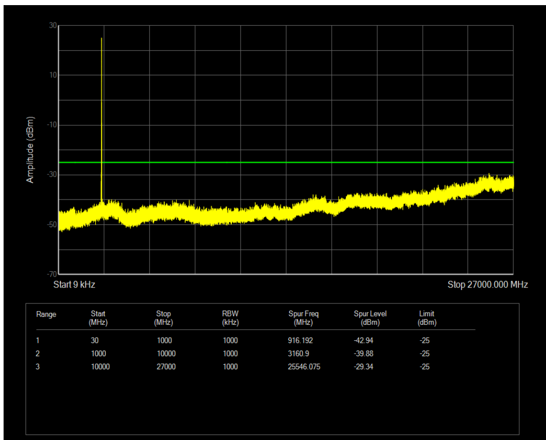
Band41(2565-2645) 16QAM BW=10MHz Channel=40390 RB Size=50 Position=#0
