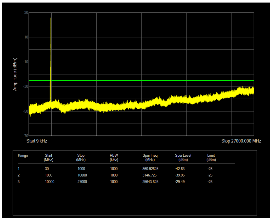
Band41(2565-2645) QPSK BW=15MHz Channel=40415 RB Size=75 Position=#0
