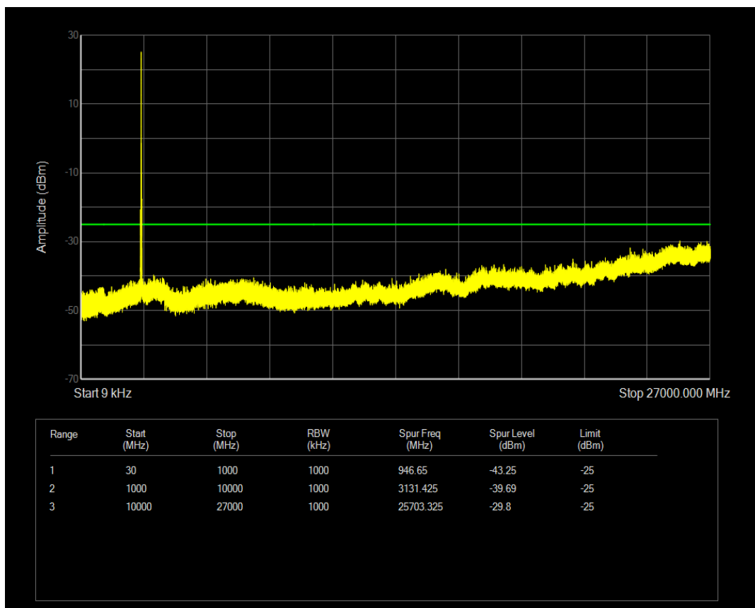
Band41(2565-2645) QPSK BW=15MHz Channel=40740 RB Size=75 Position=#0
