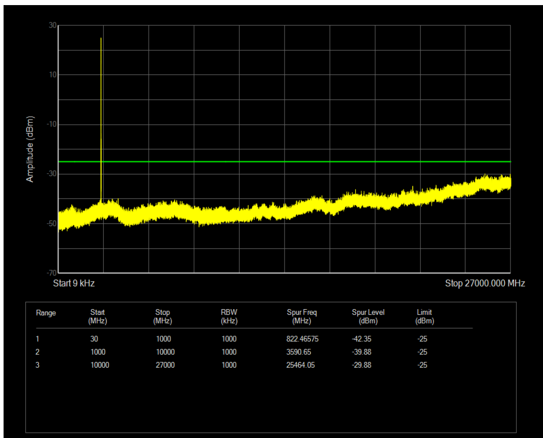
Band41(2565-2645) 16QAM BW=5MHz Channel=40365 RB Size=25 Position=#0
