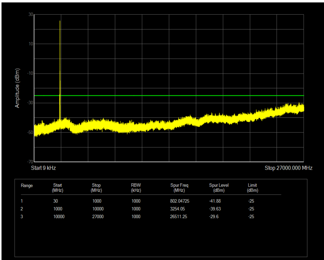
Band41(2565-2645) 16QAM BW=15MHz Channel=40740 RB Size=75 Position=#0
