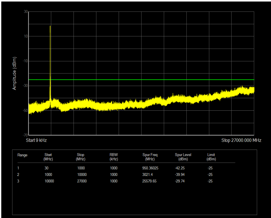
Band41(2565-2645) 16QAM BW=15MHz Channel=40740 RB Size=1 Position=#0
