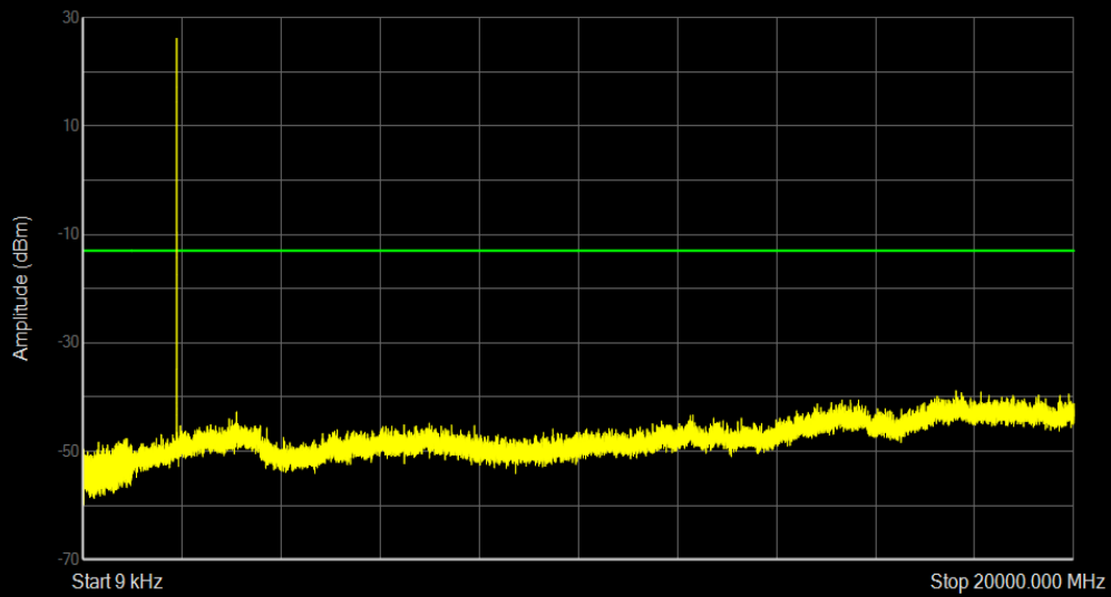
Band2 16QAM BW=1.4MHz Channel=19193 RB Size=1 Position=#0
