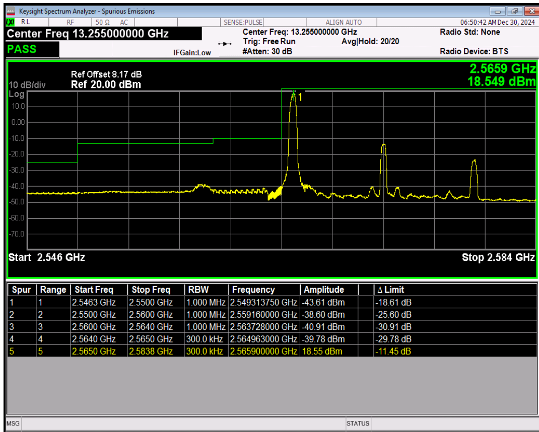
Band41(2565-2645) QPSK BW=15MHz Channel=40415 RB Size=1 Position=#Max
