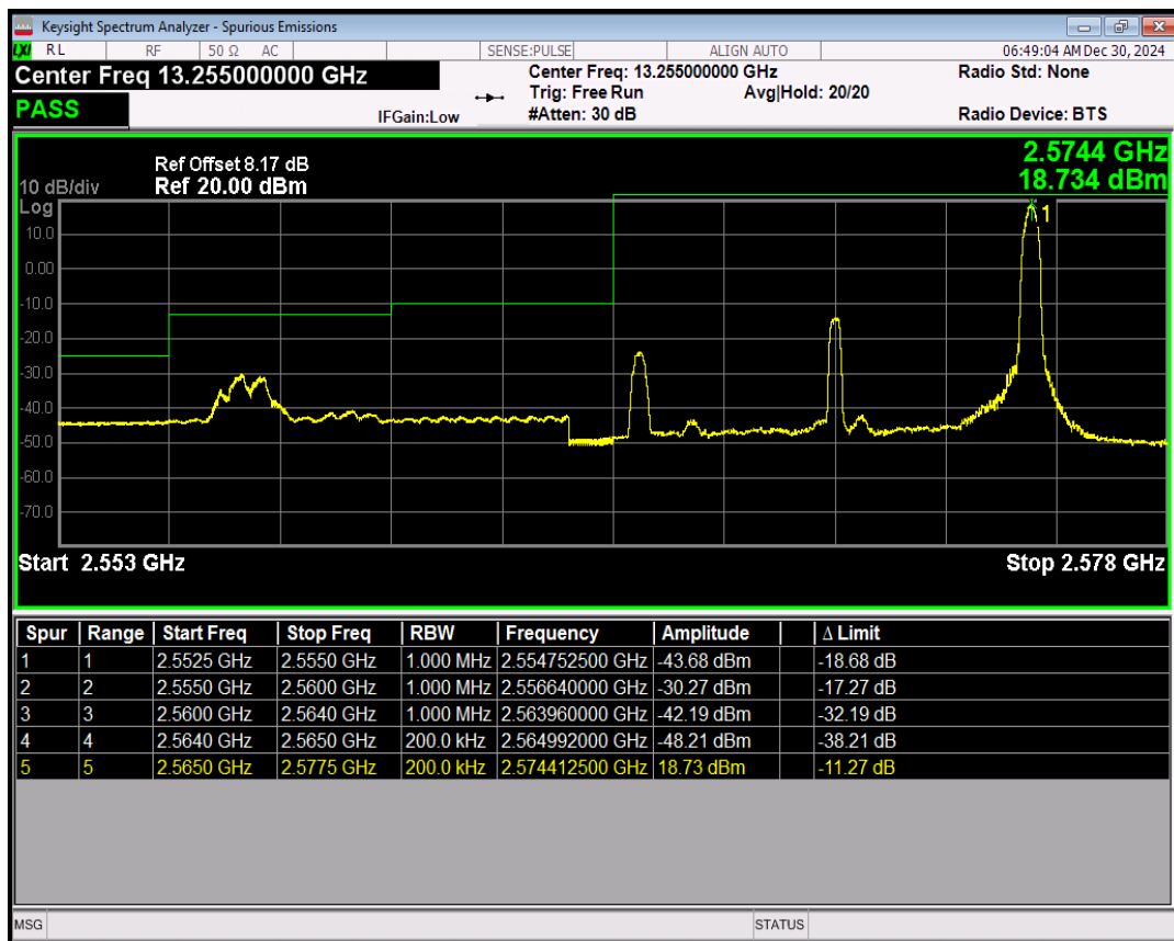
Band41(2565-2645) QPSK BW=10MHz Channel=40390 RB Size=50 Position=#0
