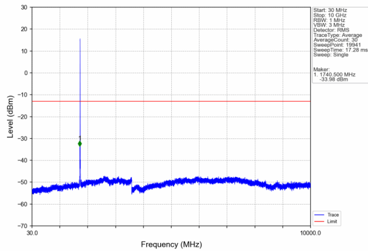
Band4_HSUPA_HCH_1752.6MHz_Subtest 1_NTNV
