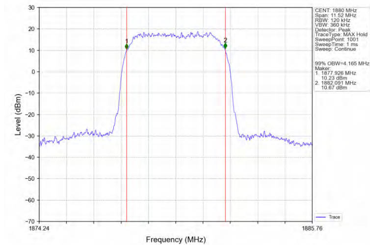
Band2_RMC_MCH_1880MHz_12.2kbps_RMC_NTNV
