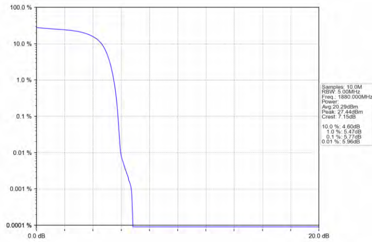
Band2_HSDPA_MCH_1880MHz_Subtest 1_NTNV
