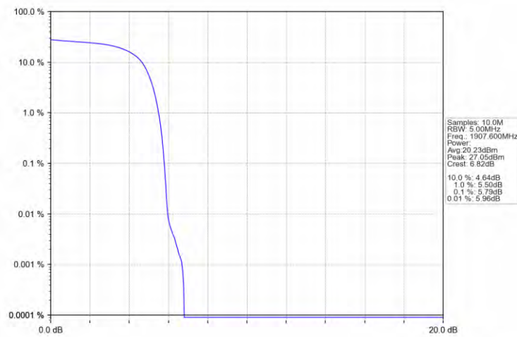
Band2_HSDPA_HCH_1907.6MHz_Subtest 1_NTNV
