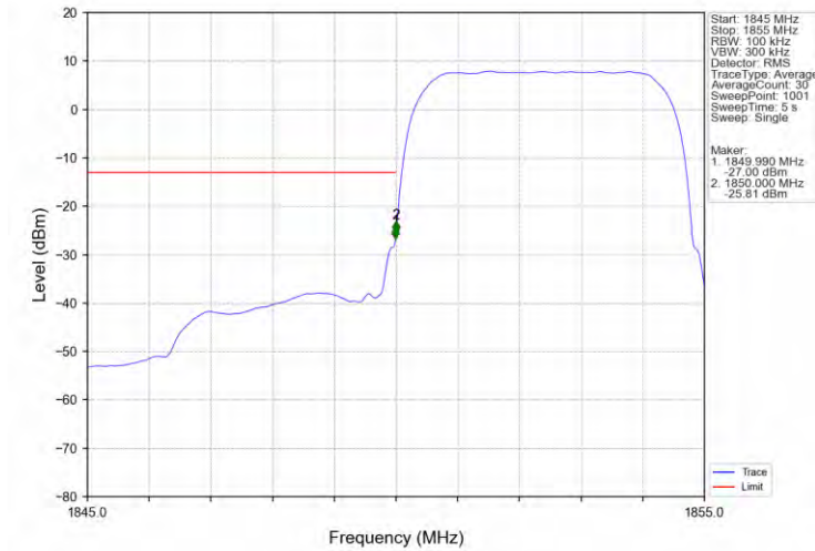
Band2 RMC LCH 1852.4MHz 12.2kbps RMC NTN
