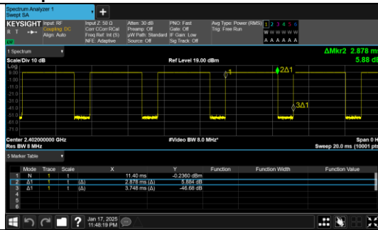
GFSK(DH5)_Channel 0
