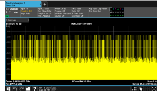
Number of Pulses in 31.6 seconds GFSK_DH3
