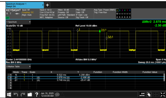
GFSK(DH5)_Channel 39
