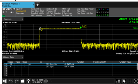
Pulse Width GFSK_DH1
