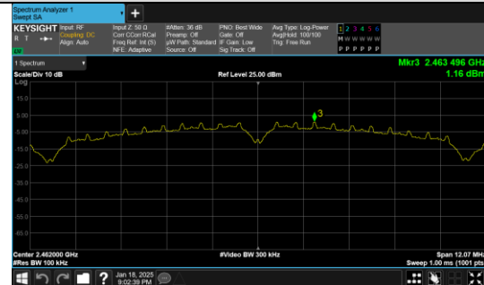
In-Band Reference Level IEEE 802.11b Channel 11 20MHz Antenna 0
