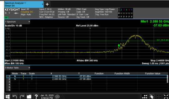
Out Of Band Emission IEEE 802.11b Channel 1 20MHz Antenna 0
