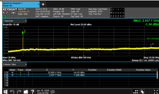
30.0 MHz - 25000.0 MHz IEEE 802.11b Channel 6 20MHz Antenna 0
