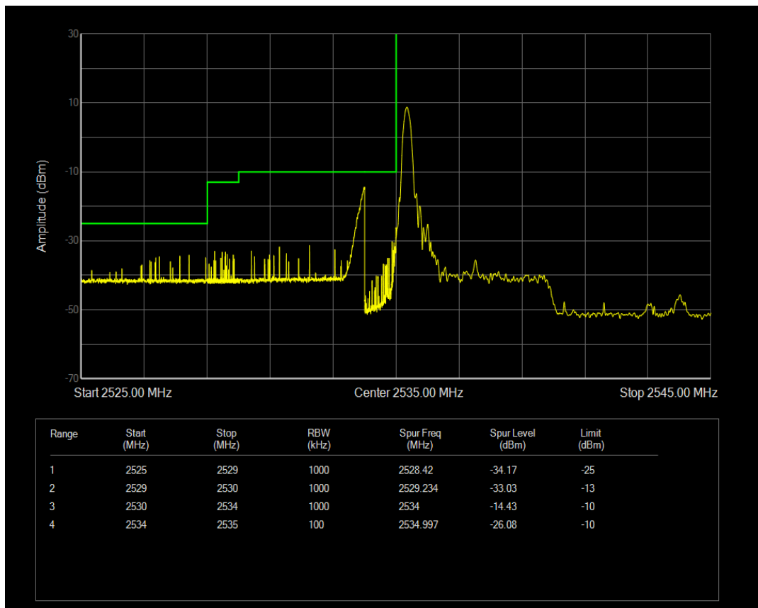
Band41(2535-2655) 16QAM BW=5MHz Channel=40065 RB Size=1 Position=#Max
