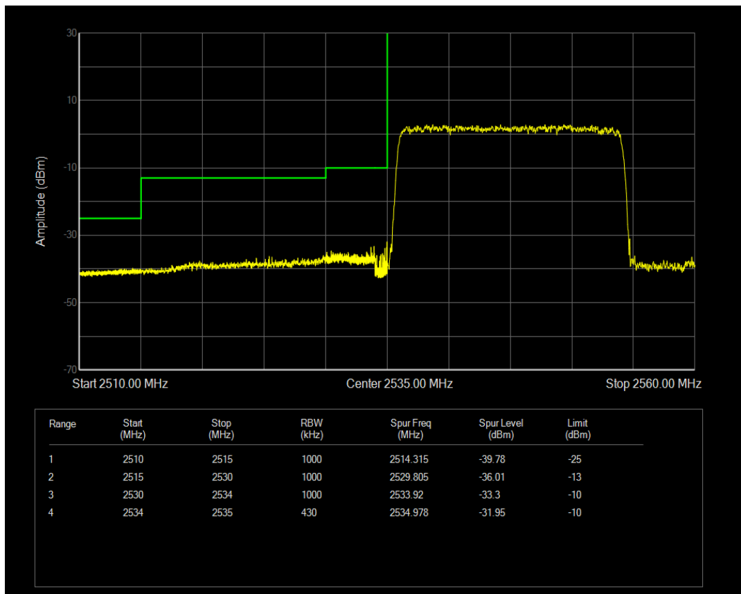
Band41(2535-2655) 16QAM BW=20MHz Channel=40140 RB Size=1 Position=#Max
