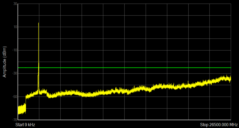
Band41 16QAM BW=20MHz Channel=40620 RB Size=100 Position=#0
