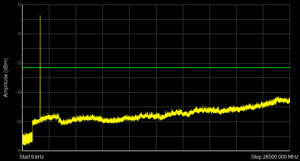
Band66 16QAM BW=5MHz Channel=132647 RB Size=25 Position=#0
