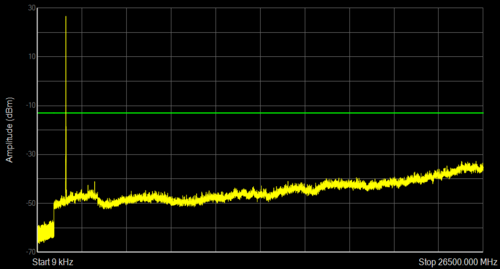
Band66 QPSK BW=10MHz Channel=132022 RB Size=1 Position=#0
