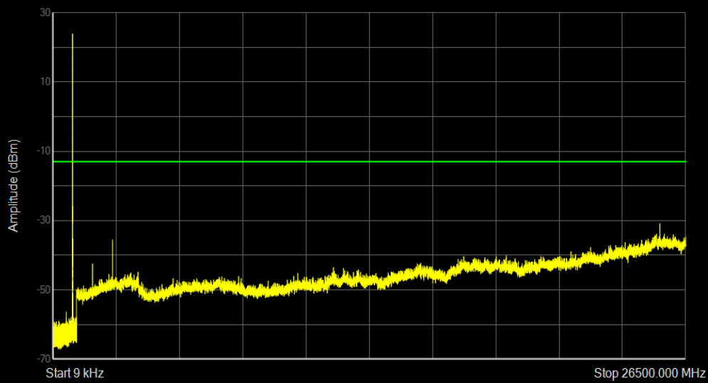
Band5 16QAM BW=1.4MHz Channel=20525 RB Size=1 Position=#0
