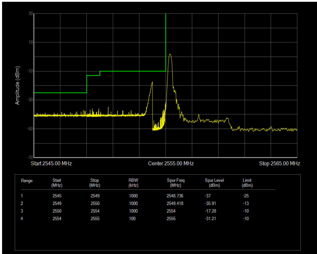
Band41(2555-2655) QAM16 BW=5MHz Channel=40265 RB Size=1 Position=#Max
