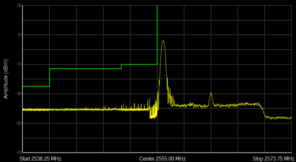
Band41(2555-2655) QPSK BW=15MHz Channel=40315 RB Size=1 Position=#0
