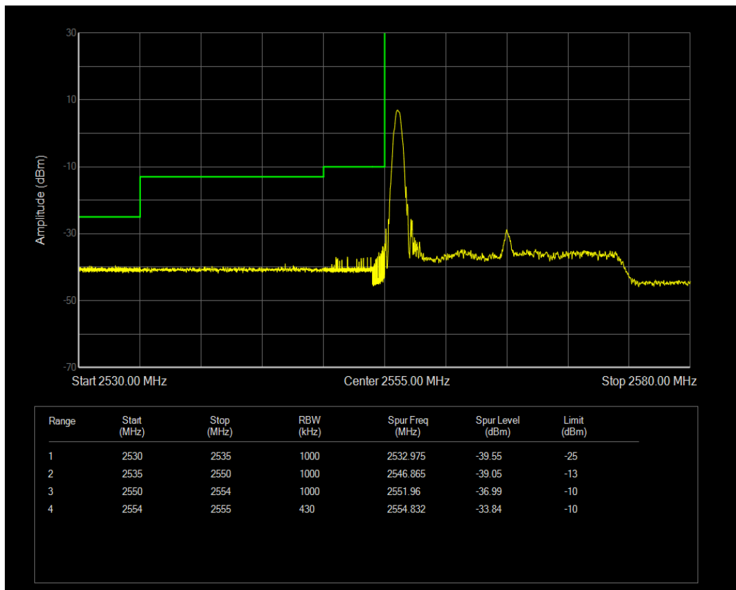
Band41(2555-2655) QPSK BW=20MHz Channel=40340 RB Size=1 Position=#Max
