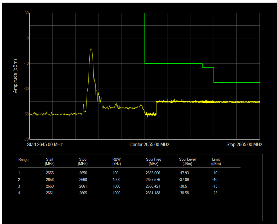
Band41(2555-2655) QAM16 BW=5MHz Channel=41215 RB Size=1 Position=#Max
