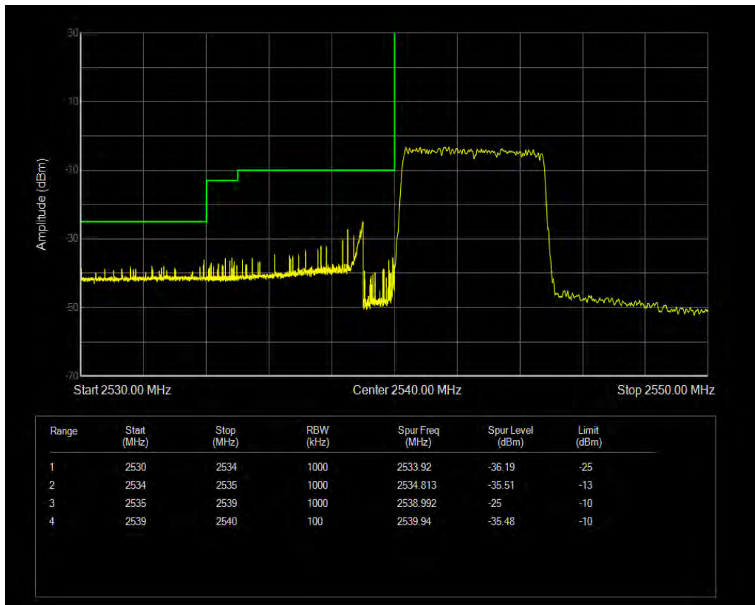
Band41 16QAM BW=5MHz Channel=40115 RB Size=1 Position=#0
