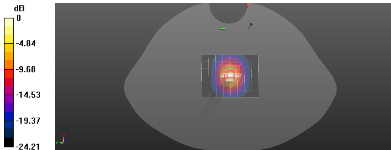
0 dB = 15.1 W/kg = 11.79 dBW/kg
