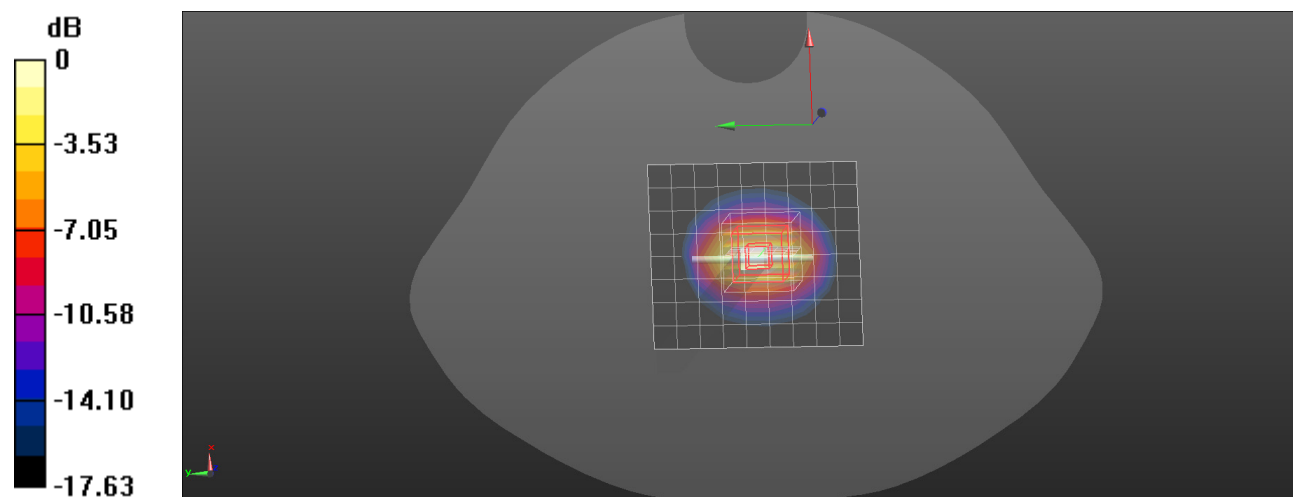
0 dB = 7.54 W/kg = 8.77 dBW/kg
