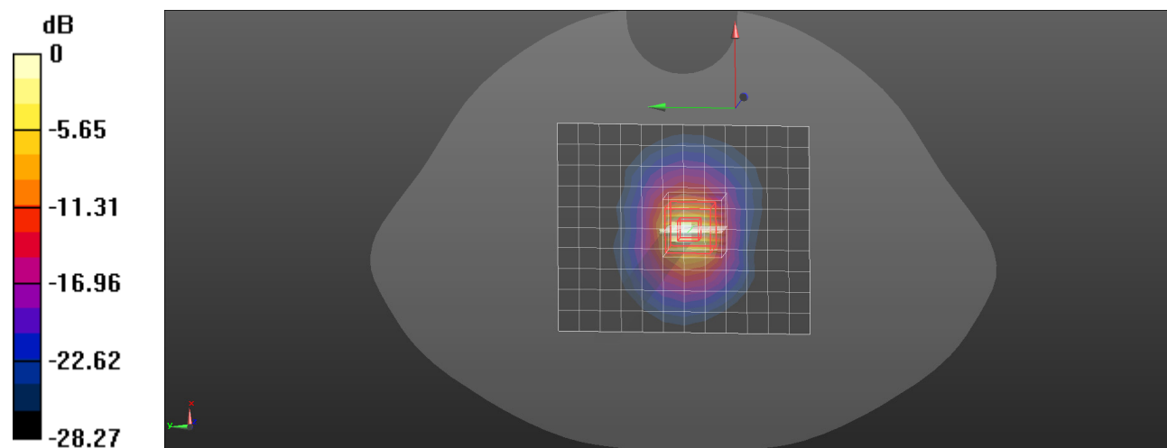
0 dB = 18.8 W/kg = 12.74 dBW/kg
