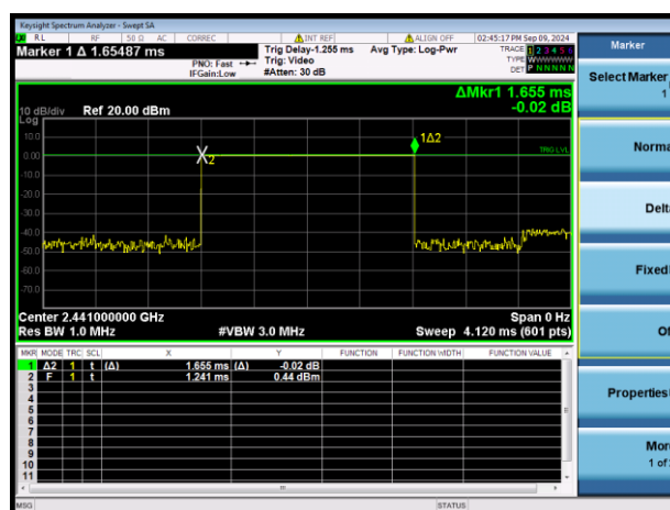
GFSK DH3
