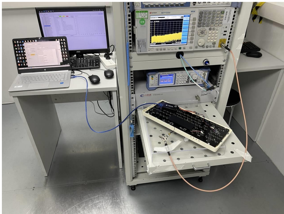
Conducted Test-BLE/2.4G ISM Band
