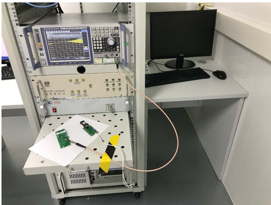
Conducted Test
