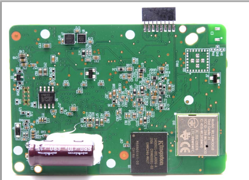
Figure 2: Back side of CCU PCA (WL1831 WiFi/BT Radio – metal box in the lower right corner)
