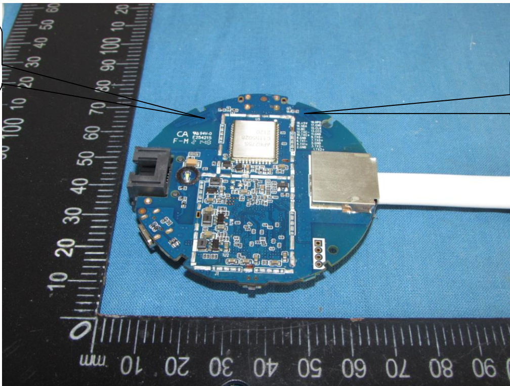
Bluetooth/WiFi Antenna [Antenna 1]
