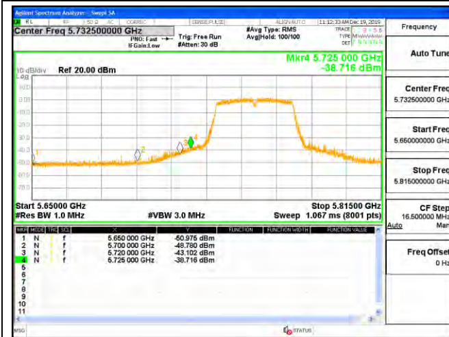
Channel 151 / 5755 MHz – Peak
