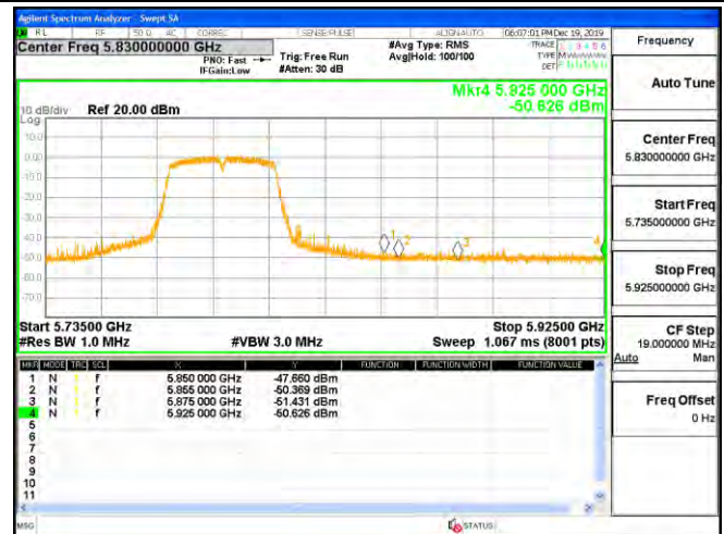
Channel 159 / 5795 MHz – Peak
