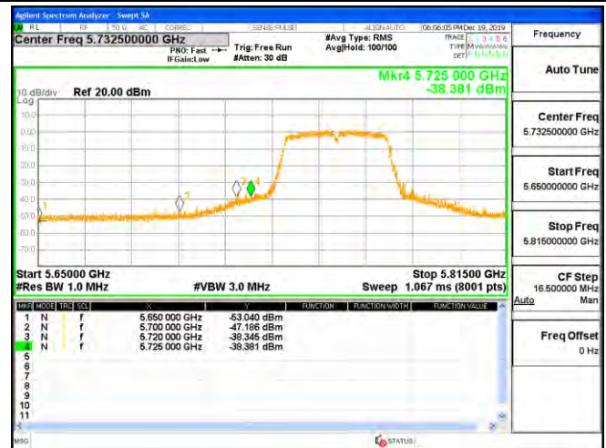
Channel 151 / 5755 MHz – Peak
