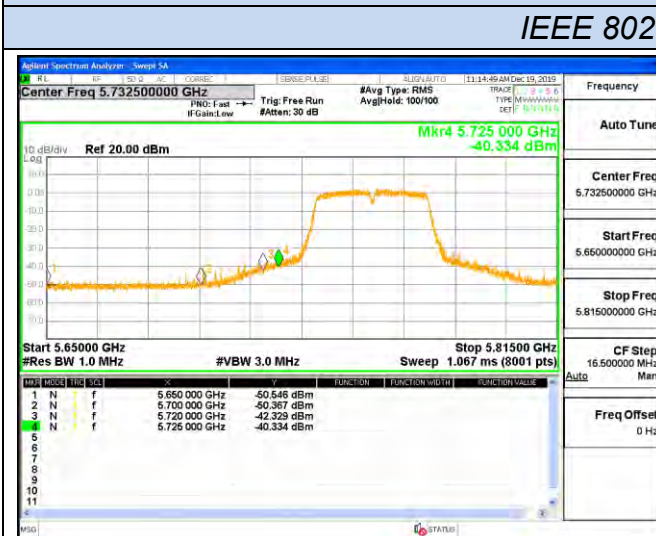
Channel 151 / 5755 MHz – Peak
