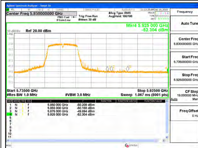
Channel 159 / 5795 MHz – Peak
