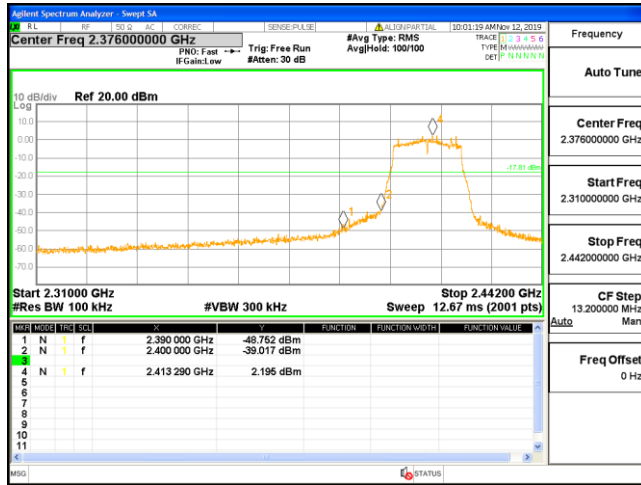
Channel 1 / 2412 MHz
