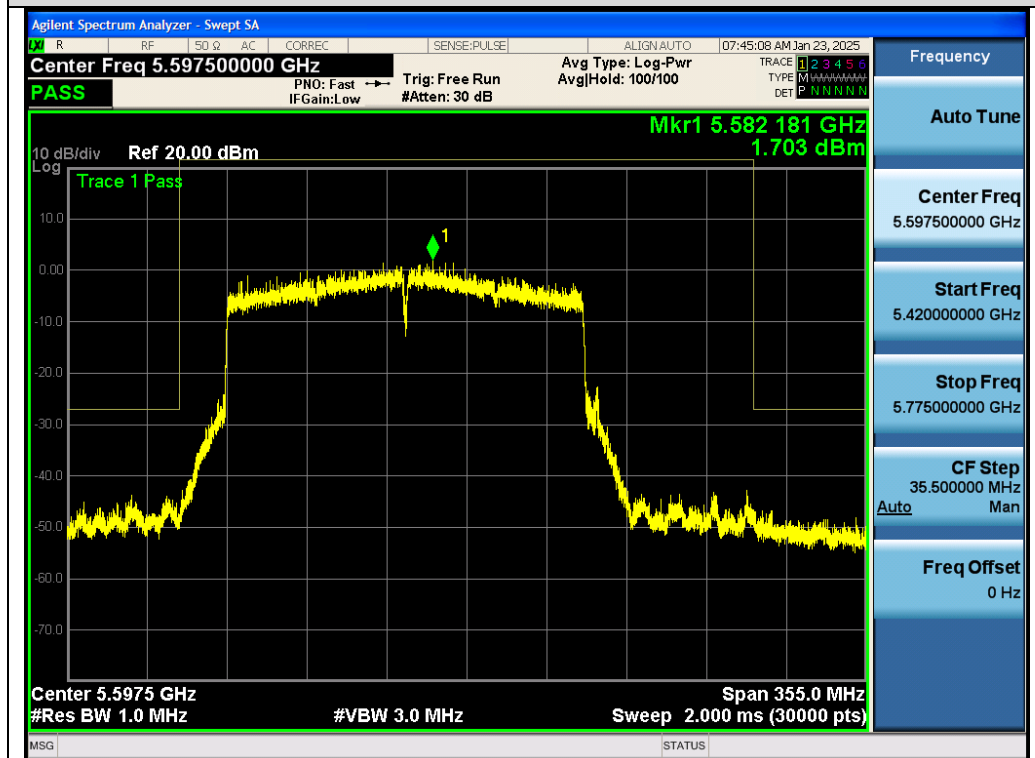
Test_Graph_802.11ax160_Chain B_5570_MCS0_Frequency Band 3
